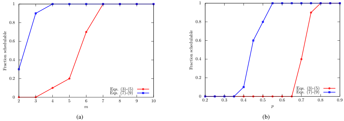
Figure 2. Experimental results II. The diagrams show the percentage of task sets found to be schedulable by Corollary III.4 (Eqs. (3)-(5)) and by Theorem IV.2 (Eqs. (7)-(9) with k=3 ). (a) Variation of m ( \kappa=m , \bar{U}=1 , p=1 , \alpha=0.2 ). (b) Variation of p ( m=10 , \kappa=10 , \bar{U}=1 , \alpha=0.2 ).
