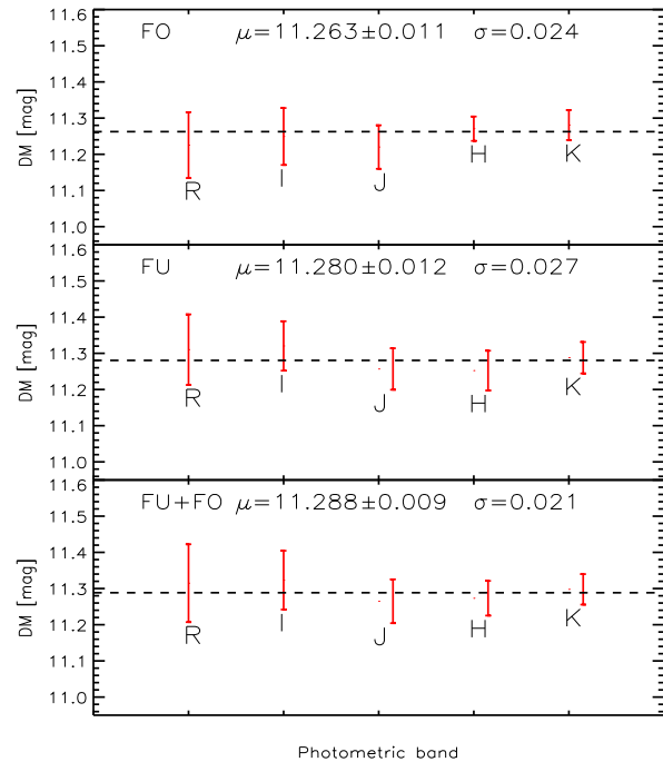
Figure 10. Top: true DM based on optical and NIR predicted FO PL relations that take account of the metallicity dependence. Following Carretta et al. (2009) we adopted for M4 an iron abundance of [\text{Fe}/\text{H}] = -1.10 . The error bars include the photometric error, the extinction error, and the standard deviation of the adopted PL relation. The dashed lines show the weighted mean true DM ( \mu ). The error on the mean and the standard deviations are also labeled. Middle: same as the top, but for optical and NIR predicted FU PL relations. Bottom: same as the top, but for optical and NIR predicted PL relations including FU and FO RR Lyrae models.
