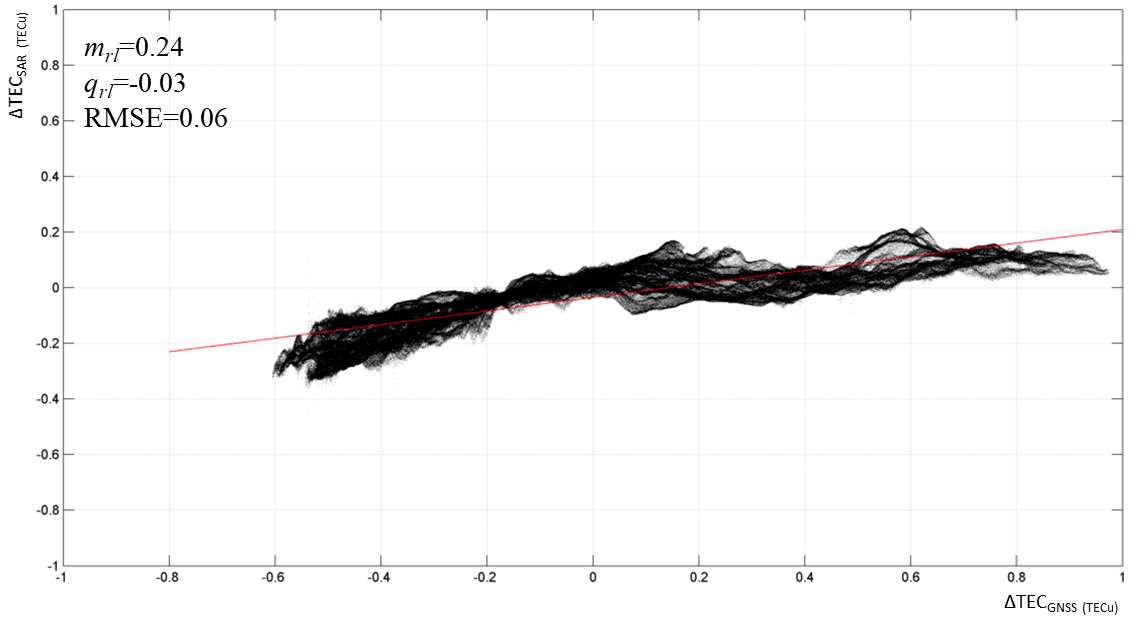
Fig. 6-24 Scatter plot of \Delta TEC_{SAR} vs \Delta TEC_{GNSS} for the third case study (master: 16 August 2007 and slave: 1 October 2007). In red, the regression line is plotted. Its angular coefficient, m_{rl} , and its intercept q_{rl} are also shown together with the RMSE .
