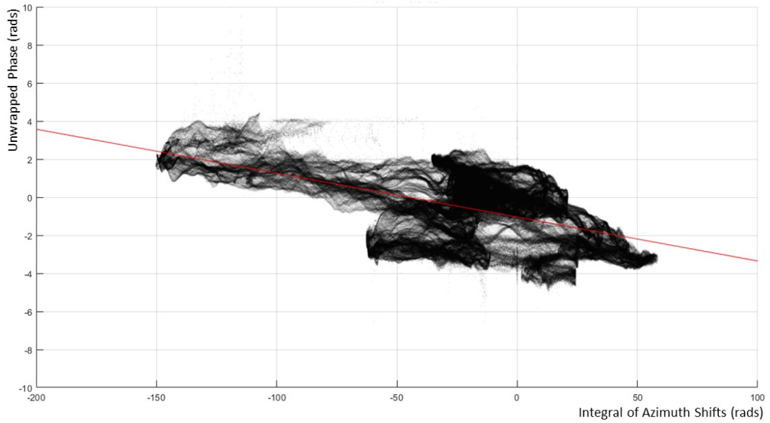
Fig. 6-30 Scatter plot of Integral of azimuth shifts vs unwrapped phase for the fifth case study (master: 24 May 2010 and slave: 9 July 2010). In red, the regression line is plotted.
