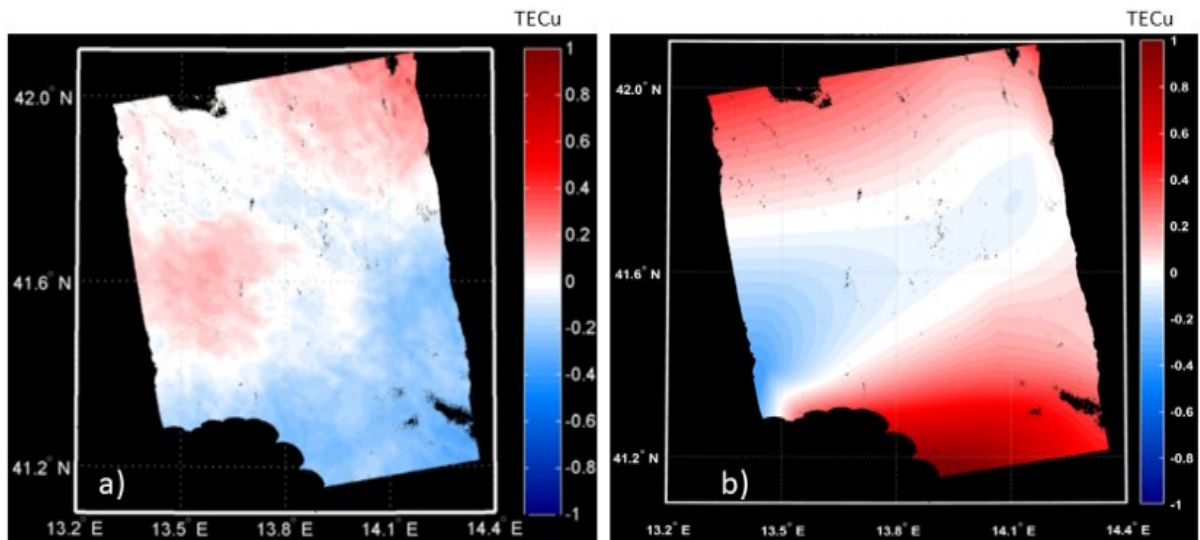
Fig. 6-31 \Delta TEC_{SAR} (a) and \Delta TEC_{GNSS} (b). The colorbars express, in TECu, the TEC variation between 24 May 2010 and 9 July 2010.
