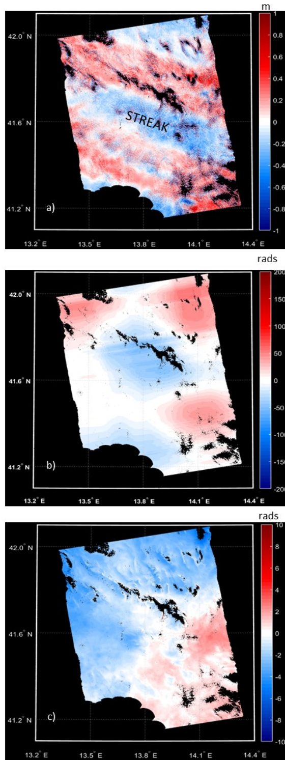
Fig. 6-25 Azimuth shifts a), integral of the azimuth shifts b) and unwrapped phase c) obtained by using as master (8 April 2010) and as slave images (24 May 2010). The shifts are obtained by using MAI technique. Colorbar for the panel a) expresses the displacement in meters. To compare panel b) with panel c), both the integral of the azimuth shifts and the unwrapped phase are expressed in radians.
