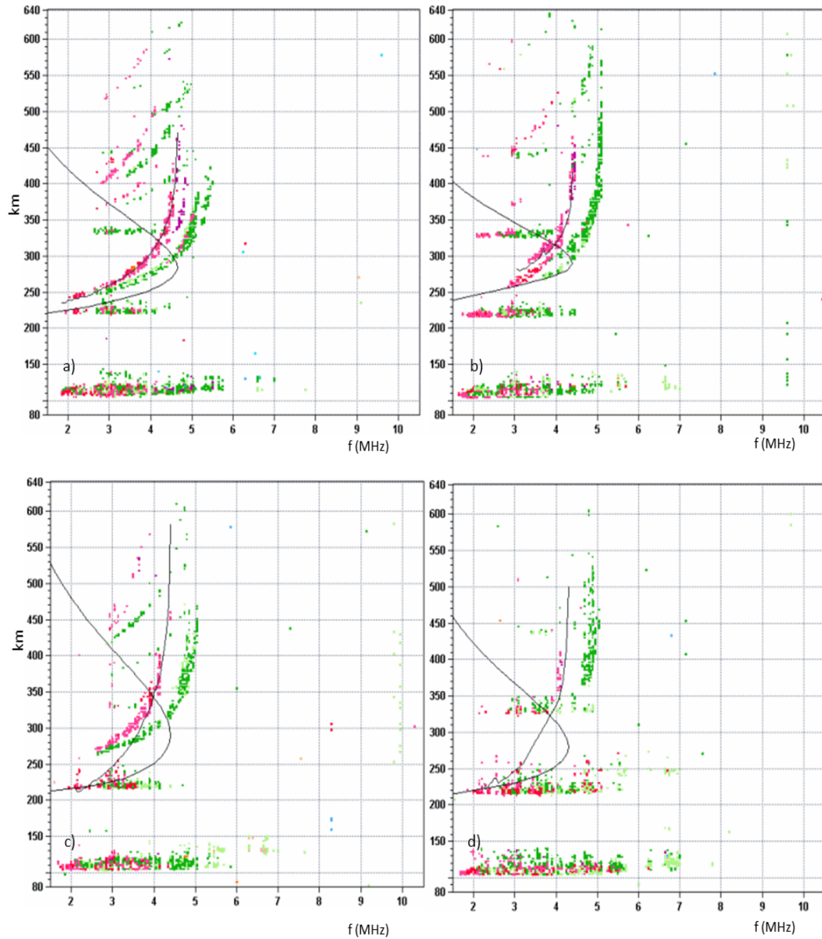
Fig. 6-8 Ionograms of 16 August 2007, obtained by using ionosonde DPS-4 locates in Rome. In a) is shown the ionogram at 21:00 UT, in b) at 21:15 UT, in c) at 21:30 Ut, in d) at 21:45 UT. The time of ALOS passage is around 21:29 UT. The occurrence of Es can be well recognized. The black line represents the modelled vertical electron density profile.
