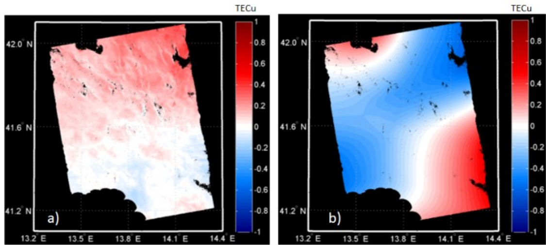
Fig. 6-19 \Delta TEC_{SAR} (a) and \Delta TEC_{GNSS} (b). The colorbars express, in TECu, the TEC variation between 1 July 2007 and 1 October 2007.
