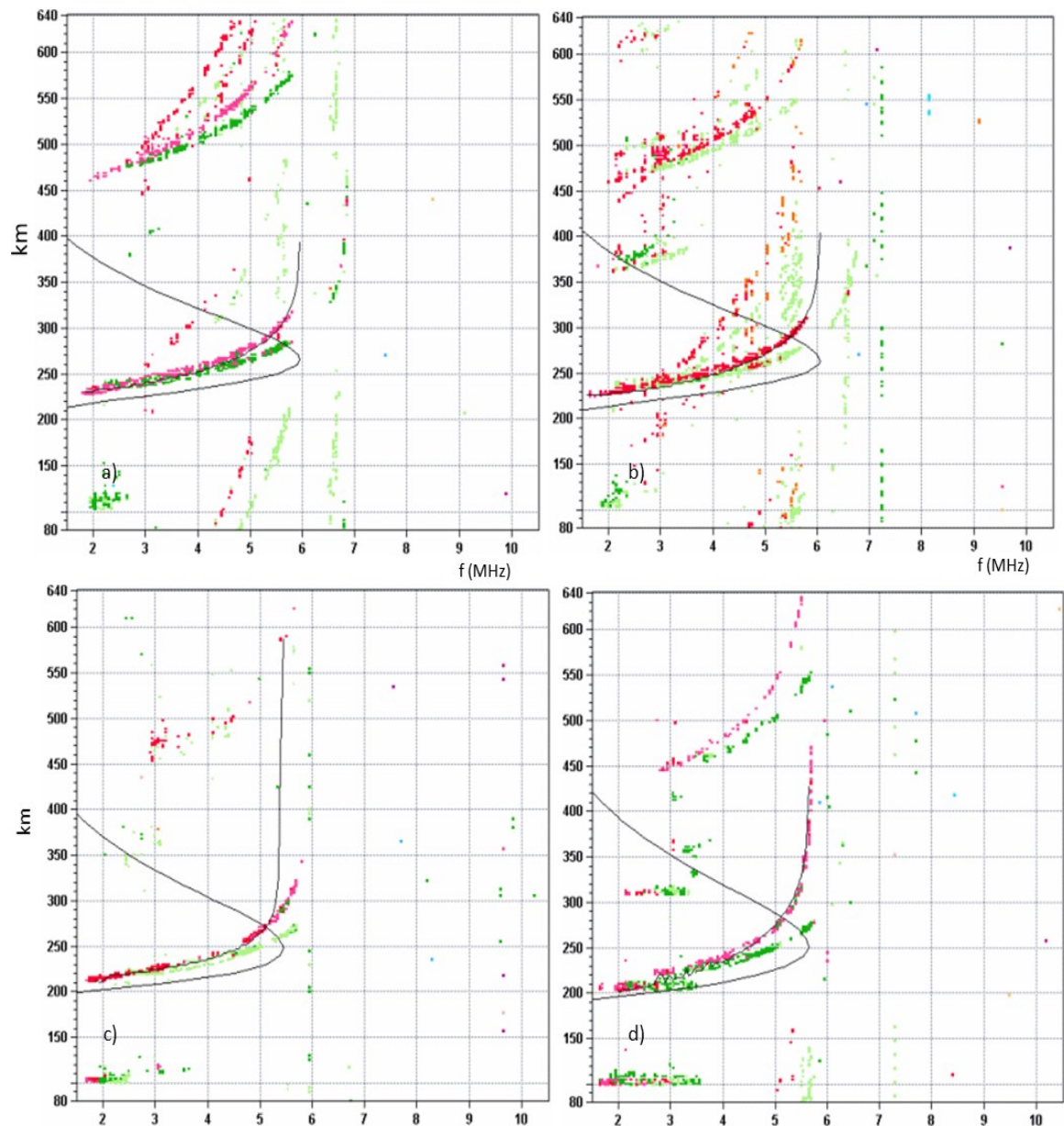
Fig. 6-7 Ionograms of 1 July 2007, obtained by using ionosonde DPS-4 located in Rome. In a) is shown the ionogram at 21:00 UT, in b) at 21:15, in c) at 21:30, in d) at 21:45. The time of ALOS passage is around 21:29. The black line is the modelled vertical electron density profile
