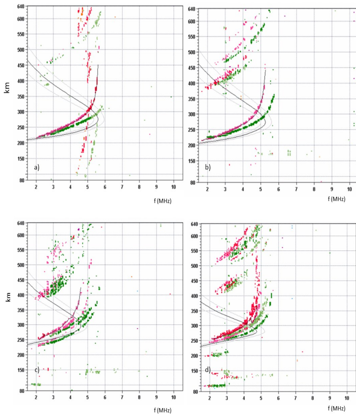
Fig. 6-12 Ionograms of 9 July 2010, obtained by using ionosonde DPS-4 locates in Rome. In a) is shown the ionogram at 21:00 UT, in b) at 21:15 UT, in c) at 21:30 UT, in d) at 21:45 UT. The time of ALOS passage is around 21:29 UT. The black line represents the modelled vertical electron density profile
