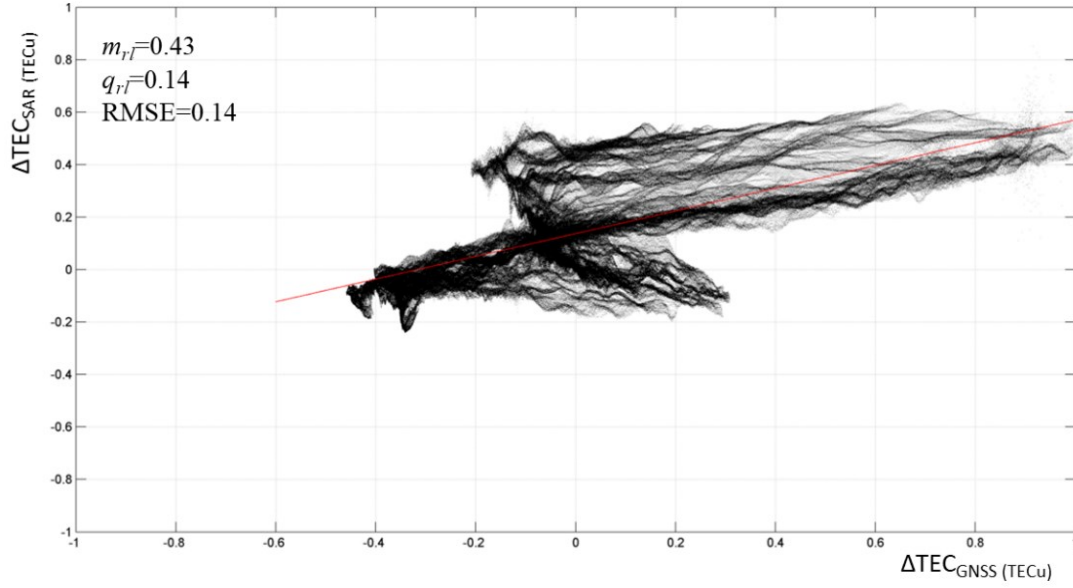
Fig. 6-16 Scatter plot of \Delta TEC_{SAR} vs \Delta TEC_{GNSS} for the first case study (master: 1 July 2007 and slave: 16 August 2007). In red, the regression line is plotted. Its angular coefficient, m_{rl} , and its intercept q_{rl} are also shown together with the RMSE .
