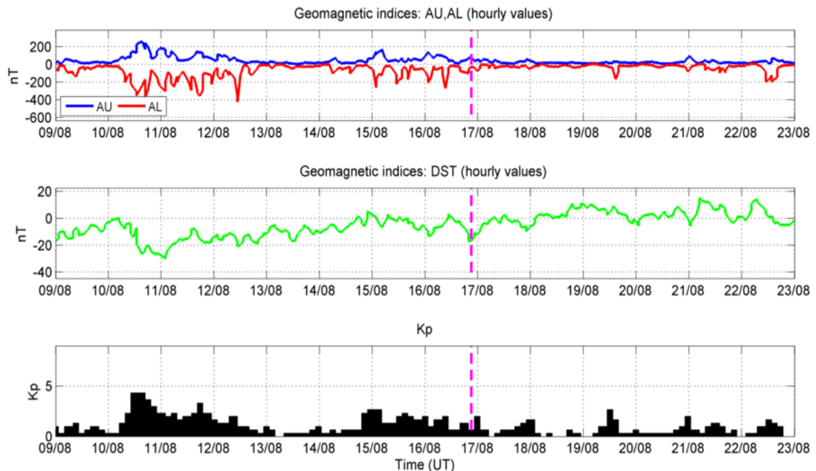
Fig. 6-2 Variation of AU/AL auroral (top), DsT (middle) and Kp (bottom) indices, 15 days around the ALOS passage of 16 August 2007 (World Data Center for Geomagnetism of Kyoto). Purple line identifies the time of the ALOS passage.
