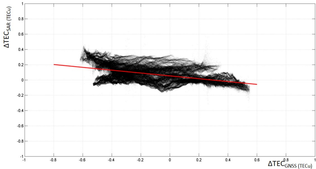
Fig. 6-20 Scatter plot of \Delta TEC_{SAR} vs \Delta TEC_{GNSS} for the second case study (master: 1 July 2007 and slave: 1 October 2007). In red, the regression line is plotted.
