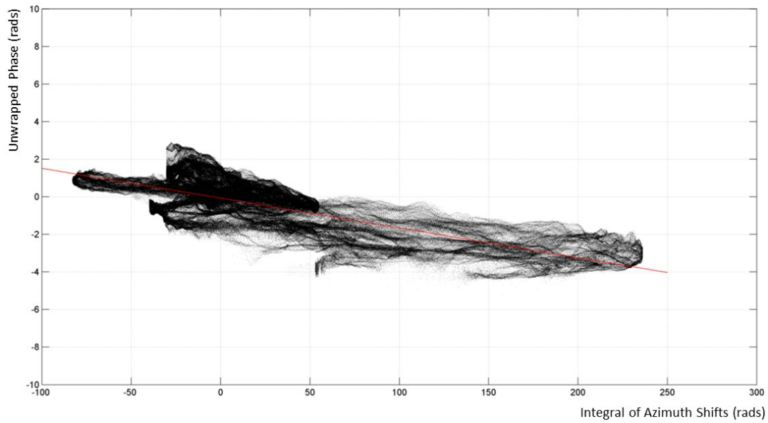
Fig. 6-22 Scatter plot of Integral of azimuth shifts vs unwrapped phase for the third case study (master: 16 August 2007 and slave: 1 October 2007). In red, the regression line is plotted.
