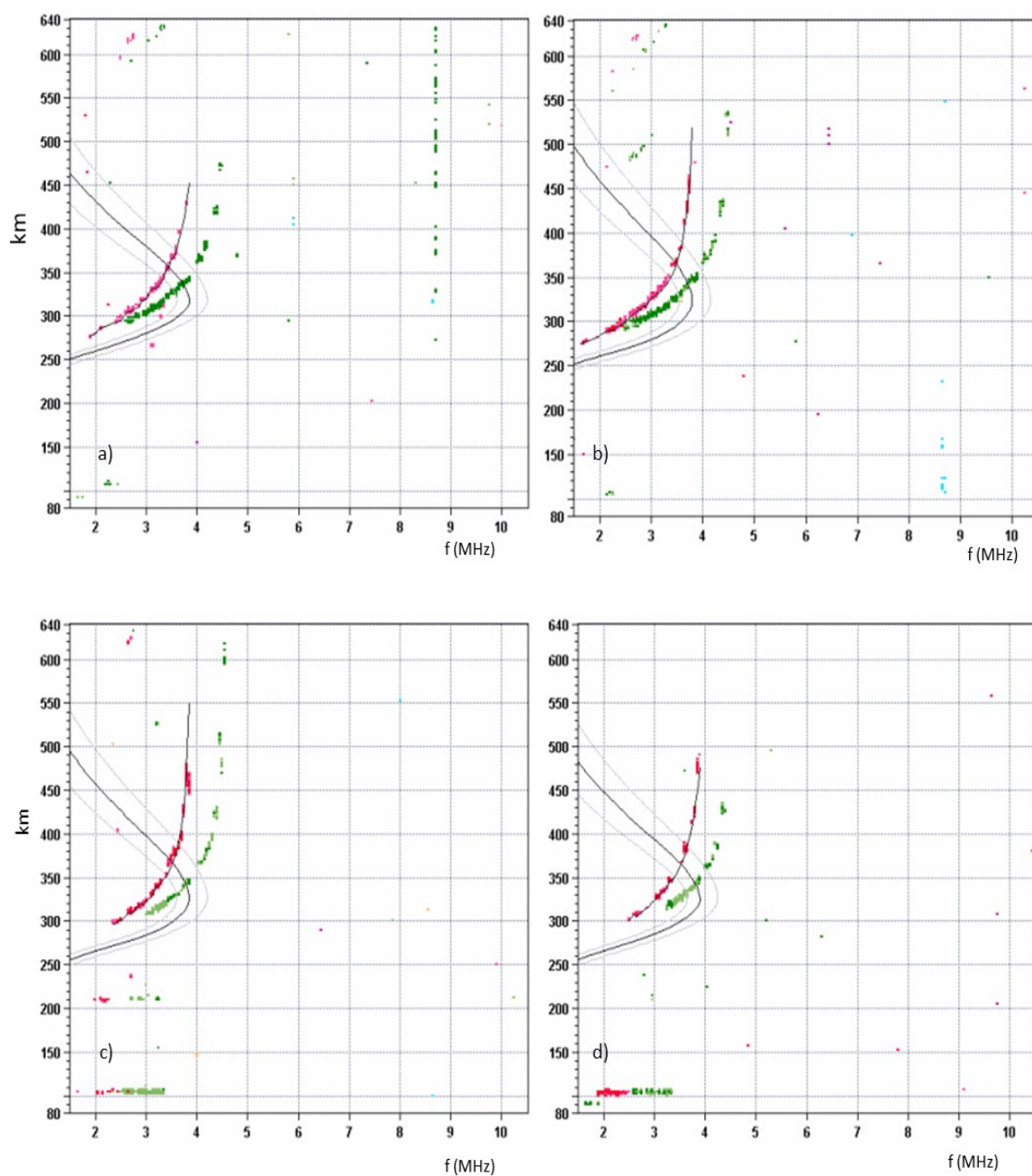
Fig. 6-10 Ionograms of 8 April 2010, obtained by using ionosonde DPS-4 locates in Rome. In a) is shown the ionogram at 21:00 UT, in b) at 21:15 UT, in c) at 21:30 UT, in d) at 21:45 UT. The time of ALOS passage is around 21:29 UT. The black line represents the modelled vertical electron density profile.
