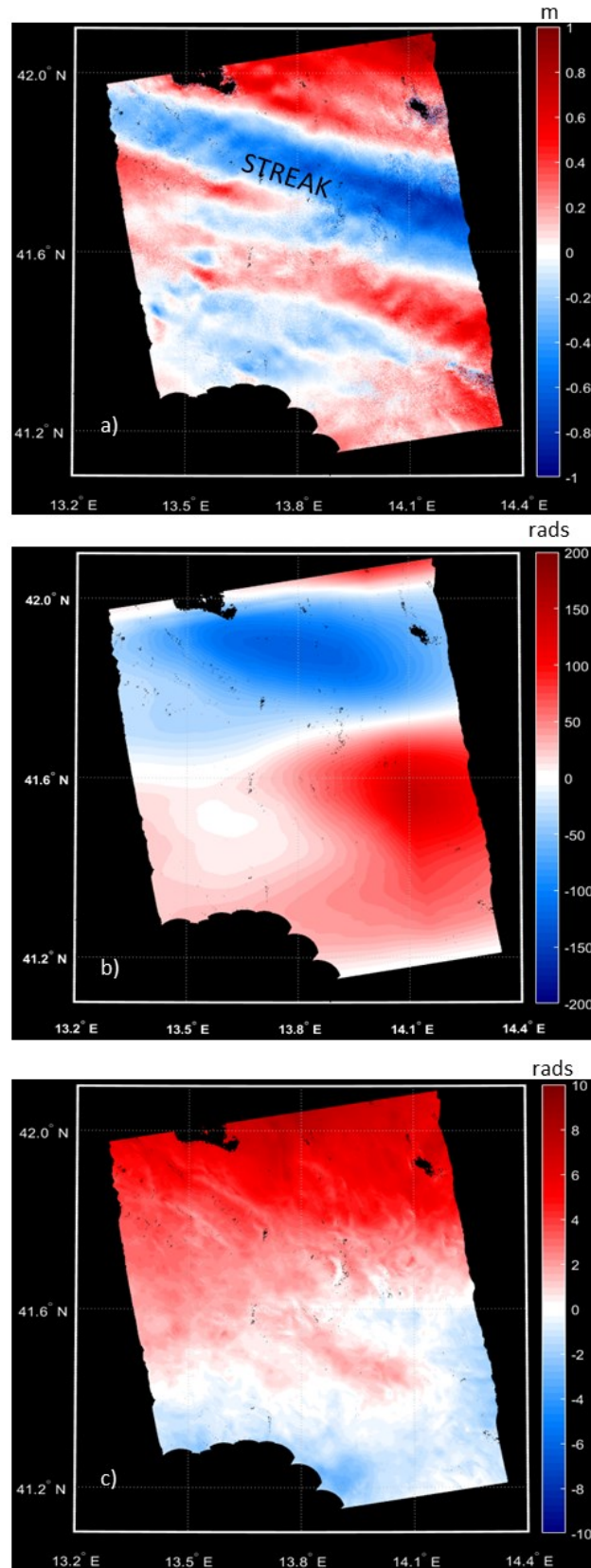
Fig. 6-13 Azimuth shifts a), integral of the azimuth shifts b) and unwrapped phase c) obtained by using as master (1 July 2007) and as slave images (16 August 2007) The shifts are obtained by using MAI technique. Colorbar for the panel a) expresses the displacement in meters. To compare panel b) with panel c), both the integral of the azimuth shifts and the unwrapped phase are expressed in radians.
