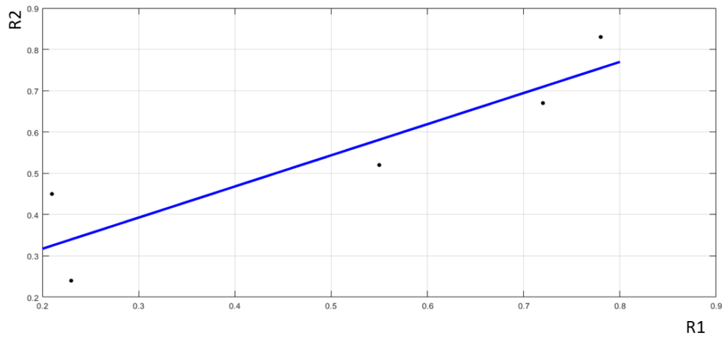
Fig. 6-33 Correlation between integral of azimuth shifts and unwrapped phase vs correlation between \Delta TEC_{SAR} and \Delta TEC_{GNSS} .
