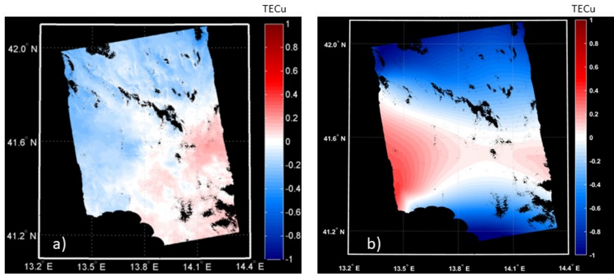
Fig. 6-27 \Delta TEC_{SAR} (a) and \Delta TEC_{GNSS} (b). The colorbars express, in TECu, the TEC variation between 8 April 2010 and 24 May 2010.
