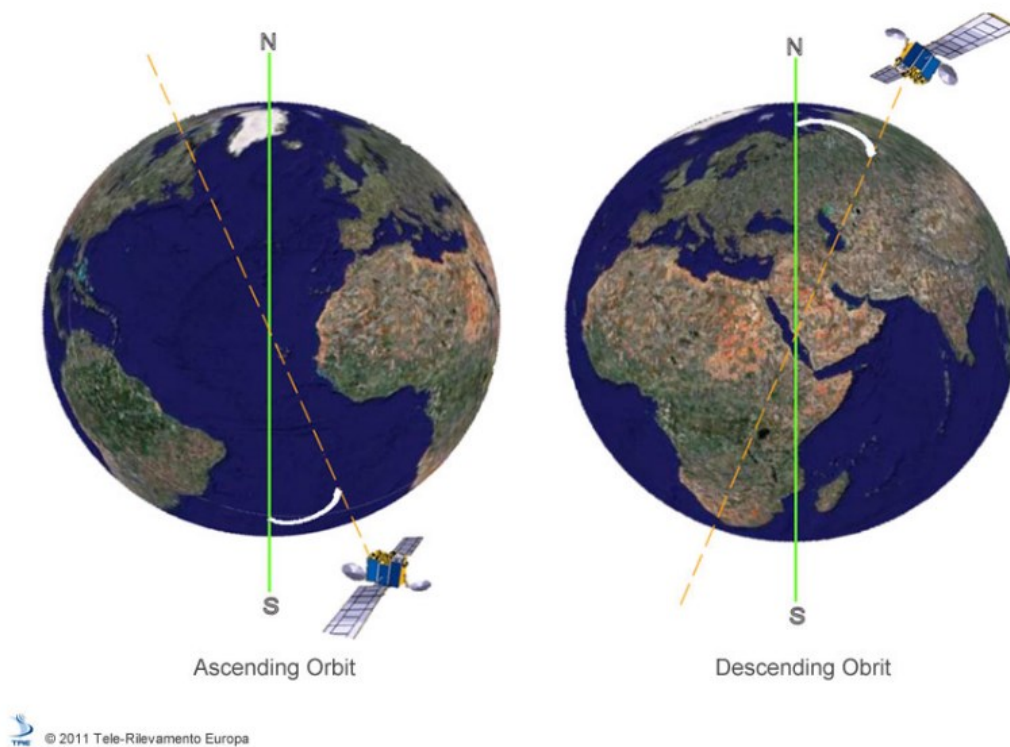
Fig. 3-2 Ascending and descending orbits
