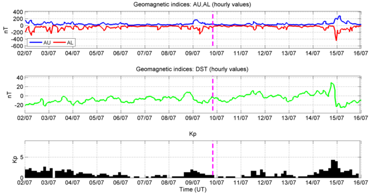
Fig. 6-6 Variation of AU/AL auroral (top), DST (middle) and Kp (bottom) indices, 15 days around the ALOS passage of 9 July 2010 (World Data Center for Geomagnetism of Kyoto). Purple line identifies the time of the ALOS passage.
