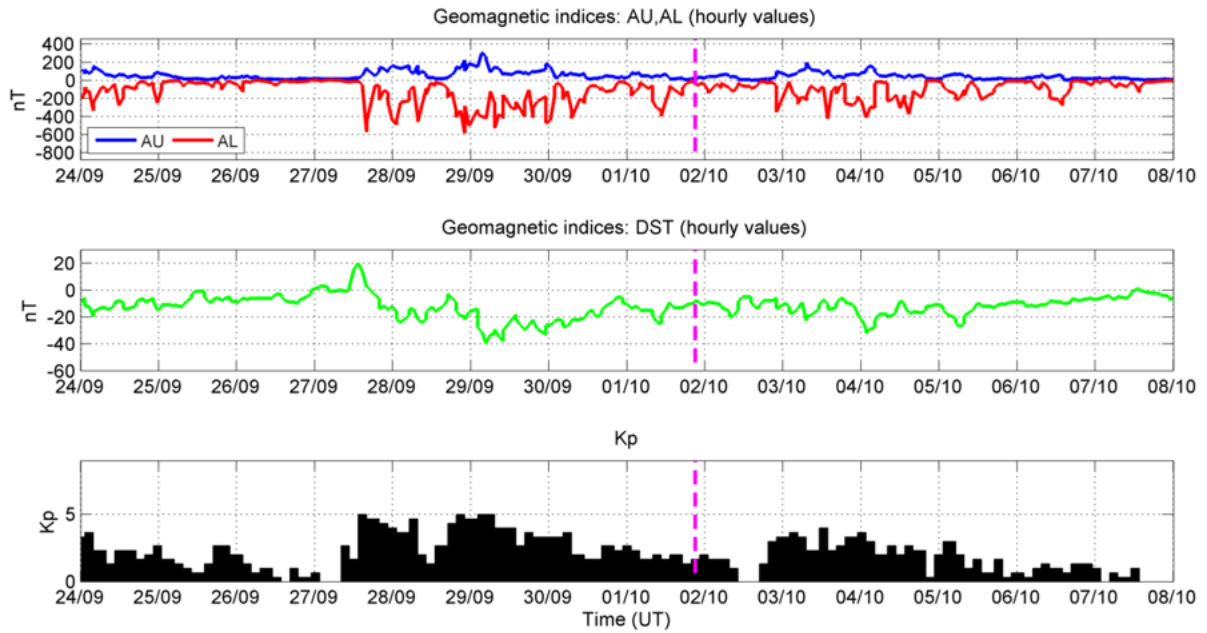
Fig. 6-3 Variation of AU/AL auroral (top), DsT (middle) and Kp (bottom) indices, 15 days around the ALOS passage of 1 October 2007 (World Data Center for Geomagnetism of Kyoto). Purple line identifies the time of the ALOS passage.
