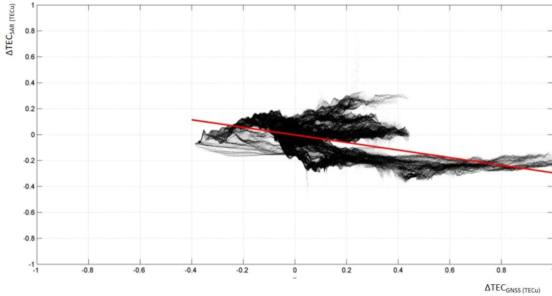
Fig. 6-32 Scatter plot of \Delta TEC_{SAR} vs \Delta TEC_{GNSS} for the fifth case study (master: 24 May 2010 and slave: 9 July 2010). In red, the regression line is plotted.
