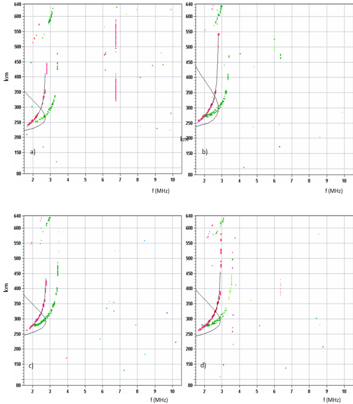
Fig. 6-9 Ionograms of 1 October 2007, obtained by using ionosonde DPS-4 located in Rome. In a) is shown the ionogram at 21:00 UT, in b) at 21:15 UT, in c) at 21:30 UT, in d) at 21:45 UT. The time of ALOS passage is around 21:29 UT. The black line is the modelled vertical electron density profile.
