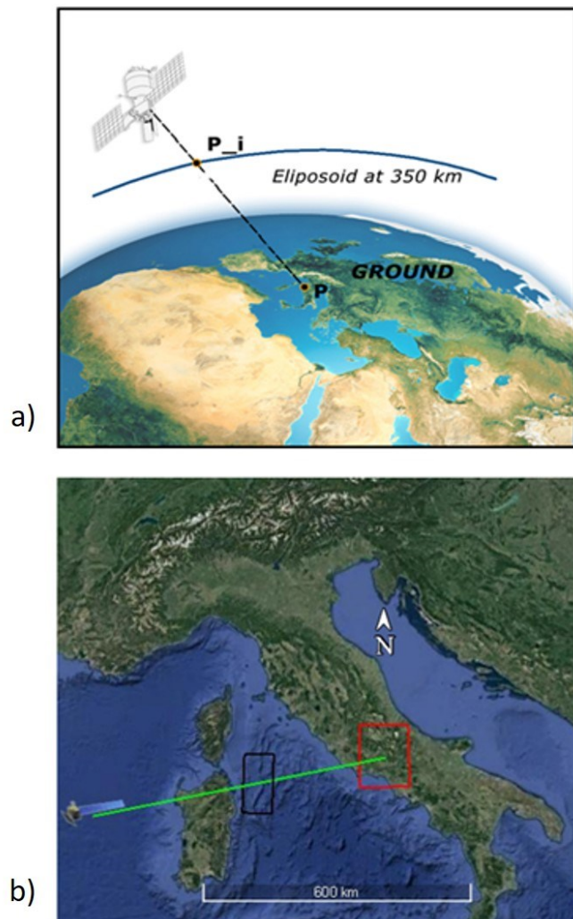
Fig. 5-3 Ionosphere crossed by SAR signal. Panel a sketches how to found the intersection P_i between the SAR signal and the ellipsoid project at 350 km (altitude of the thin ionospheric shell) given a point P at ground level Panel b shows the portion of the ionosphere (black rectangle) at 350 km crossed by ALOS-PALSAR signals and the corresponding image area at ground (red rectangle).
