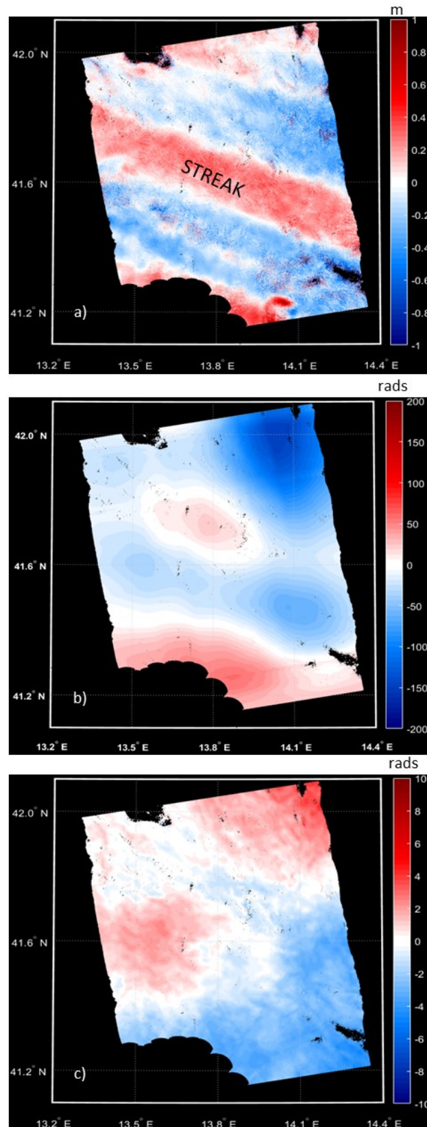
Fig. 6-29 Azimuth shifts a), integral of the azimuth shifts b) and unwrapped phase c) obtained by using as master (24 May 2010) and as slave images (9 July 2010). The shifts are obtained by using MAI technique. Colorbar for the panel a) expresses the displacement in meters. To compare panel b) with panel c), both the integral of the azimuth shifts and the unwrapped phase are expressed in radians.
