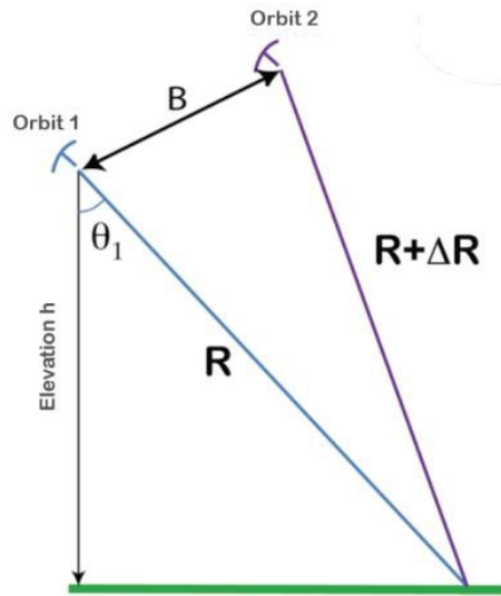
Fig. 3-3 Repeat-pass interferometry mode R is the satellite-target distance for the first orbit, R + \Delta R is the satellite-target distance for the second orbit, \theta_1 is the look angle for the first satellite and B is the baseline
