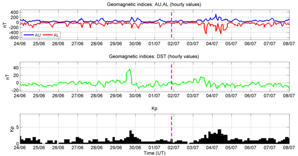
Fig. 6-1 Variation of AU/AL auroral (top), DsT (middle) and Kp (bottom) indices, 15 days around the ALOS passage on 1 July 2007 (World Data Center for Geomagnetism of Kyoto). Purple line identifies the time of the ALOS passage.
