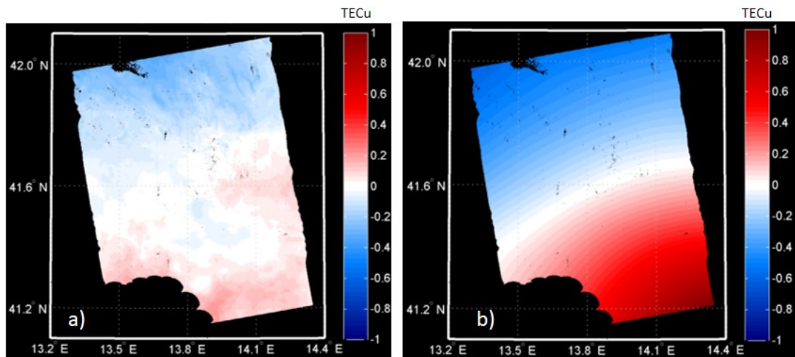
Fig. 6-23 \Delta TEC_{SAR} (a) and \Delta TEC_{GNSS} (b). The colorbars express, in TECu, the TEC variation between 16 August 2007 and 1 October 2007.
