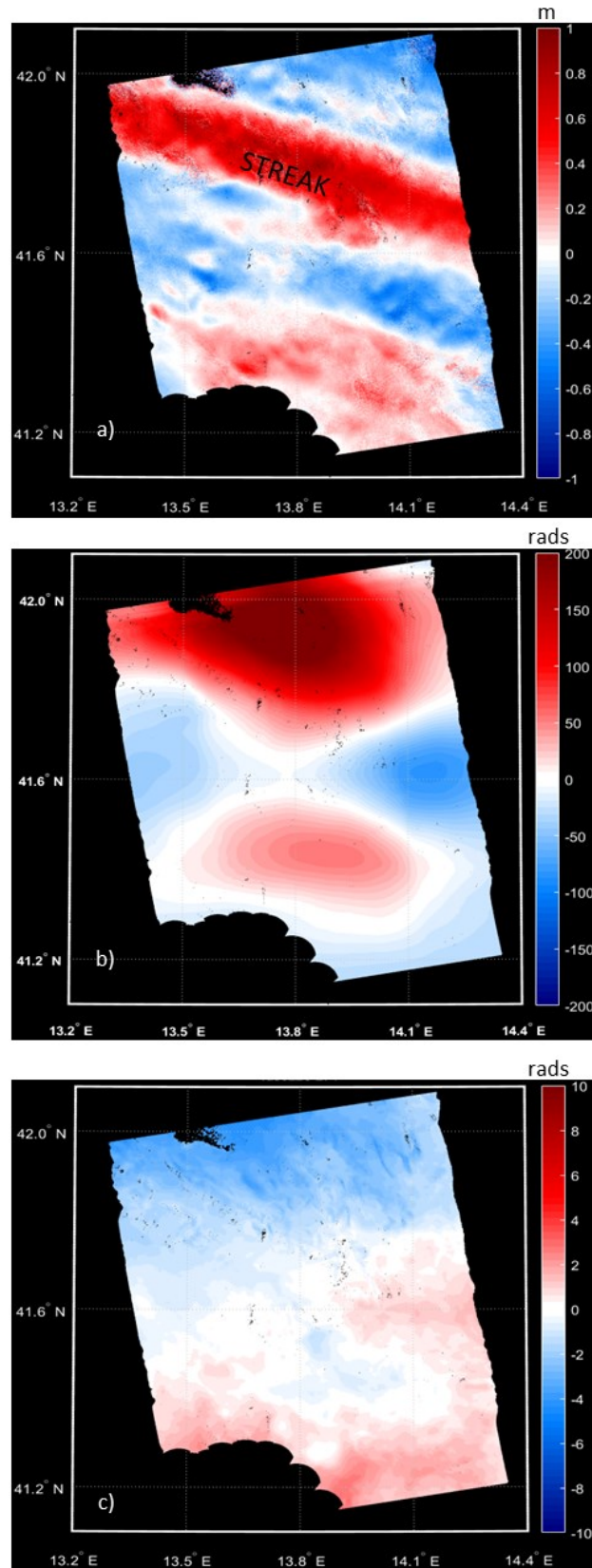
Fig. 6-21 Azimuth shifts a), integral of the azimuth shifts b) and unwrapped phase c) obtained by using as master (16 August 2007) and as slave images (1 October 2007). The shifts are obtained by using MAI technique. Colorbar for the panel a) expresses the displacement in meters. To compare panel b) with panel c), both the integral of the azimuth shifts and the unwrapped phase are expressed in radians.
