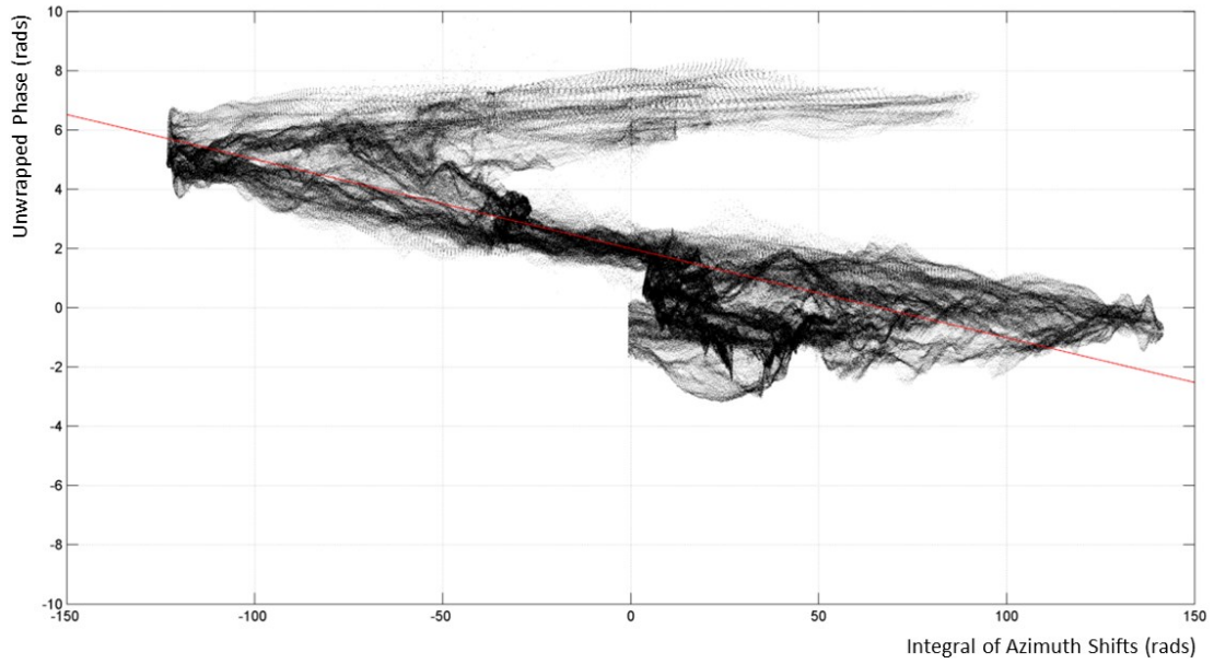
Fig. 6-14 Scatter plot of Integral of azimuth shifts vs unwrapped phase for the first case study (master: 1 July 2007 and slave: 16 August 2007). In red, the regression line is plotted.
