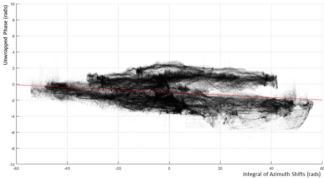
Fig. 6-26 Scatter plot of Integral of azimuth shifts vs unwrapped phase for the fourth case study (master: 8 April 2010 and slave: 24 May 2010). In red, the regression line is plotted.
