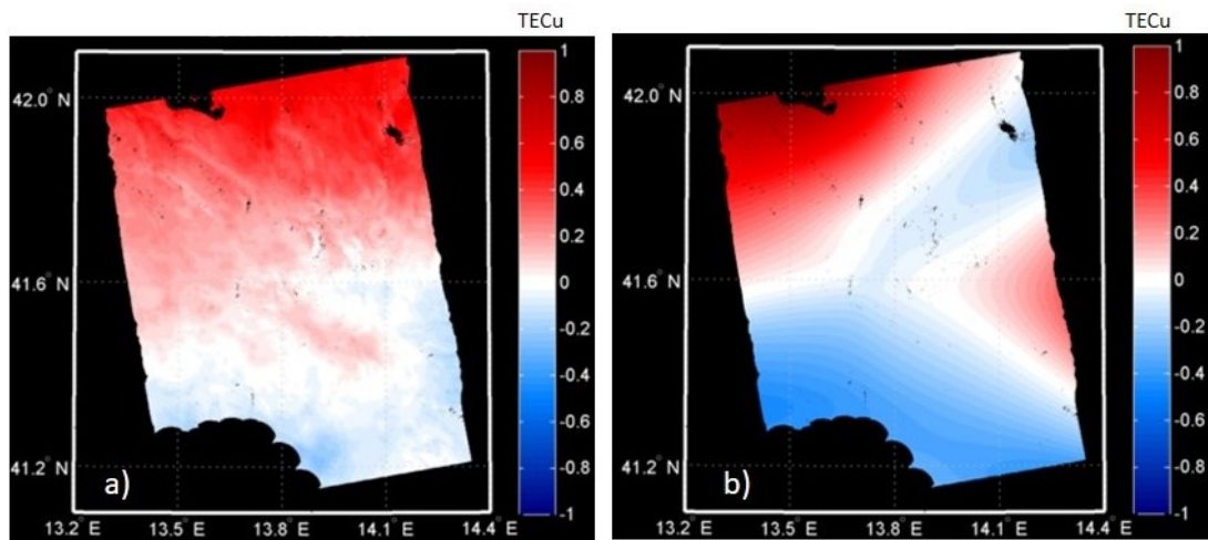
Fig. 6-15 \Delta TEC_{SAR} (a) and \Delta TEC_{GNSS} (b). The colorbars express, in TECu, the TEC variation between 1 July 2007 and 16 August 2007.
