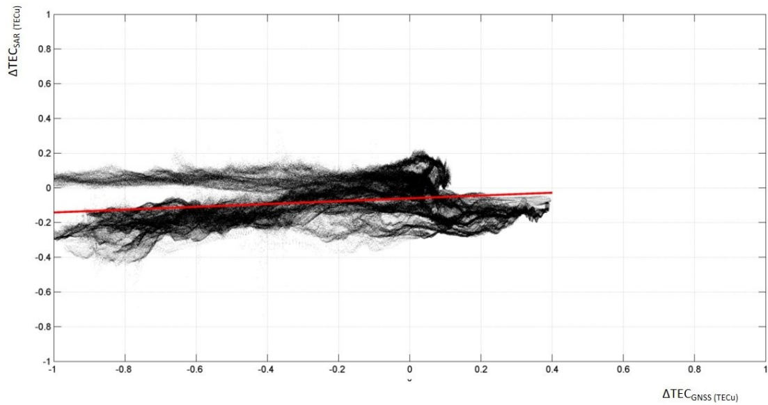
Fig. 6-28 Scatter plot of \Delta TEC_{SAR} vs \Delta TEC_{GNSS} for the fourth case study (master: 8 April 2010 and slave: 24 May 2010). In red, the regression line is plotted.
