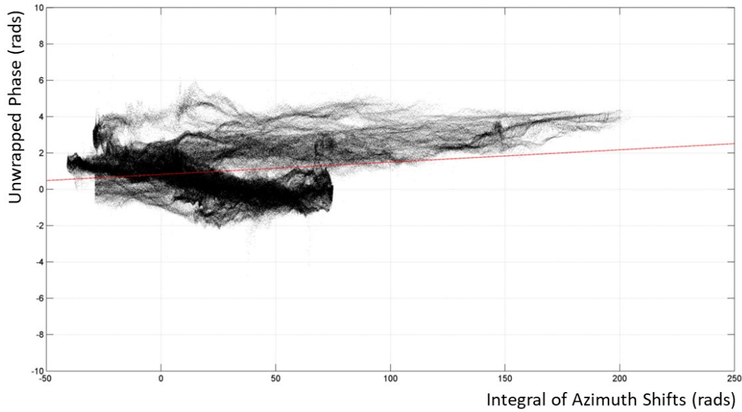
Fig. 6-18 Scatter plot of Integral of azimuth shifts vs unwrapped phase for the second case study (master: 1 July 2007 and slave: 1 October 2007). In red, the regression line is plotted.
