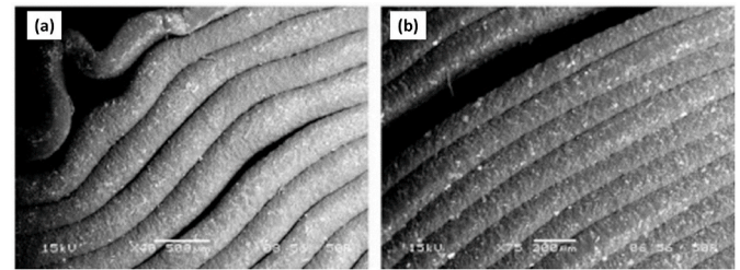
Fig. 13. SEM image of compression failed ABS composite (a) failure due to buckling and (b) de-bonding between layers, reproduced under the terms of the Creative Commons Attribution (CC-BY) license from Ref. [157].
