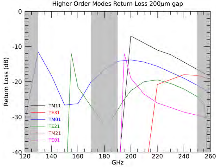
Figure 21. Simulation of the return loss induced by the 200\mu\text{m} gap where the shutter enter to short circuit the waveguide.
