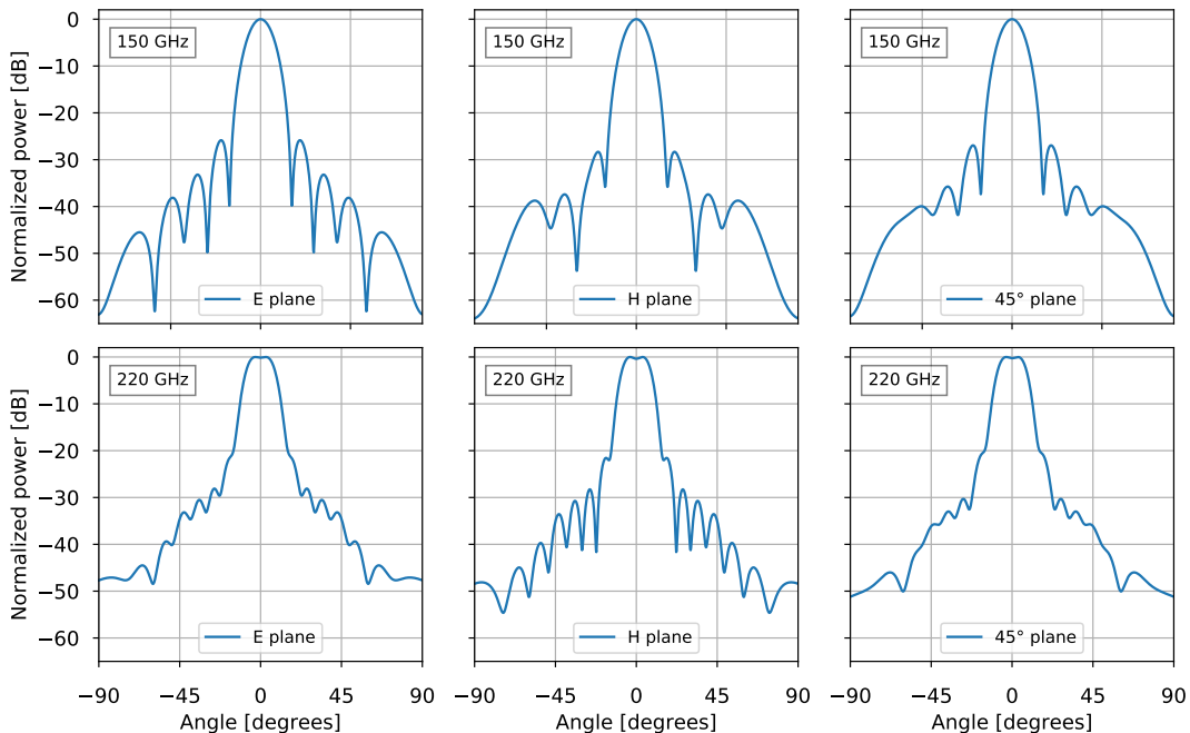
Figure 5. Co-polar simulated beam patterns (E, H, and 45° planes) at 150 GHz (top row) and 220 GHz (bottom row).
