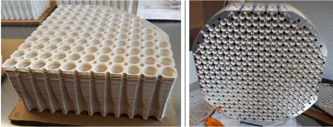
Figure 19. The back-to-back feed-horn system of the QUBIC FI. Left: stacked platelets of a quarter array. Right: one of the two 400 horn arrays.
