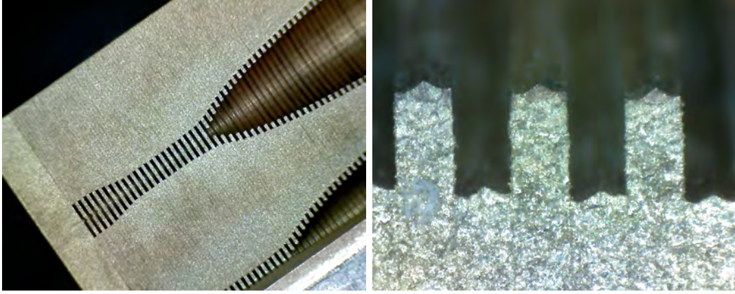
Figure 7. Left. A section of the first feed-horn prototype. Right. Detail of the cusps on teeth and grooves resulting from non uniform chemical erosion.
