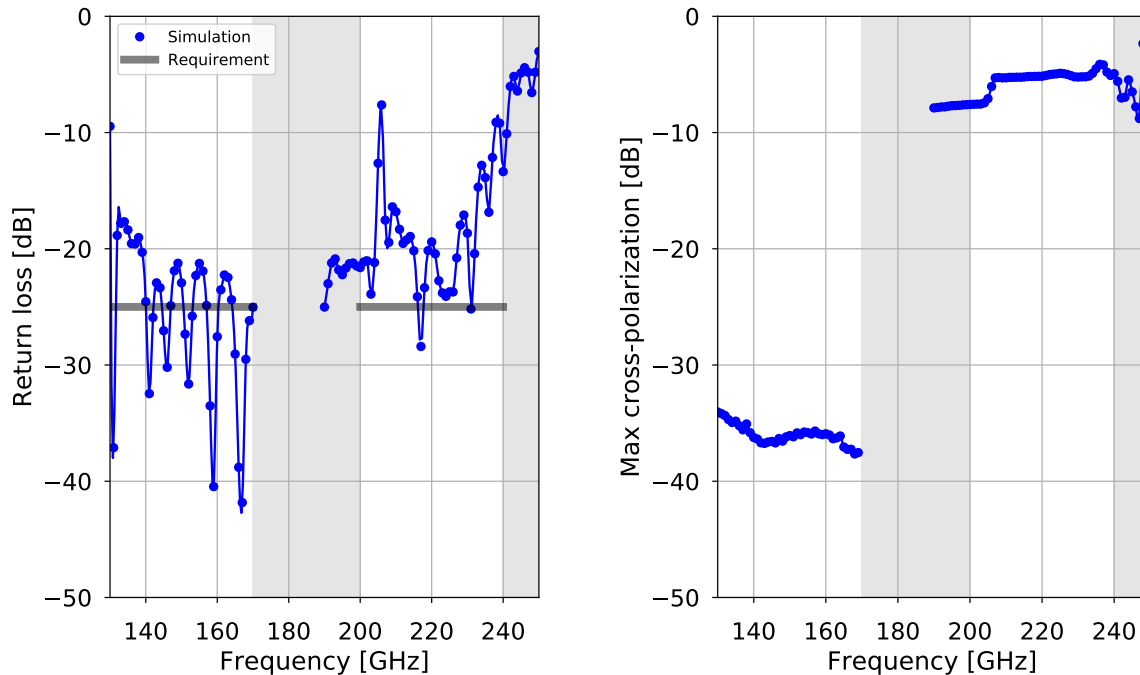
Figure 4. Simulated return loss (left) and maximum cross-polarization (right) in the two QUBIC frequency bands.
