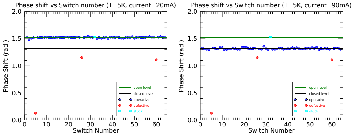
Figure 30. Phase between voltage and current measured by XOR algorithm. Left: shutters in open position Right: shutters in closed position. Switch n.1 was operative at 5K. N. 5, 26 and 60 were defective and n. 32 was stuck open.
