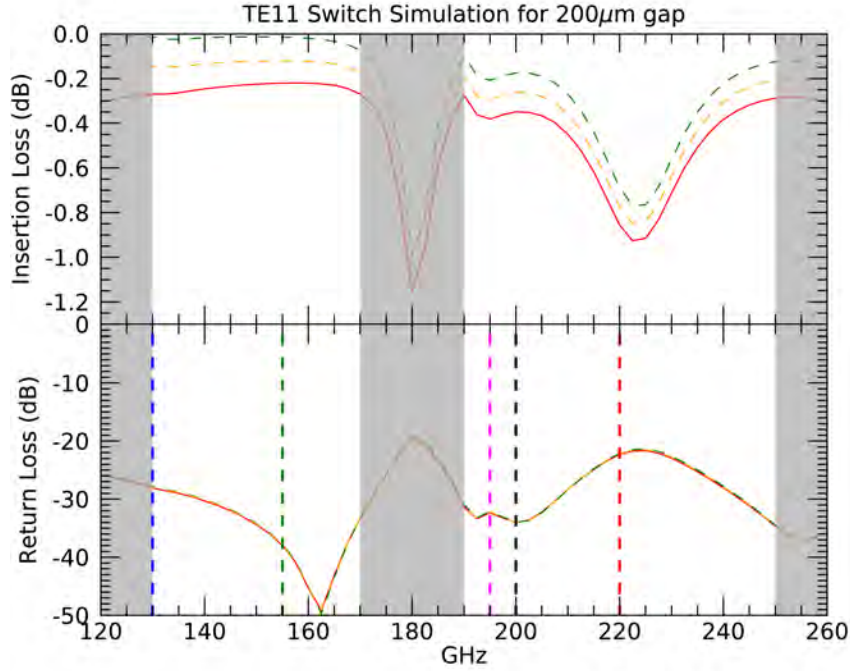
Figure 20. Top: simulation of TE11 mode insertion loss of the switch waveguide for a choke gap of 200\ \mu\text{m} . The red solid line is for an effective resistivity \rho = 16\ \mu\Omega\ \text{cm} , the green dashed line is for a perfect conductor ( \rho = 10^{-6}\ \mu\Omega\ \text{cm} for computational reasons) and the orange dashed line is for Al-6061 resistivity at room temperature ( \rho = 4.19\ \mu\Omega\ \text{cm} ). Bottom: simulation of TE11 mode return loss of the switch waveguide for a choke gap of 200\ \mu\text{m} . Since the return loss is dominated by the switch geometry, the cases for the three resistivities ( \rho = [0, 4.19, 16]\ \mu\Omega\ \text{cm} ) are practically identical. The dashed vertical lines are placed where the higher order modes start to propagate. We used the same color code as in figure 21.
