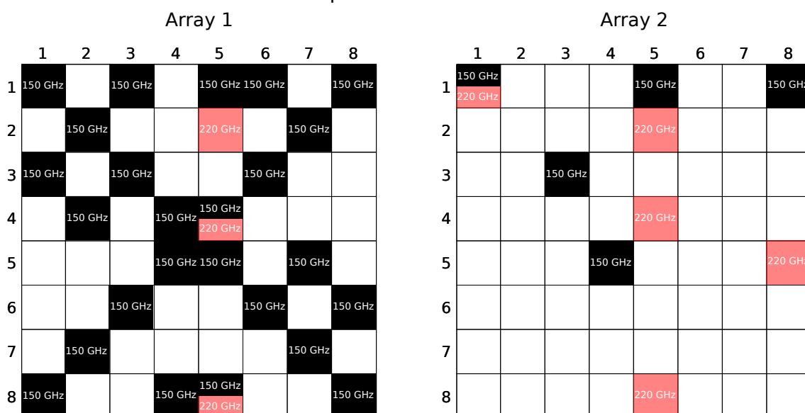
Figure 13. Grids summarizing the electromagnetic measurements carried out on the TD feed-horn arrays. See text for further details.
