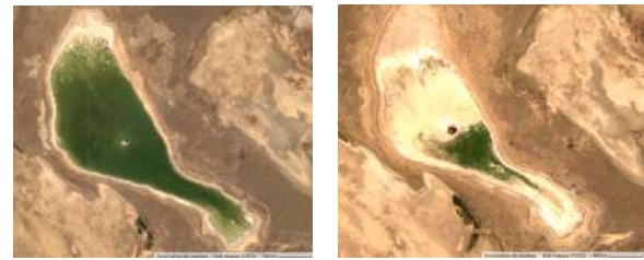
Figure 10. Sentinel-2 median image of Sawa lake on January-March 2020 (left) and on January-March 2022 (right).
