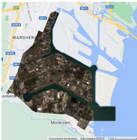
Figure 1. Sentinel-2 multispectral median image (Marghera dock, January-March 2019).
