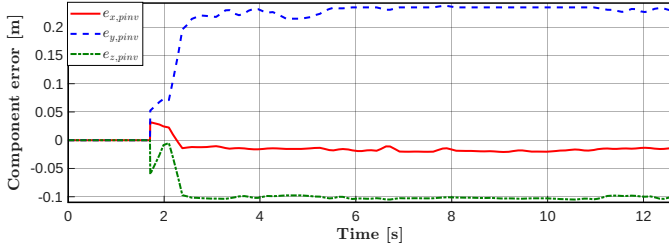
Fig. 7. Components of the position error when estimating the contact point \mathbf{p}_c = (-0.032, -0.052, 0.061) [m] at link 3 using only the residual method with pseudoinversion. The y and z components are both clearly off.
