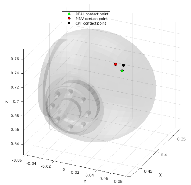
Fig. 4. Visualization of actual contact point (●) at link 6 and its estimate using only the residual method with pseudoinversion (●) or also the contact particle filter (●).
