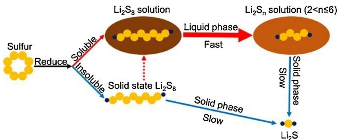
Figure 3. A schematic illustration of the differences in the reaction pathway in unsaturated and saturated LiPSs organic electrolytes. Reproduced with permission from Ref. [52]. Copyright (2017) Published by Elsevier Ltd.
