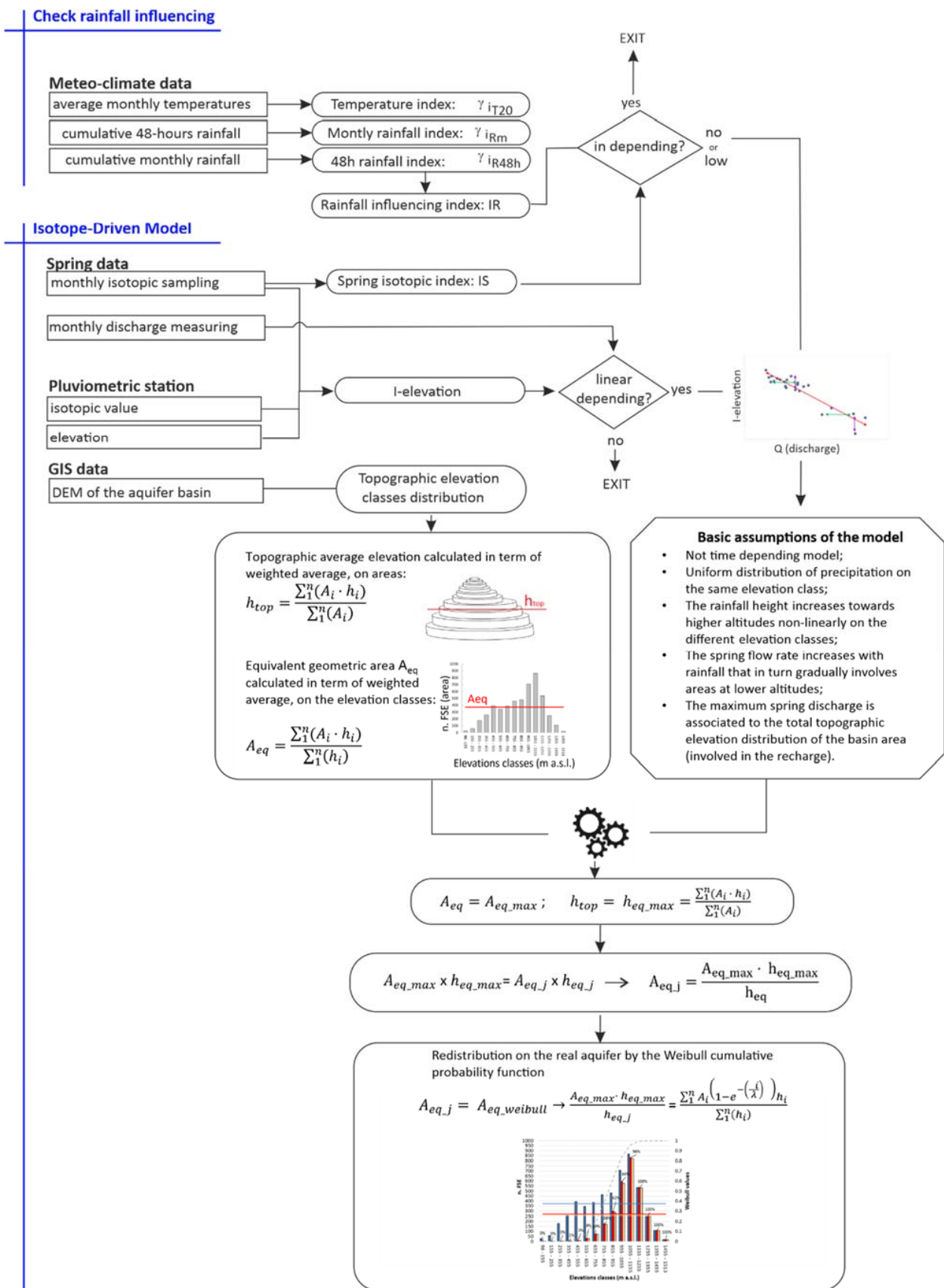
Figure 7. Flowchart of the proposed procedure for the recharge area estimation.
