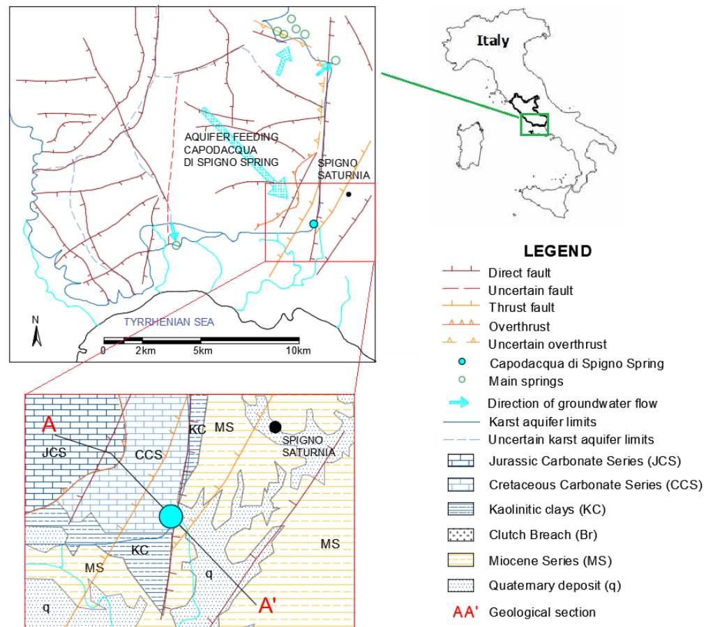
Figure 1. Structural map and main groundwater flow direction of Capodacqua di Spigno Spring ( up ); excerpt of the geological map and positioning of the geological section AA' represented in Figure 3 ( down )—based on Baldi et al., 2005 [28].
