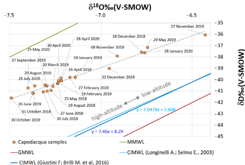
Figure 8. Plot of \delta^2D vs. \delta^{18}O for Capodacqua di Spigno samples.
