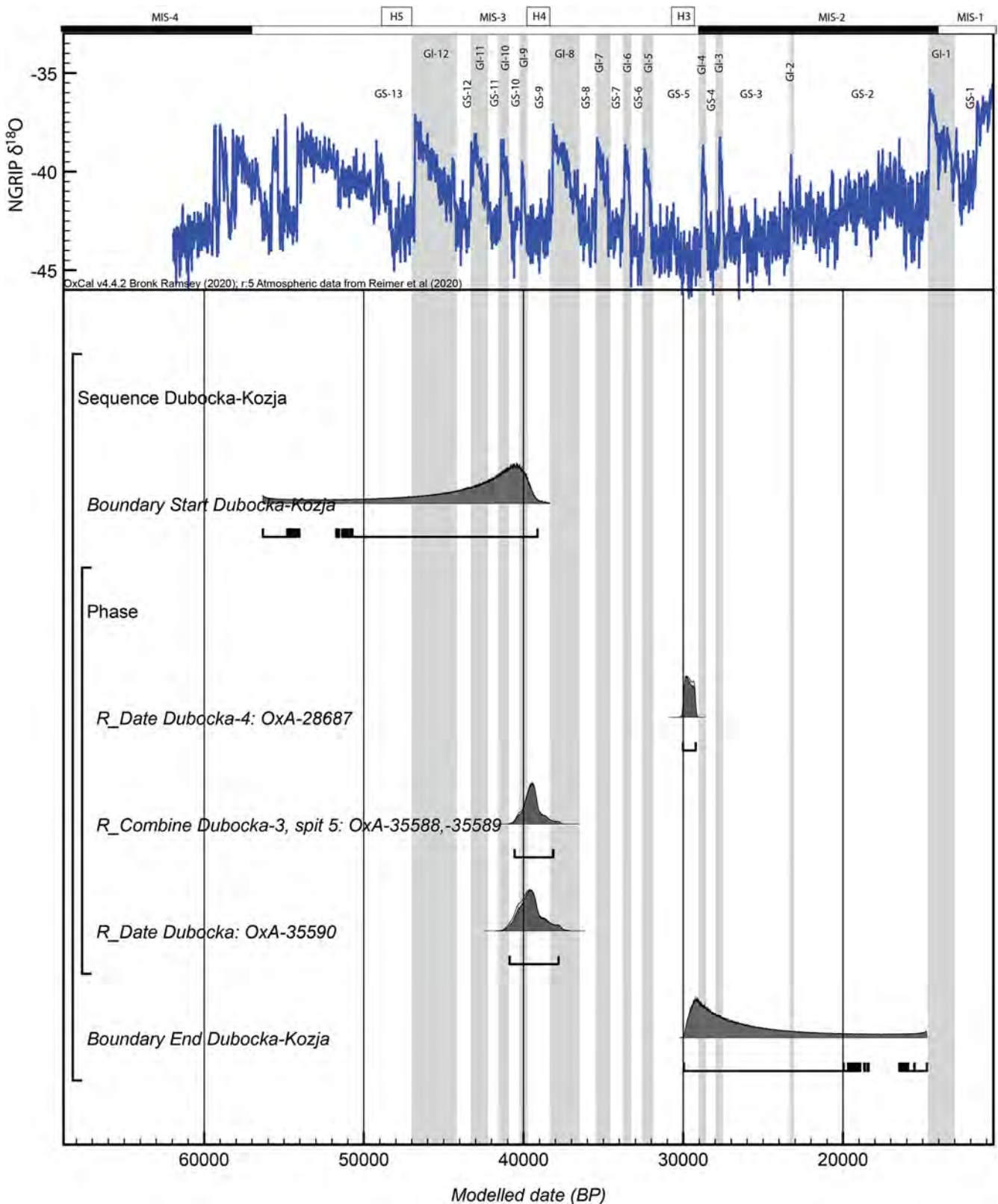
Figure 22. Bayesian modelling of all available dates from DK plotted against the North Greenland (NGRIP) \delta^{18}\text{O}_{\text{ice}} record and event stratigraphy; Greenland Stadal/Interstadial (GS/GI) cycles for the last 48 kyr BP (before 2000 AD). For the radiocarbon measurements, distributions in outline are the results of simple radiocarbon calibrations, solid distributions are the output from the chronological model. The large square brackets and OxCal v. 4.4 CQL2 keywords define the overall model exactly. [Color figure can be viewed at wileyonlinelibrary.com ]
