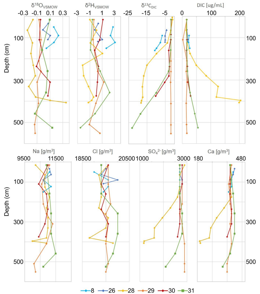
FIGURE 8 Profiles of \delta^{18}\text{O} , \delta^2\text{H} , \delta^{13}\text{C}_{\text{DIC}} , DIC, \text{Na}^+ , \text{Cl}^- , \text{SO}_4^{2-} and \text{Ca}^+ concentrations in pore water from sediment cores TAN1703-8, 26, 28, 29, 30 and 31. Locations are shown in Figure 2
