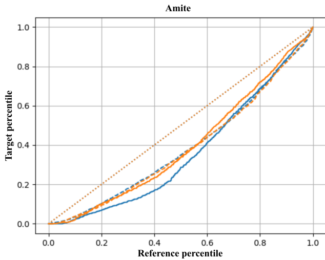
Figure 4. The transformation functions of the 1951–1960 FDC (solid) and API (dashed) to the target periods 1971–1980 (blue) and 1981–1990 (orange) for Amite. For the sake of comparison, the diagonal is dotted in orange.
