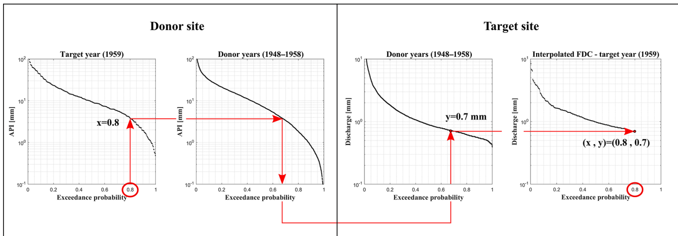
Figure 6. Illustration of FDC generation using the interpolation with the API of the donor site as a proxy.
