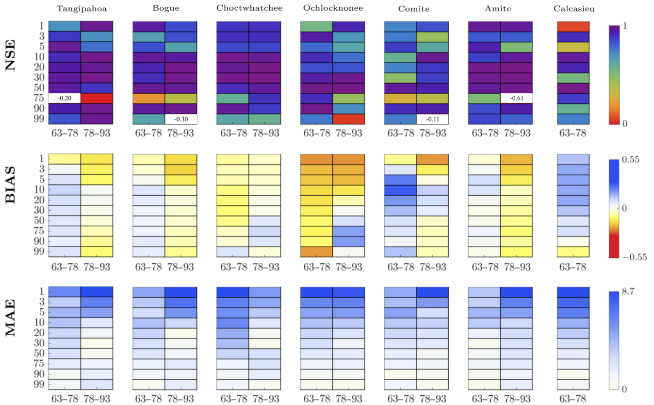
Figure 11. Performance measures NSE, BIAS and MAE evaluated for specific percentiles (on the y axis) and for specific 15 target years (i.e., 1963–1978 and 1978–1993 on the x axis). The donor decade is 1948–1963 and the donor basin is Blanco (TX). Each target basin is indicated in the corresponding box. Negative values of the NSE are reported in the corresponding box.
