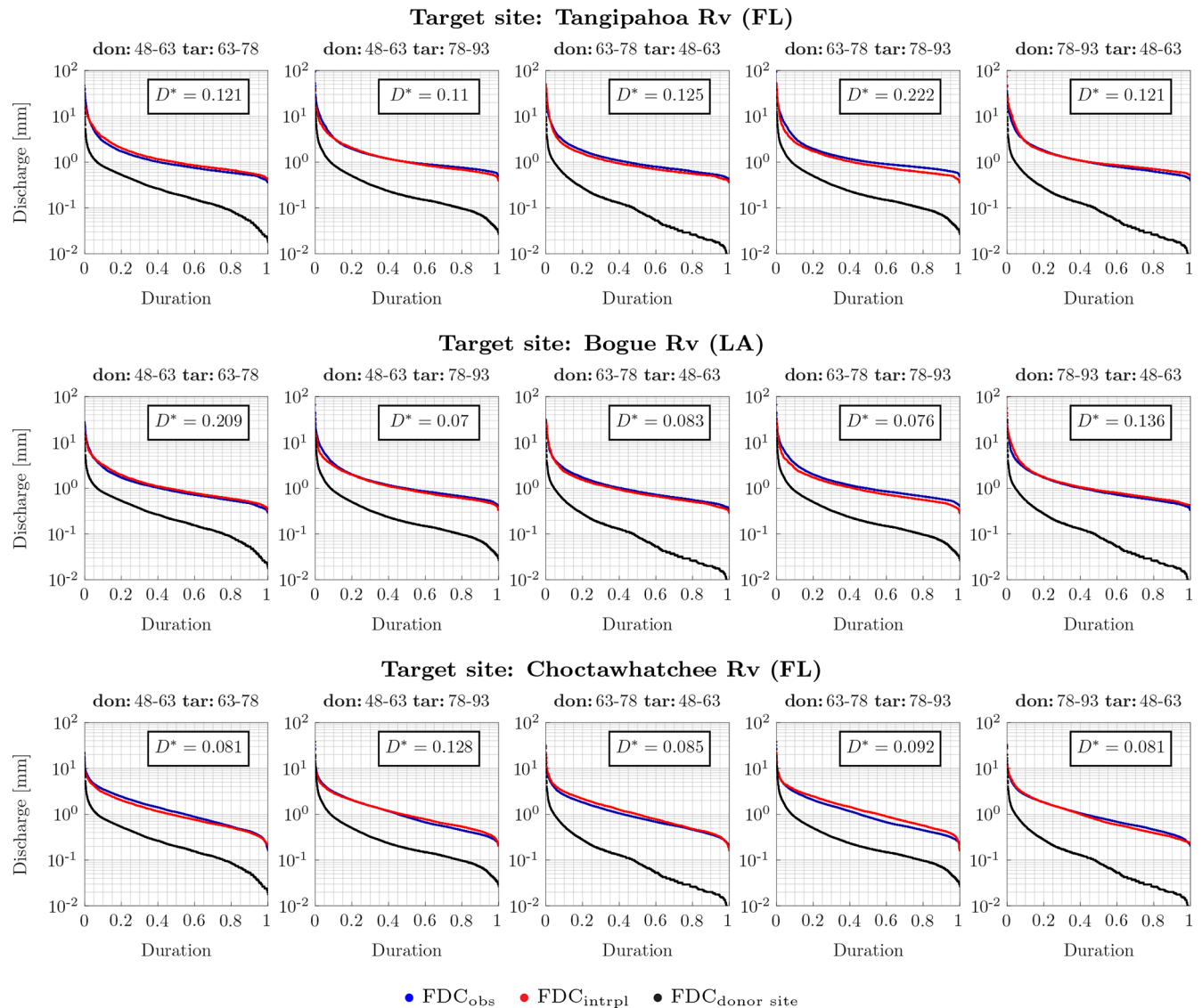
Figure 8. Interpolated FDC at Tangipahoa River (FL), Bogue River (LA) and Choctawhatchee River (FL), in the upper, middle and lower panels, respectively. The donor basin is Blanco River (TX). The donor and target years are periods of 15 years. The blue and red dots are observed and interpolated FDC, respectively, at the target basin during the target period; the black dots are the observed FDC at the donor basin during the target period. In each box the KS distance, D^* , is reported. The p value of D^* is always around zero.
