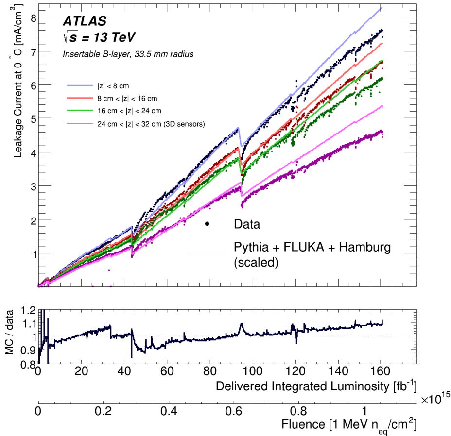
Figure 4. The measured and predicted leakage currents for sensors on the Insertable B -layer, both normalized to 0^\circ\text{C} for four module groups spanning |z| < 8\text{ cm} , 8 < |z| < 16\text{ cm} , 16 < |z| < 24\text{ cm} , and 24 < |z| < 32\text{ cm} . Modules in the highest |z| region use 3D sensors. The A and C sides of the detector ( z > 0 and z < 0 ) are consistent with each other and averaged. The dominant time-independent uncertainty of 10% is not included to avoid overlapping bands. The prediction is based on the thermal history of the modules combined with the Hamburg Model for modelling changes in the leakage current and PYTHIA + FLUKA for simulating the overall fluence. For all four predictions, the overall scale normalization is based on a fit to the data across the entire range. Normalization factors are determined per |z| region. The lower panel shows the ratio of the prediction to the data for the innermost module group. Similar MC/data trends are observed for the other three |z| regions. For illustration, the fluence is shown as a lower horizontal axis using the nominal luminosity-to-fluence from simulation at |z| = 0 .
