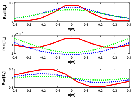
Figure 4. Real part of scattering field from a sphere-I translated along z -axis at z = 0.4 m (red solid line), z = 0.5 m (blue dot line) and z = 0.6 m (green dot line). Here, radius of sphere-I a = 0.2 m, radius of sphere-II c = 0.1 m
