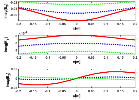
Figure 7. Imaginary part of scattering field from a sphere-I translated along z -axis at z = 0.4 m (red solid line), z = 0.5 m (blue dot line) and z = 0.6 m (green dot line). Here, radius of sphere-I a = 0.1 m, radius of sphere-II c = 0.1 m
