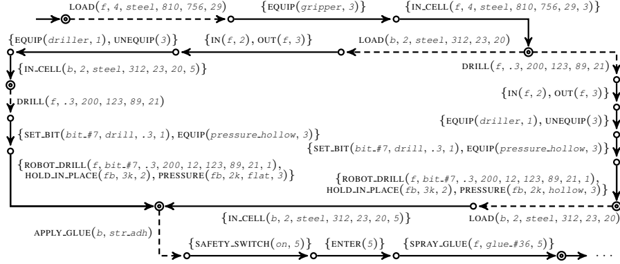
Figure 6: A fragment of a possible controller for \delta_F^0 that realizes \delta_R^0 as in the running example, represented as a control structure in which double-circled control states correspond to states q of \mathcal{T} such that q \models \phi_{OK} , i.e., it is the turn of player ENVIRONMENT. Dashed transitions from these control states are labelled with the next action of the recipe, and the rest with compound actions for the facility process (we do not include NOP actions for brevity). Each control state is associated to configurations of \delta_F^0 and \delta_R^0 , indicating their current program and situation, but these are not shown for brevity.
