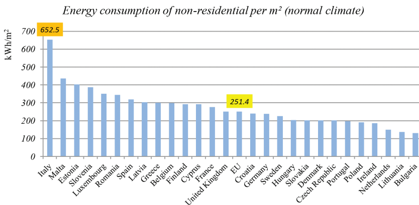
Figure 2: Energy consumption of non-residential per m 2 (normal climate) (source: https://ec.europa.eu/energy/eu-buildings-datamapper_en , 2020).
