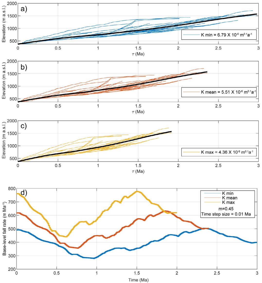
FIGURE 8 (a) Colored lines = empirical \tau plots for the entire upper Aniene river basin. Black line = mean best-fit \tau plots resulting from inverse modeling, where m = 0.45 and K = K_{\min} . (b) As (a), but for K = K_{\text{mean}} . (c) As (a), but for K = K_{\text{max}} . (d) The linear river inversion curves describing the uplift rate histories, obtained for K_{\text{max}} , K_{\text{mean}} , and K_{\min} . The parameters chosen in the modeling are described in the text and summarized in the panel
