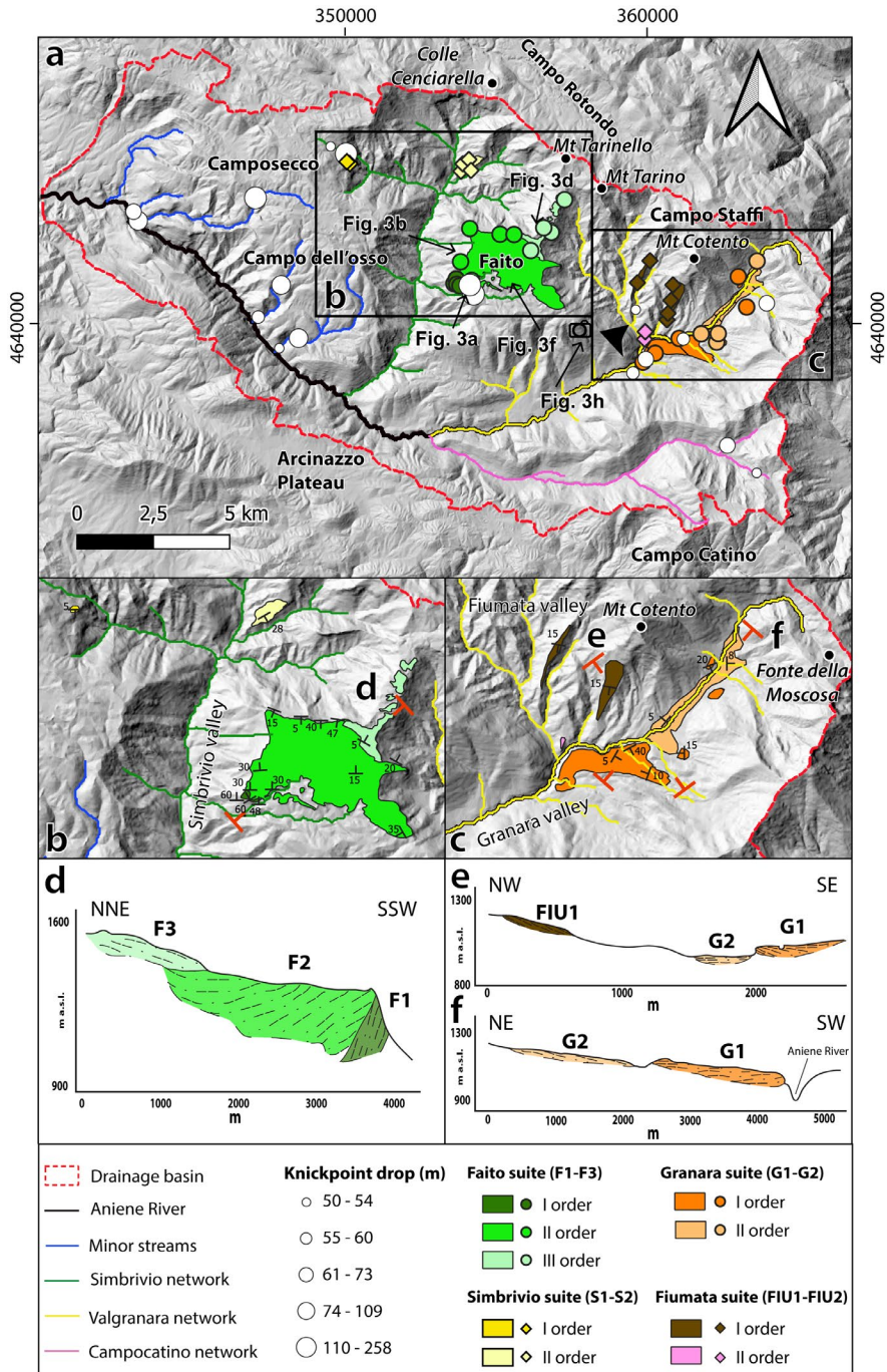
FIGURE 2 (a) Hillshade map of the study area in which the outcrops of the continental clastic deposits, the related ordered points (in correspondence with the erosive base outcrop), the knickpoints, and the geological sections are shown. (b) Zoom on the Faito and Simbrivio sequences. (c) Zoom on the Granara and Fiumata sequences. (d)–(f) Geological cross-sections of the Faito, Granara, and Fiumata suites. The coordinate system is WGS84-33N, EPSG: 32633. The hillshade map is derived from the 10 m-resolution TINITALY DEM (Tarquini & Nannipieri, 2017) [Correction added on October 3, 2021, after first online publication: The figures 2 and 3 are interchanged.]
