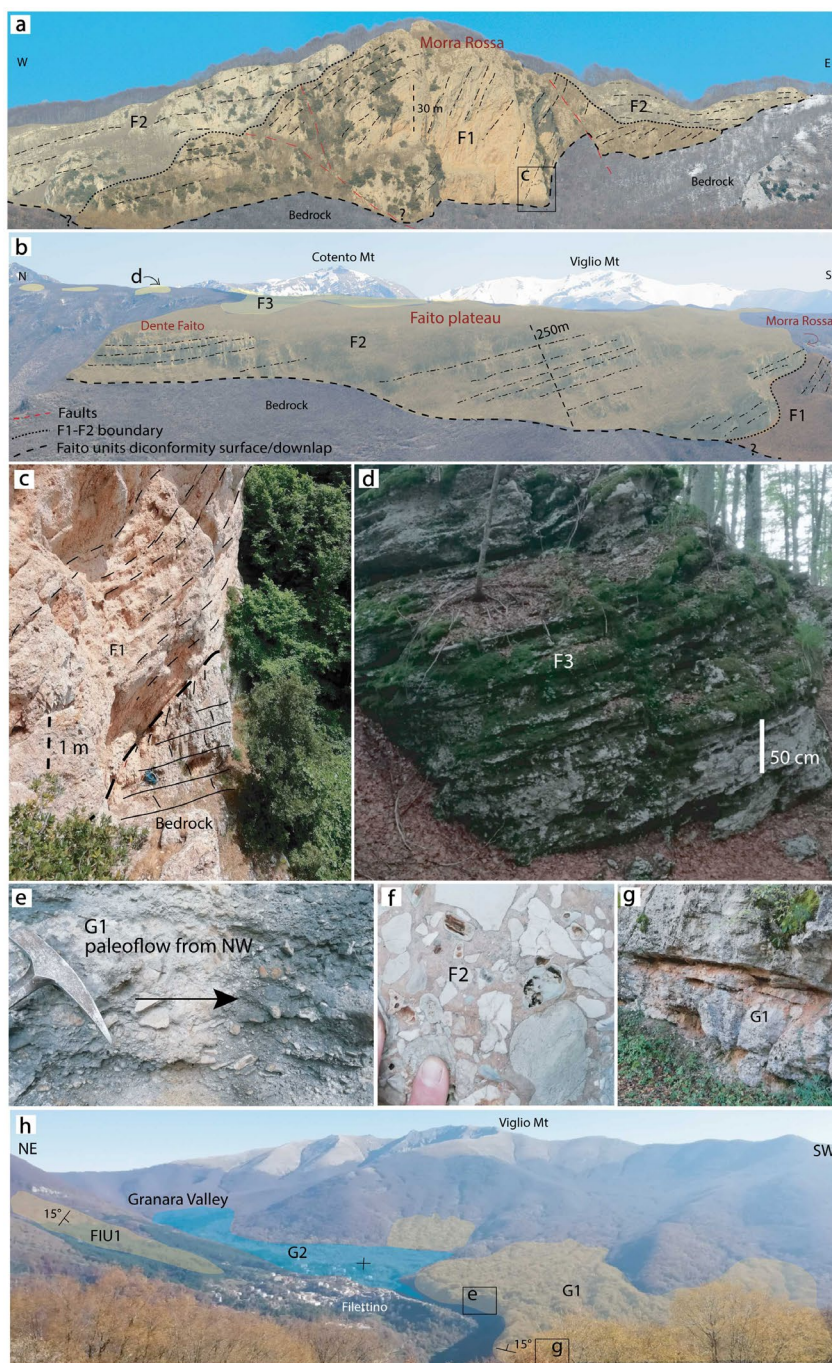
FIGURE 3 Photos taken during the field survey. (a) The spectacular morphology of the south side of the Faito plateau consisting of bedrock cliffs and overhangs, localized in correspondence with the disconformity boundary with the cretaceous bedrock, where F1 proximal facies crop out. (b) West side of the Faito plateau in a N–S panoramic view with the layering of the breccia deposits clearly visible. (c) Detail of the very steep beds, clast-supported and heterometric F1 unit, and the boundary with the bedrock. (d) Faito's F3 unit, well organized, with cross-laminations and channelization features. (e) Detail of clast embracement in G1 unit (Granara valley). (f) Close-up on the matrix-supported texture of F2 Faito's breccia. (g) G1 Granara deposit—layers dip in the opposite direction to the present-day slope. (h) Panoramic view of Granara valley. See Figure 2 for locations
