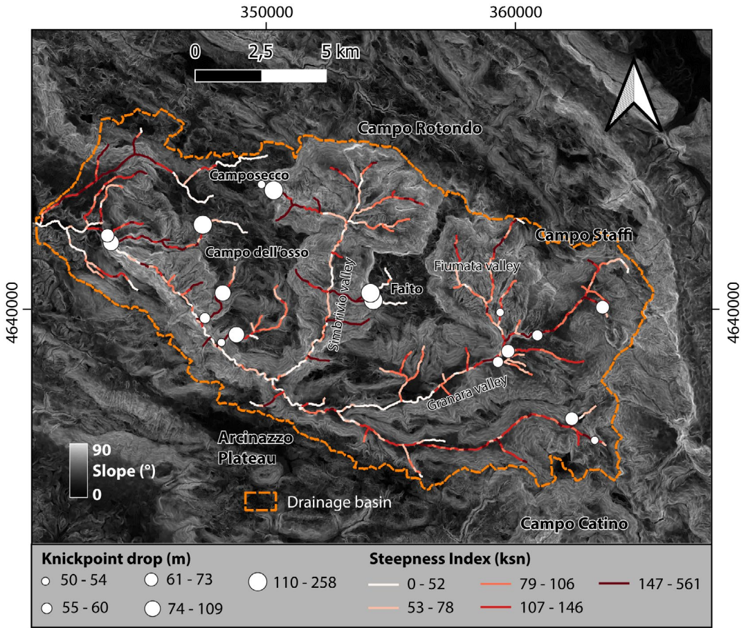
FIGURE 7 Slope map with k_{sn} values associated with the stream networks of the upper Aniene river basin (including Simbrivio, Granara, and Campocatino sub-catchments). The k_{sn} values were computed following Equation (3), keeping fixed the mn ratio, or \theta , at -0.45 , resulting from the linear regression shown in Figure 5. The coordinate system is WGS84-33N, EPSG: 32633. Both the slope map and the k_{sn} values are derived from the 10 m-resolution TINITALY DEM (Tarquini & Nannipieri, 2017)
