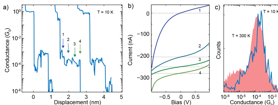
Figure 6. (a) Breaking traces, recorded in the presence of OPE3 (sample 3) at a temperature of 10 K (bias 0.1 V). The traces have been offset along the x -axis for clarity. (b) Current–voltage characteristics measured during the central breaking trace shown in (a), shifted along the y -axis for clarity. (c) Conductance histogram built from molecular low temperature and room temperature conductance traces. Adapted with permission from ref 22. Copyright American Physical Society.
