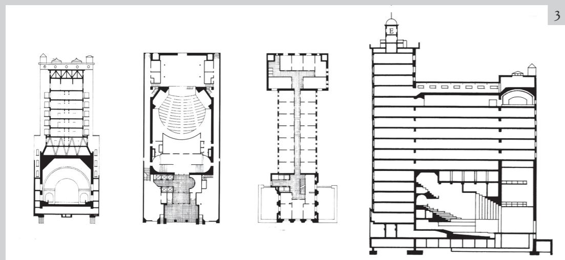
Figure 3 Louis Sullivan, Schiller Building (ex Garrick Theatre) , 1890. Cross section, ground floor plan, standard floor plan and longitudinal section of the building built in Chicago in 1890 and destroyed in the 1960s. CIOTOLI 2017, p. 85.
