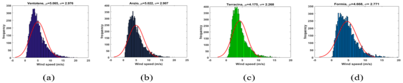
Figure 7. The histogram with a normal distribution fit of the wind speed data for Lazio ports: (a) Ventotene, (b) Anzio, (c) Terraciana, and (d) Formia. The estimated fittest normal distribution parameters: mean and variance are shown per each port.
