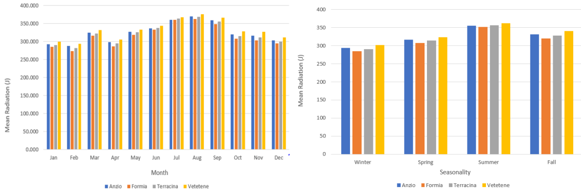
Figure 5. Shows a monthly and seasonality solar radiation using hourly time series from 2020 to 2021.
