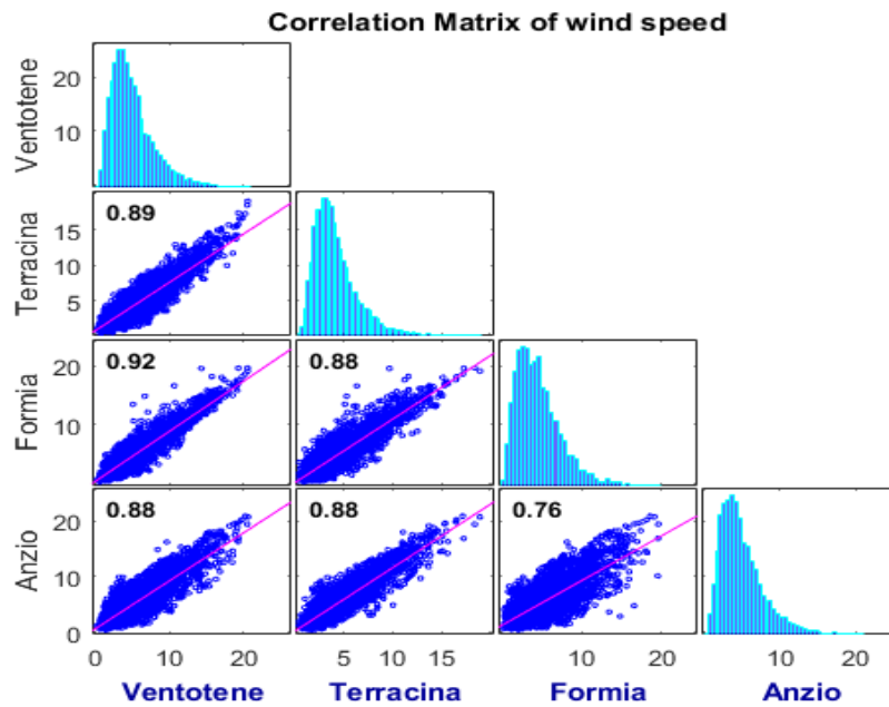
Figure 8. The Pearson's linear correlation coefficients of pairs ports wind speed data are depicted using scatter plots of variable pairs (Ventotene, Anzio, Terraciana, and Formia) in the off diagonal. The slopes of the lines in the scatter plots notify the represented correlation coefficients.
