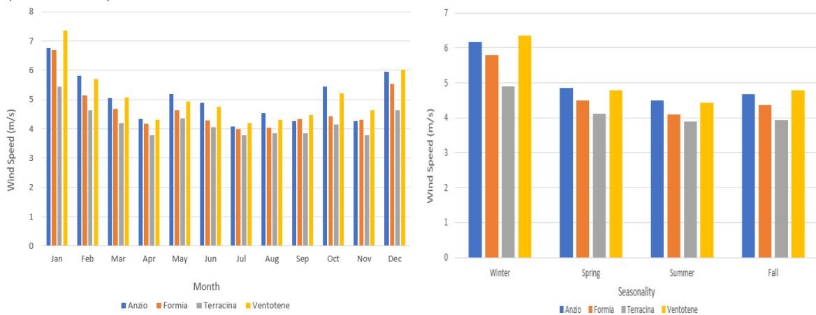
Figure 3a, b) shows a monthly and seasonality wind speed using hourly time series from 2020 to 2021.
