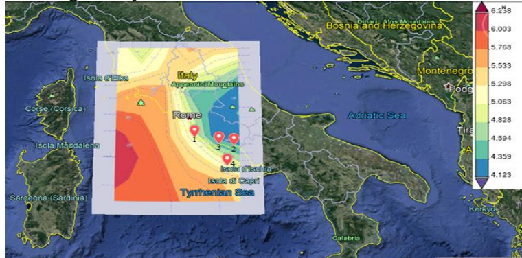
Figure 2. Surface wind speed monthly 0.5 \times 0.625 deg. m s^{-1} over 2011-May - 2021-Mar, Region 10.0707E, 39.6929N, 14.3334E, 43.648N.
