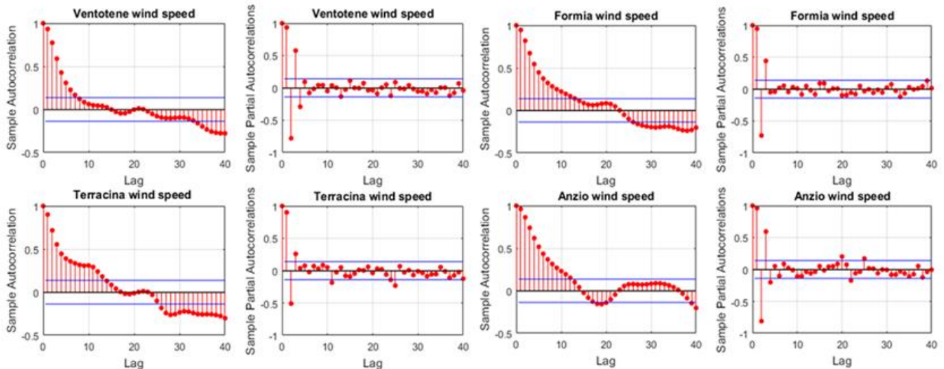
Figure 9. The sample autocorrelation function (ACF) and partial autocorrelation of the univariate, stochastic wind speed time series with confidence bounds for four ports (Ventotene, Anzio, Terraciana, and Formia).
