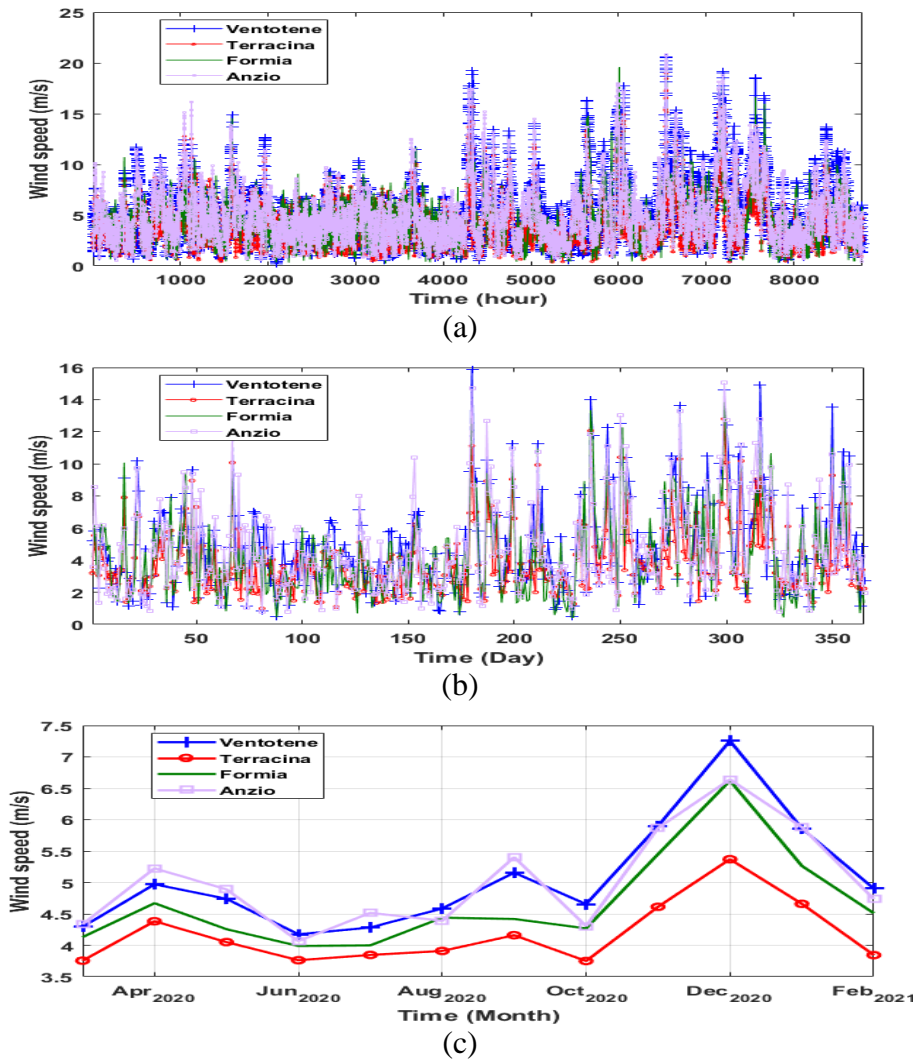
Figure 6. Sequential wind speed patterns of Lazio ports: Ventotene, Terraciana, Formia and Anzio recorded per hour, day and months.
