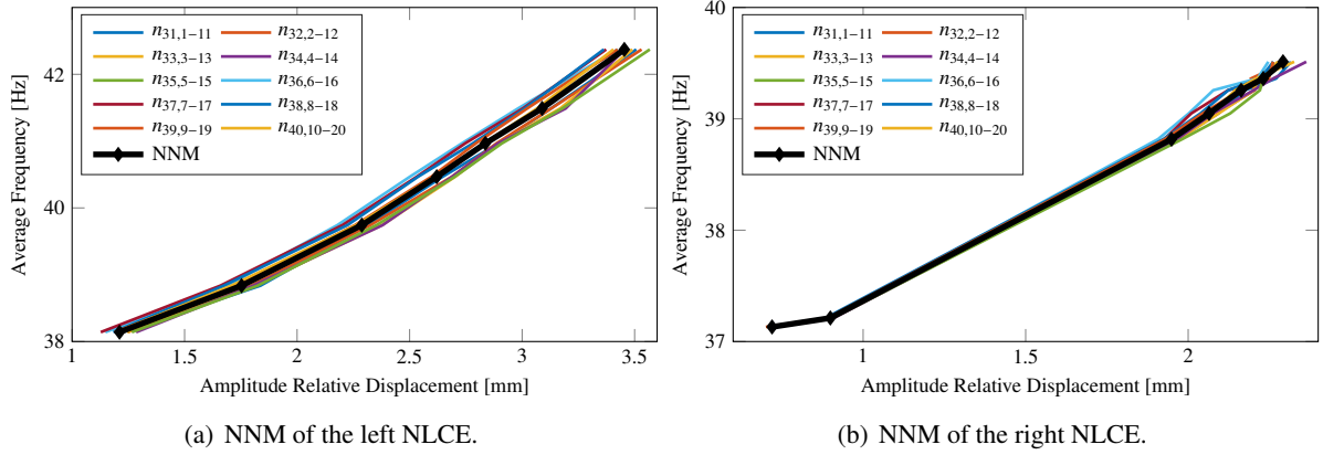
Figure 8: NNMs of the two NLCEs.
