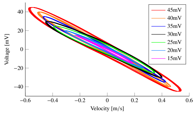
Figure 5: Resonance condition in which the measured velocity of point 11 is almost 180^\circ out-of-phase with respect to the input signal at the 7 excitation levels.
