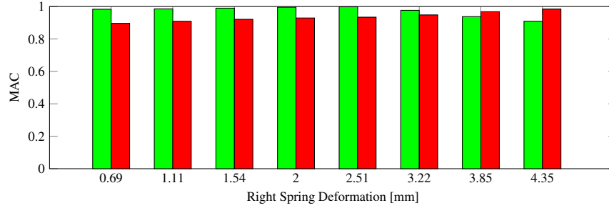
(b) MAC between numerical and experimental results: ■ using results from CP with experimentally identified NLCEs parameters; ■ using results from CP with optimized NLCEs parameters.
