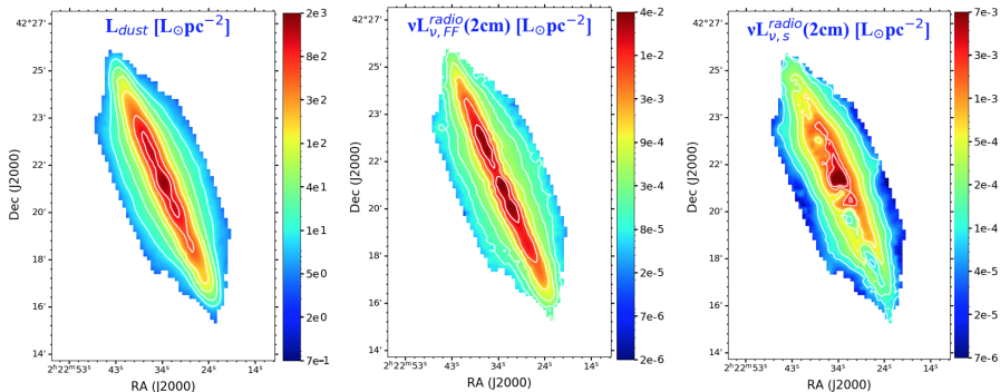
Figure 3. Maps of the model-inferred luminosity for the dust emission (left panel), the free-free luminosity at 2 cm (middle panel) and the synchrotron luminosity at 2 cm (right panel). The colorbar on the right in each panel indicates the luminosity in units of L_{\odot}\text{pc}^{-2} .
