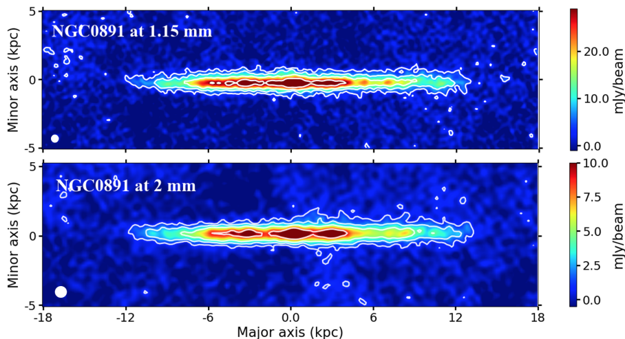
Figure 1. NIKA2 high-resolution millimeter observations of NGC 891 at 1.15 (top panel) and 2 mm (bottom panel). The maps are presented in their native resolution ( 11.1'' and 17.6'' at 1.15 and 2 mm respectively; indicated by the white circles in each panel) and they are rotated by 22.9^\circ (the position angle of the galaxy). Their sky RMS values are 1.0 \text{ mJy beam}^{-1} and 0.3 \text{ mJy beam}^{-1} at 1.15 mm and 2 mm. The surface brightness contours correspond to 3.5, 8, 15 and 30 \times \text{RMS} .
