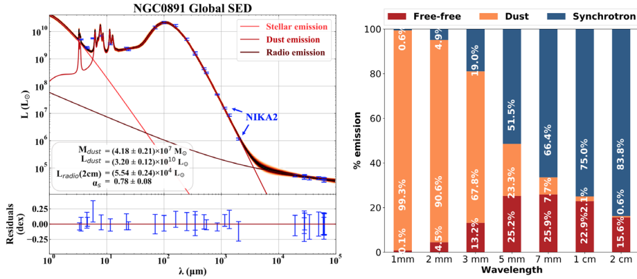
Figure 2. Left panel: the global SED of NGC 891 with multiwavelength data ranging from 3.4 \mu\text{m} to 6.3 \text{ cm} . The curve passing through the photometric data is the best fitted model with the width of the curve indicating the uncertainty of the model along the spectrum. The emission components of the total SED of the galaxy, stellar, dust and radio, are plotted with orange, red and brown color respectively. The residuals between the observed and the model predicted fluxes are given in the graph below the SED in dex. Right panel: An emission decomposition plot for characteristic wavelengths in the spectral range between 1 \text{ mm} to 2 \text{ cm} . The percentage of the dust emission is presented with orange color, while red and blue colors are used for percentages of the free-free and the synchrotron emission respectively.
