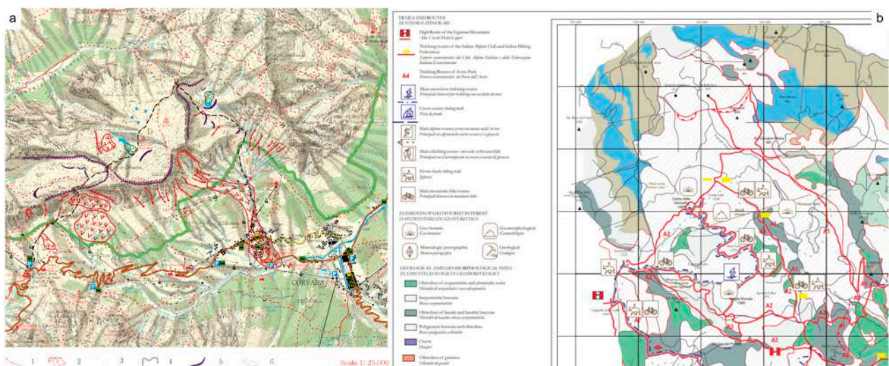
Figure 2. Examples of geotourism map for amateurs of Earth Sciences. (a) Excerpt from the leaflet of the geological-geomorphological itinerary in Val Badia (Dolomites, Italy) (modified after [79]). (b) Excerpt from the Geo-hiking Map of the Mt. Penna and Mt. Aiona area (Aveto Natural Park, Italy) (modified after [80]).
