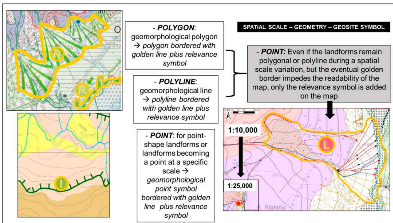
Figure 7. Examples of the graphical representation changes with the spatial scale.
