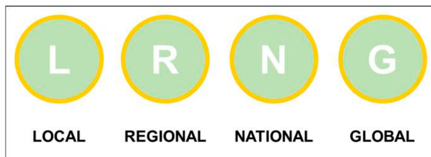
Figure 6. Examples of symbols to represent a geosite as a point according to their importance.
