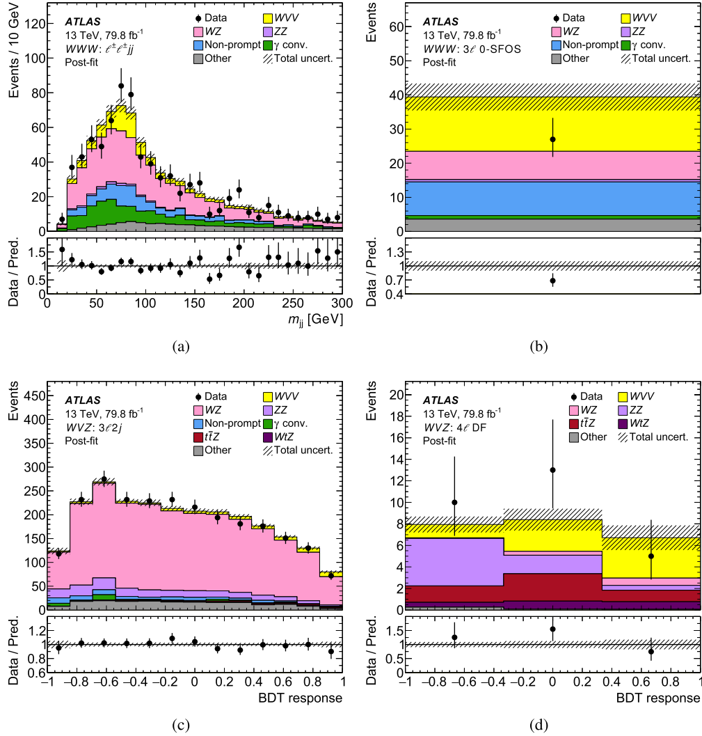
Fig. 4. Post-fit distribution of (a) m_{jj} for the WWV \rightarrow \ell\nu\ell\nu qq analysis ( e\bar{e}, e\mu, \mu e, \mu\mu combined), (b) number of events for the WWV \rightarrow \ell\nu\ell\nu\ell\nu analysis, and the BDT response in the (c) 3\ell -2j and (d) 4\ell -DF channels for the WVZ analysis. The contributions denoted “Other” are dominated by the (a) W^\pm W^\pm + 2\text{jets} , (b) t\bar{t}W and (c) t\bar{t}Z process, respectively. The uncertainty band includes both statistical and systematic uncertainties as obtained by the fit.
