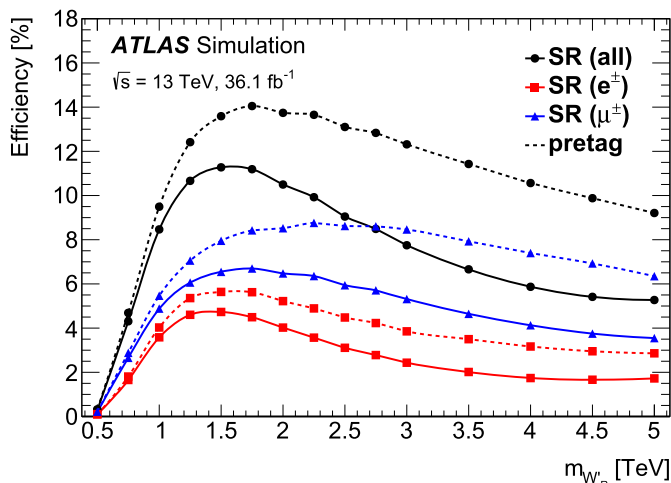
Fig. 2. Signal selection efficiency (efficiency is defined as the number of events passing all selections divided by the total number of simulated W' \rightarrow tb \rightarrow \ell\nu b\bar{b} events) in the signal region as a function of the simulated W'_R mass. Efficiencies are shown for: all channels combined (full circle), electron channels only (full square) and muon channels only (full triangle). For reference, signal efficiency curves are also shown without the requirement on b -tagging (pretag selection: dotted lines).
