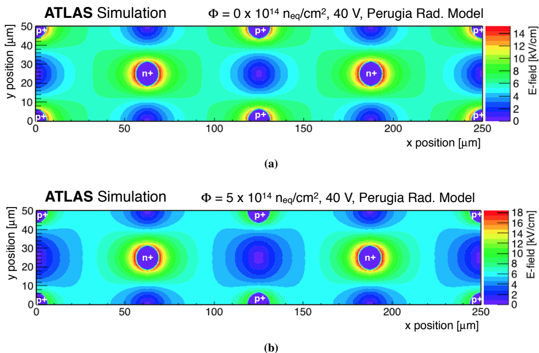
Figure 17. Simulated magnitude of the electric field as a function of local x and y in an ATLAS IBL 3D sensor with a bias voltage at V_{\text{bias}} = -40 V for (a) an unirradiated sensor and (b) for a fluence of 5 \times 10^{14} n eq /cm 2 . The doping type of the columns is indicated.
