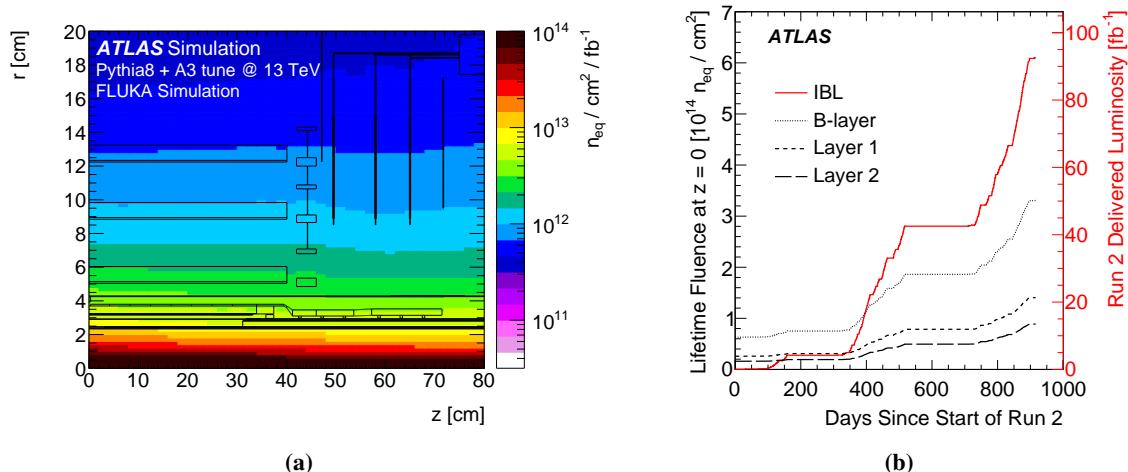
Figure 1. (a) Simulated 1 MeV n_{eq} fluence predictions shown as a function of the radial and longitudinal distance from the geometric centre of the detector for a one-quarter slice ( z > 0 and above the beam) through the ATLAS FLUKA geometry. (b) Predictions for the lifetime fluence experienced by the four layers of the current ATLAS pixel detector as a function of time since the start of Run 2 (June 3, 2015) at z \approx 0 up to the end of 2017. For the IBL, the lifetime fluence is only due to Run 2 and for the other layers, the fluence includes all of Run 1. The IBL curve represents both the fluence on the IBL (left axis) as well as the delivered integrated luminosity in Run 2 (right axis).
