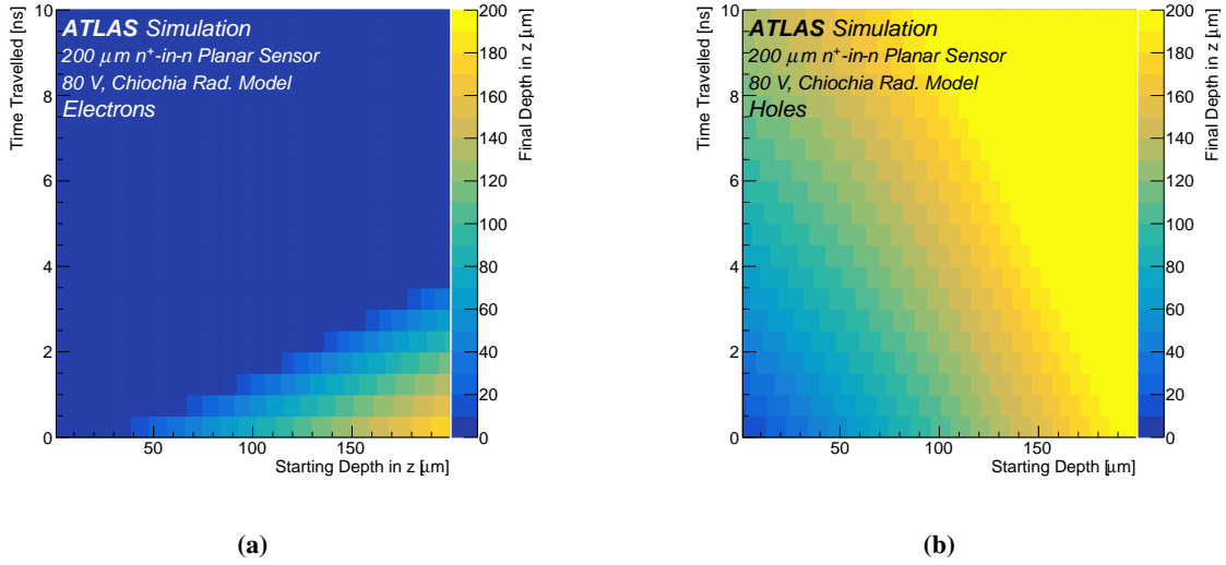
Figure 12. The z position of trapped (a) electrons and (b) holes as a function of their starting position and the time travelled for \Phi = 10^{14} n_{\text{eq}}/\text{cm}^2 . The n^+ electrode is located at the left ( z = 0 ) and the back plane at z = 200 \mu\text{m} .
