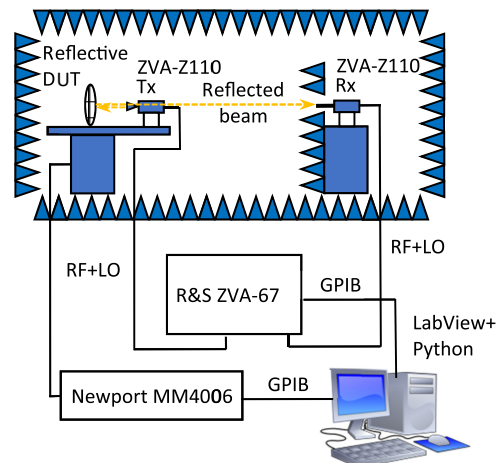
Fig. 9. Schematic diagram of the automated beam-pattern measurement system for reflective pupil characterization.
