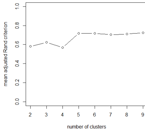
Figure 3: ClustOfVar stability analysis of the partition obtained via bootstrapped mean-adjusted Rand Index
