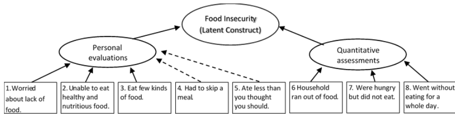
Figura 2: FIES's model of measurement: formative approach
