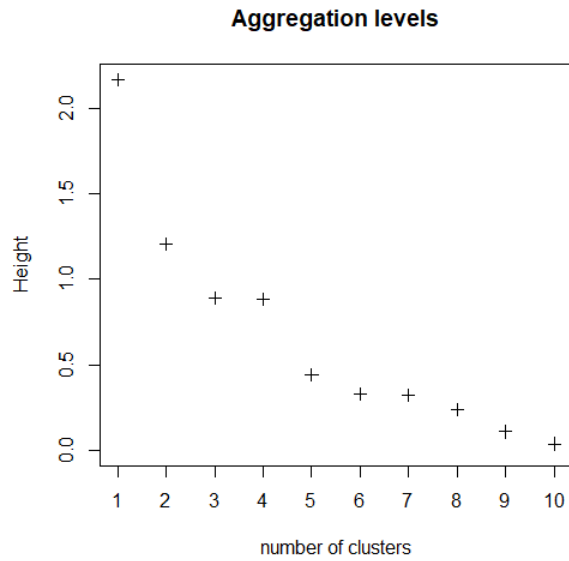
Figure 2: ClustOfVar aggregation levels
