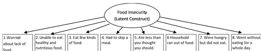
Figure 1: FIES's model of measurement: reflective approach.
