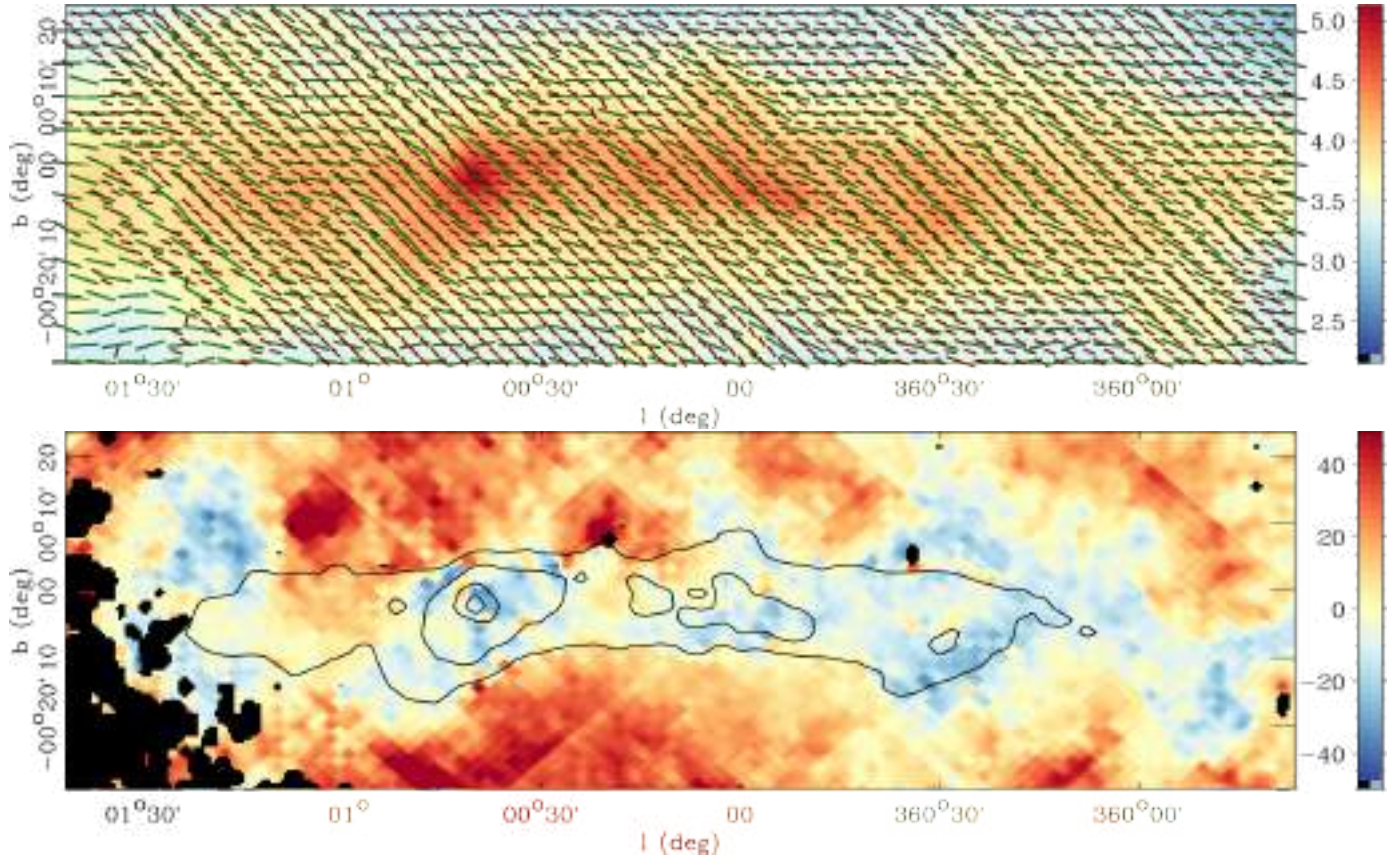
Fig. 9. Top panel: comparison between the B -field orientation as derived from the PILOT 240\ \mu\text{m} (red) and Planck 353 GHz (green) dust polarization measurements. The B -field orientation is shown as constant length line segments. The background image is the PILOT Stokes I map shown in log scale. Bottom panel: map of the angle difference (in degrees) between Planck 353 GHz and PILOT 240\ \mu\text{m} .
