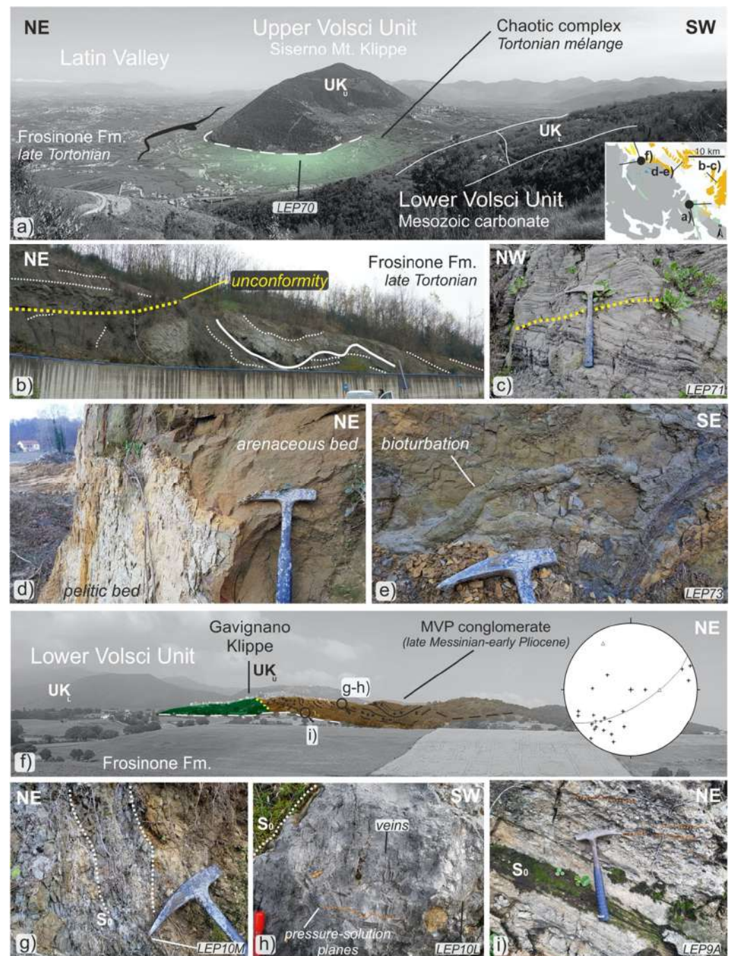
Figure 10. (a) Structural overview over two frontal klippen of the Latin Valley cropping out at Siserno Mt. where the Chaotic complex is juxtaposed to the Frosinone Fm. (b) Near Frosinone, an unconformity subdivides folded FFS units from the channelized facies on top. (c) Detail of the unconformity. (d) Vertical pelitic-arenaceous succession with (e) bioturbated levels. (f) Structural overview of the Gavignano area with stereoplot (lower hemisphere projection, equal area) of bedding and eigenvectors, that are indicative of the orientation of the axes of deformation related to the MVP thrust top conglomerates of Gavignano with (g–i) location of sampling localities. Conglomerates at the base are affected by pressure solutions and in the most calcareous beds also by veins. Sampling sites are referred to the Table in Appendix B.
