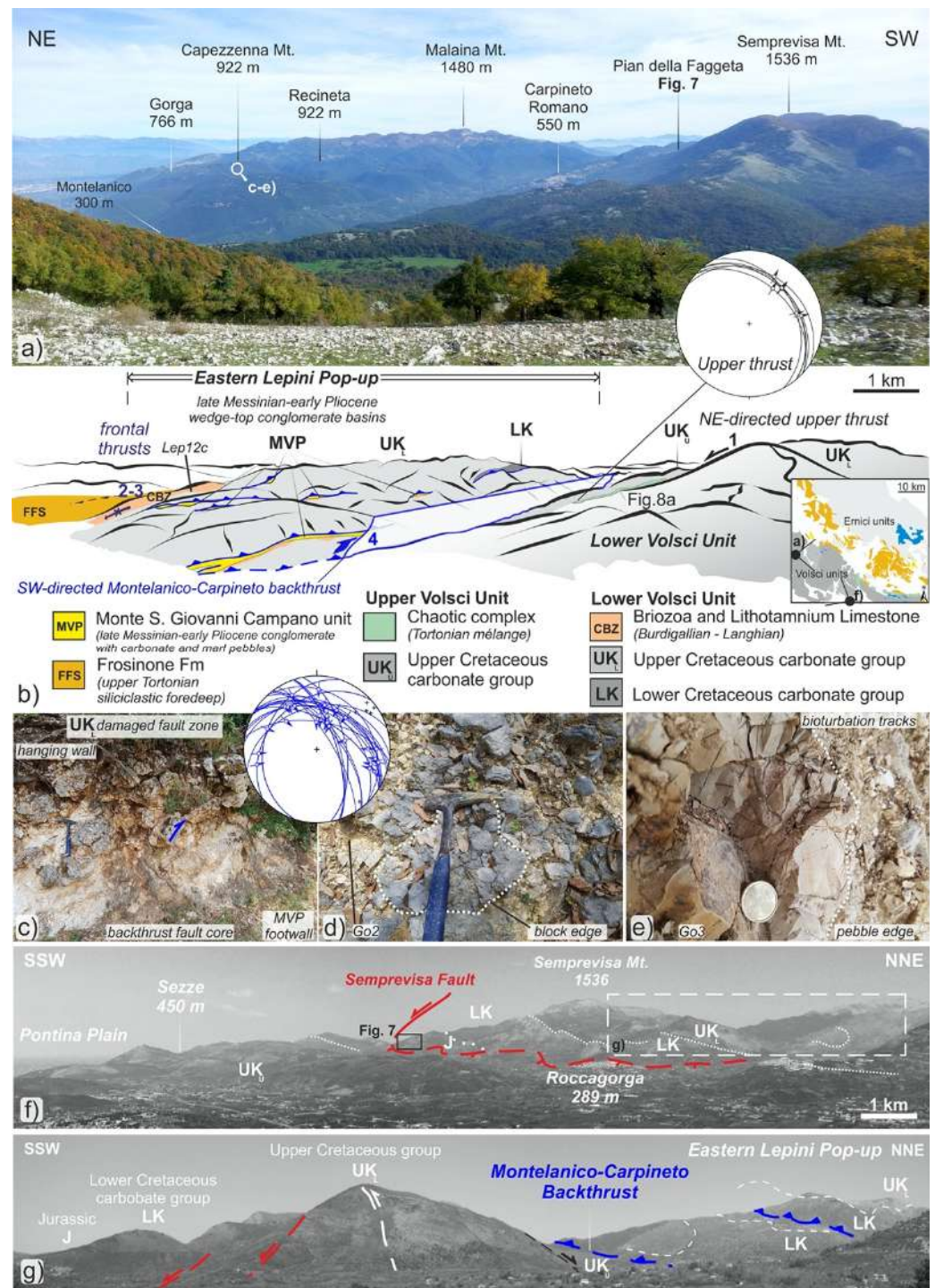
Figure 11. (a,b) Structural overview of the backthrusts in the northern Volsci Range with sampling sites (see Appendix B) and stereoplotted (lower hemisphere projection, equal area) of bedding and backthrusts. (c) Thrust zone detail. (d) Block of conglomerate within conglomerate with clayish marly matrix. (e) Pebble of bioturbated marl with chondrites. (f,g) Structural overview of the Lepini sector and the Montelanico-Carpineto backthrust continuation towards the south beneath the Eastern Lepini Pop-up.
