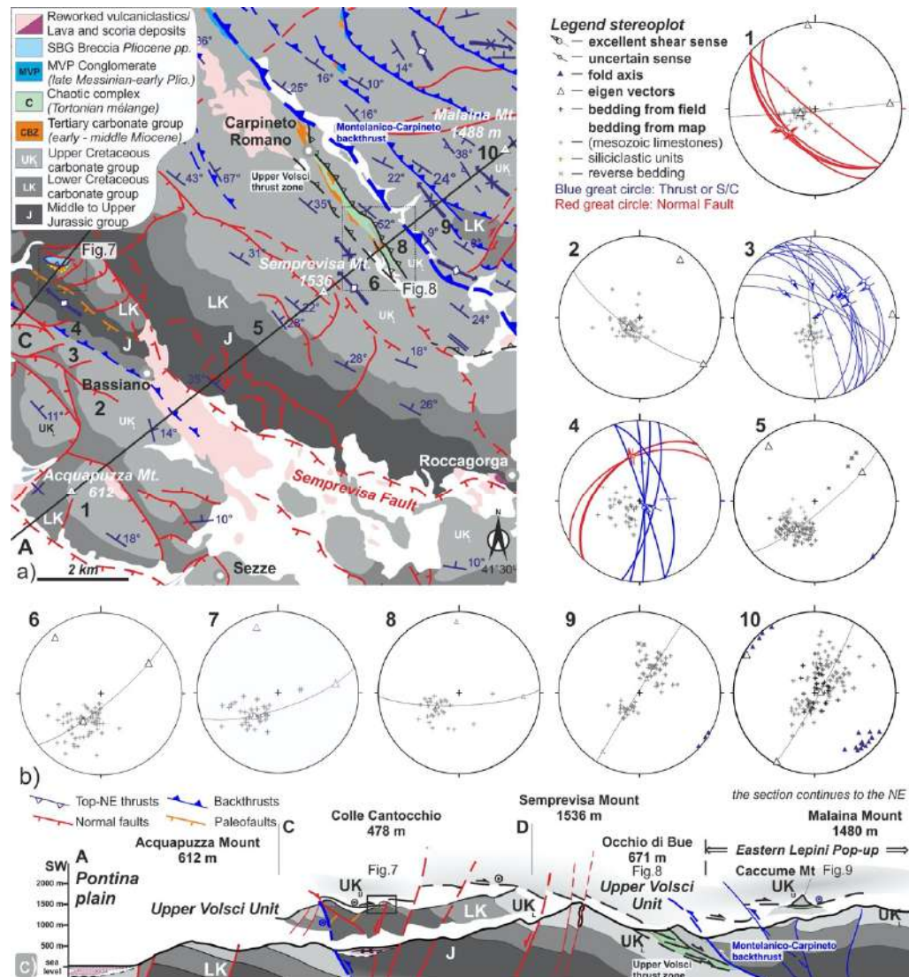
Figure 6. (a) Geological map of the western Lepini sector. (b) Stereoplots (lower hemisphere projection, equal area) summarizing orientation data for the structural elements representative of the subdivided areas in panel (a). Eigen vectors are indicative of the orientation of the axes of deformation calculated from the bedding, where the gray circles represent planes that contain the intermediate and maximum eigenvectors, as shown also by the data reported in the supplementary material. (c) Cross-section of the Volsci Range limited to the Malaina Mount to the northeast.
