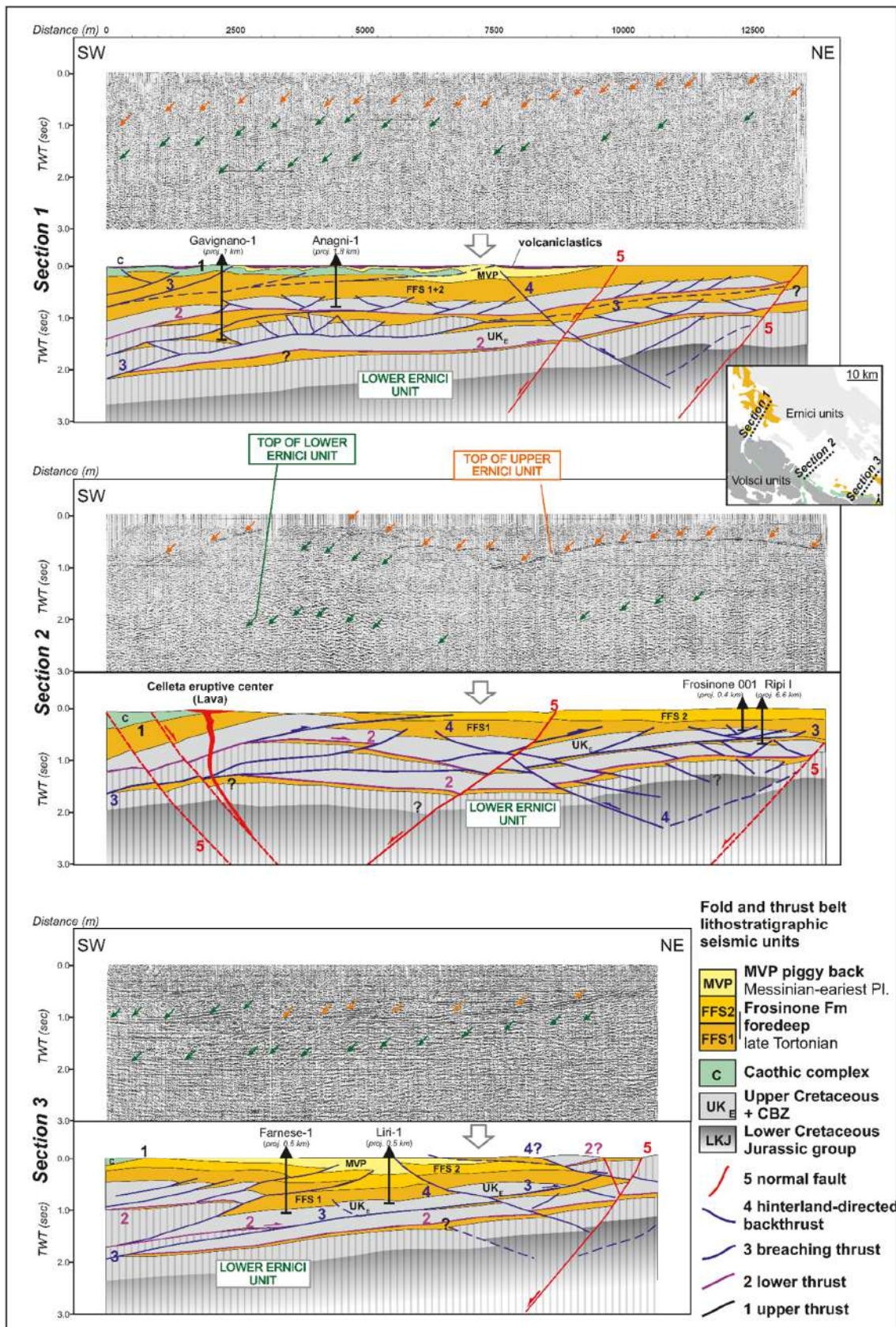
Figure 12. Two-times travel (TWT) seismic lines (from www.vidempi.com (accessed on 20 January 2021)); below, interpreted), also showing the projection of the wells. The location of both wells and seismic line traces of Section 1 (line label FR-309-80), Section 2 (FR-306-82), and Section 3 (FR-302-80) are in Figure 3. The vertical gray stripes highlight the Lower Ernici Unit.
