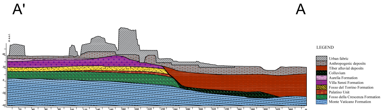
Fig. 4 - Geological cross section (track in Fig. 2). Topography derived from DSM provided by Ministry of Environment
