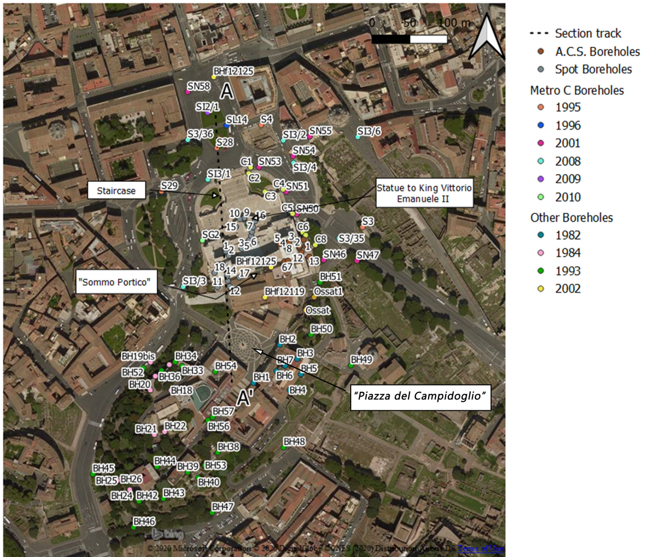
Fig. 2 - Location of the examined boreholes and track of the geological section A'-A' of Fig. 4
