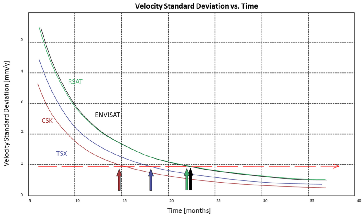
Fig. 7 - Standard deviation of the estimated average displacement rates for different satellites as a function of time for an average atmospheric noise mean square delay (after ROCCA et alii , 2013, modified)
