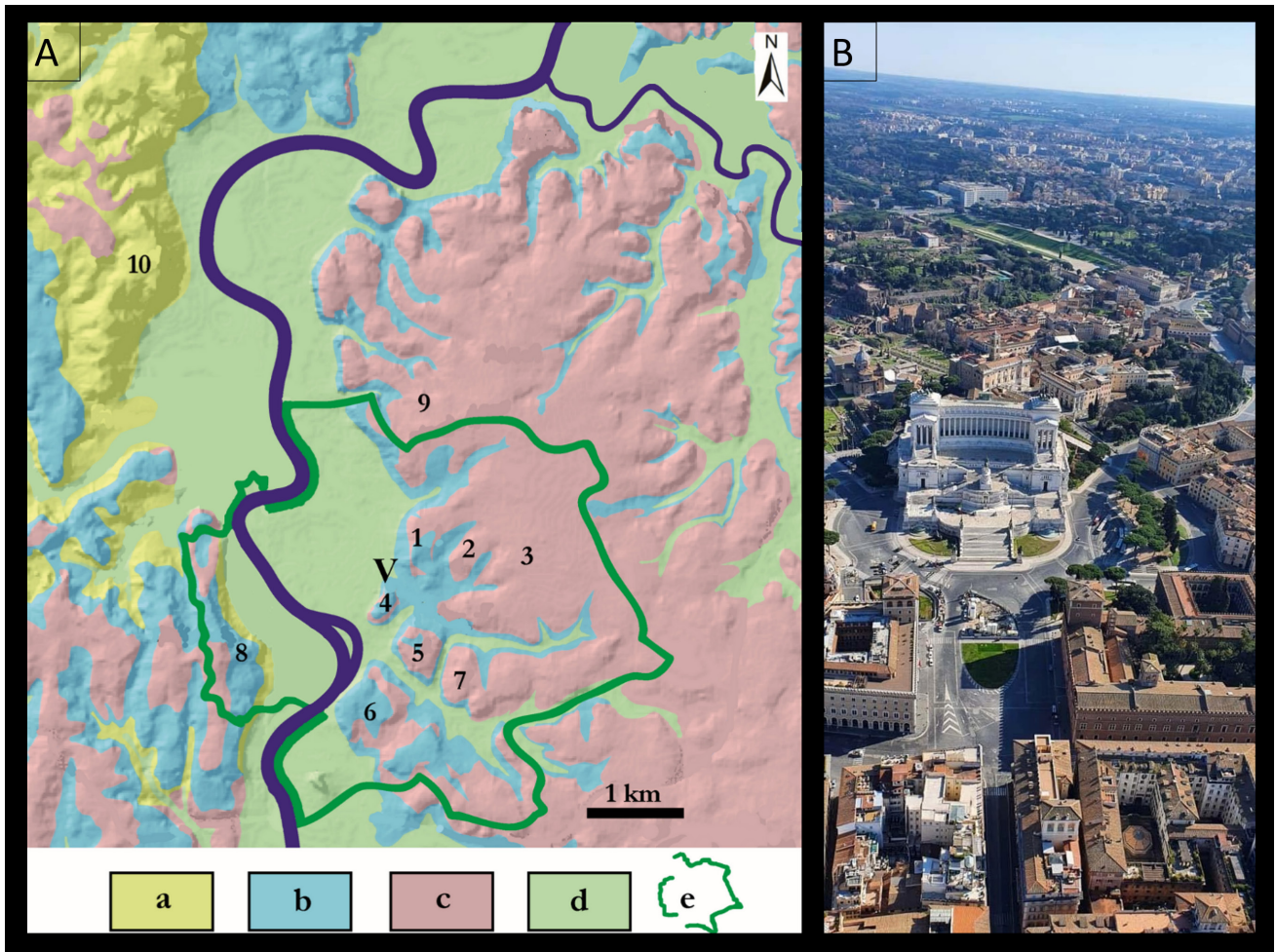
Fig. 1 - A) Hill-shade lithological sketch of Rome urban area. Legend: a) marine deposits b) continental sedimentary deposits, c) pyroclastic rocks, d) post-Wurmian alluvium, e) city center. Hills: 1) Quirinale, 2) Viminale, 3) Esquilino, 4) Campidoglio, 5) Palatino, 6) Aventino, 7) Celio, 8) Gianicolo, 9) Pincio, 10) Monte Mario. V: Vittoriano. (modified after: VERGARI et al. , 2020). B) Southward view of Piazza Venezia during the Covid 19 pandemic with the Vittoriano Monument clearly visible
