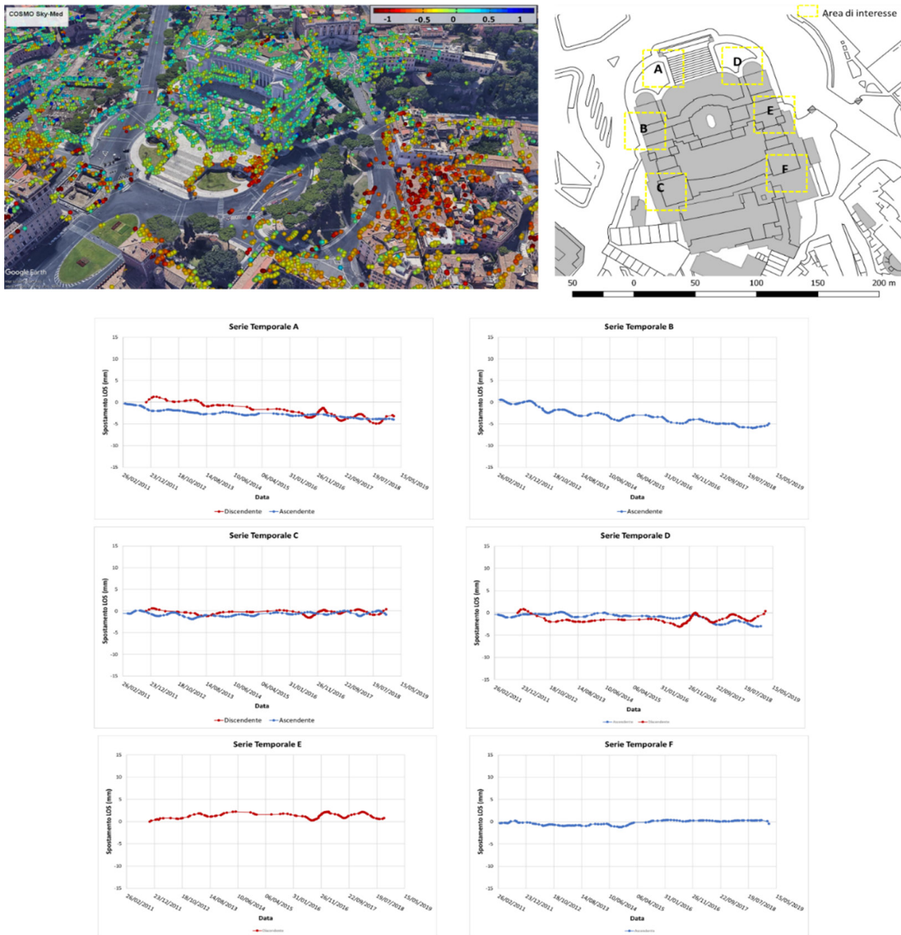
Fig. 9 - Analysis of the MP located on the Vittoriano. Data are related to the analysis performed through COSMO Sky-Med in both geometries (Descending and Ascending). Top: 3D interferometric map and location of the analyzed MP. Bottom: displacement time series representative of the 6 selected areas
