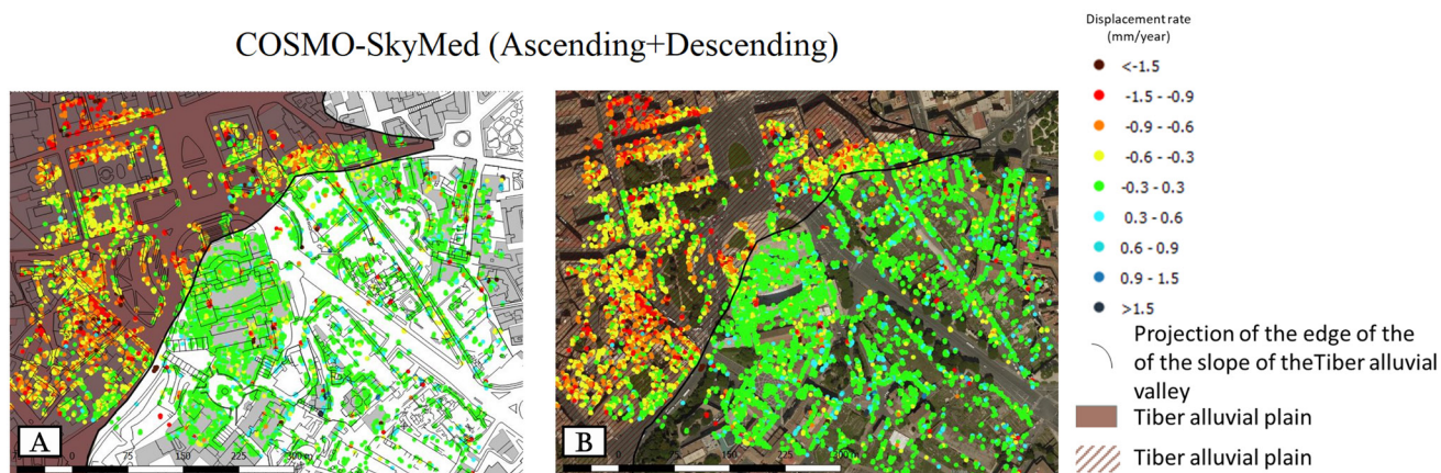
Fig. 10 - Displacement rates according to the line of sight obtained from the images COSMO Sky-Med (2011-2019), ascending and descending mode. The image A is based on the regional CTR and B on an ortho-rectified satellite image
