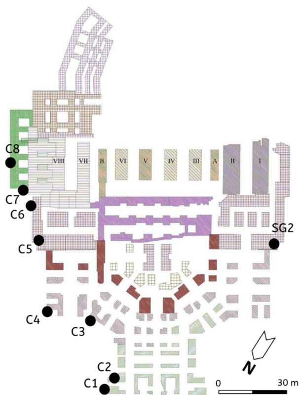
Fig. 5 - Planimetric reconstruction of the Vittoriano foundations (after GIUNTINI, 1954) with location of the Metro C boreholes and pylons number indicated in the text
