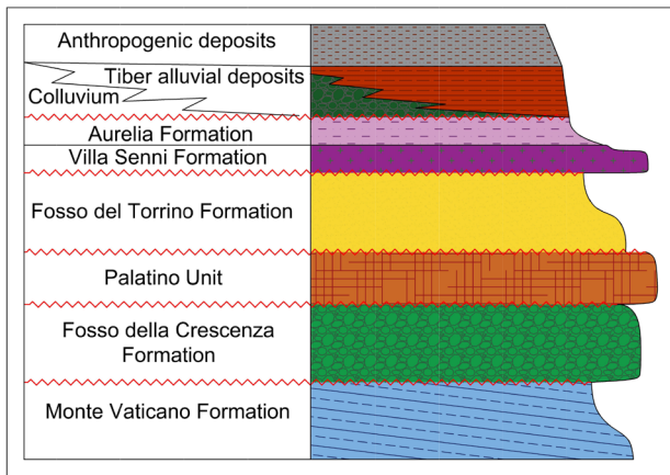
Fig. 3 - Stratigraphic column of the Arx (Capitoline Hill)
