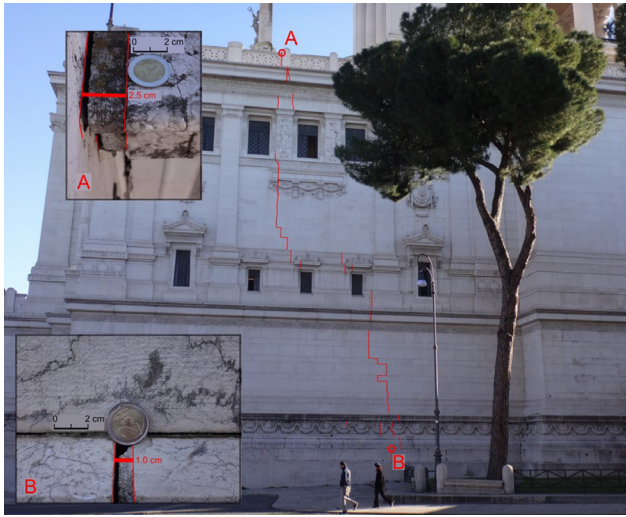
Fig. 6 - Main joints on the western perimeter wall
