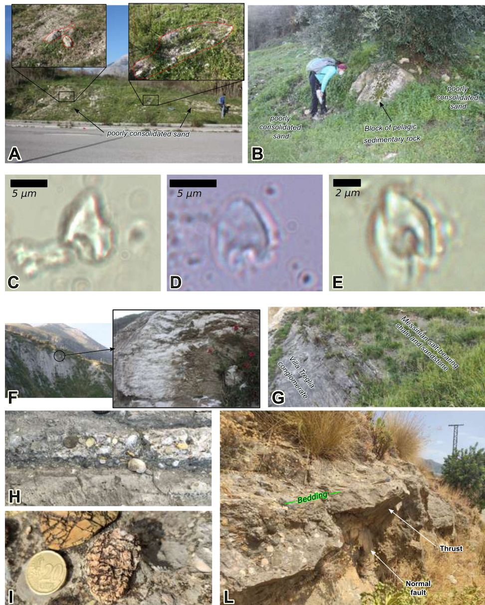
Figure 5. (a) Sedimentary mélange formed by poorly consolidated sand of the lower portion of the Messinian salt-bearing shales and sandstones, with insets showing m-sized blocks of pelagic limestones (Location 41.274694°N, 13.710114°E). (b) Block of pelagic limestone embedded within poorly consolidated sand of the lower portion of the Messinian salt-bearing shales and sandstones, Spigno section. Microphotographs showing calcareous nannofossils found in the Messinian salt-bearing shales and sandstones: (c) Amaurolithus primus , (d, e) cf. Amaurolithus primus (primitive morphotypes) (samples location in Figure 8a). (f) Panoramic photo and close up view of a Gypsum block at the topmost portion of slightly mixed and disrupted Messinian salt-bearing sandstones and shales in the Villa Treglia section (Location of the block 41.269094°N, 13.613944°E). (g) Conformable stratigraphic contact between the Messinian salt-bearing sandstones and shales and the underlying Villa Treglia Conglomerate in the Villa Treglia section (Location of the contact 41.267289°N, 13.612959°E). (h) Detail of the Villa Treglia Conglomerate showing a conglomerate level sandwiched between two calcarenite levels. (i) Detail of a pink granite clast within the Villa Treglia conglomerate. (l) Gently dipping strata of the Villa Treglia conglomerate affected by a brittle normal fault cutting and displacing a previous brittle thrust (Location of the contact 41.261963°N, 13.611167°E).
