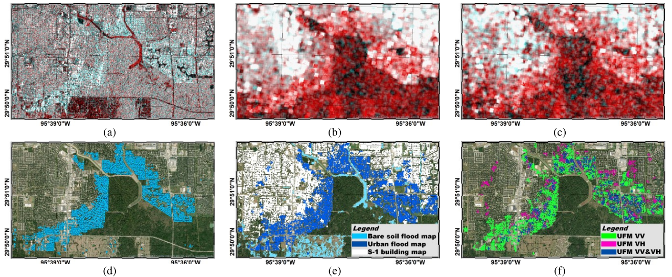
Fig. 6. AOI 2. (a) Intensity RGB composite: R = 24/08/2017 , B = G = 30/08/2017 . (b) VV and (c) VH InSAR \rho RGB composite: R = \rho_{pre}^{18-24/08/2017} , B = G = \rho_{co}^{24-30/08/2017} . (d) DG VHR imagery (31/08/2017) and crowd sourcing points of flooded buildings. (e) UFM (dark blue), flooded bare soil (light blue), nonflooded built-up areas (white). (f) VV-VH comparative UFM.
