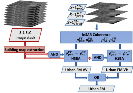
Fig. 2. Flowchart of the proposed algorithm.
