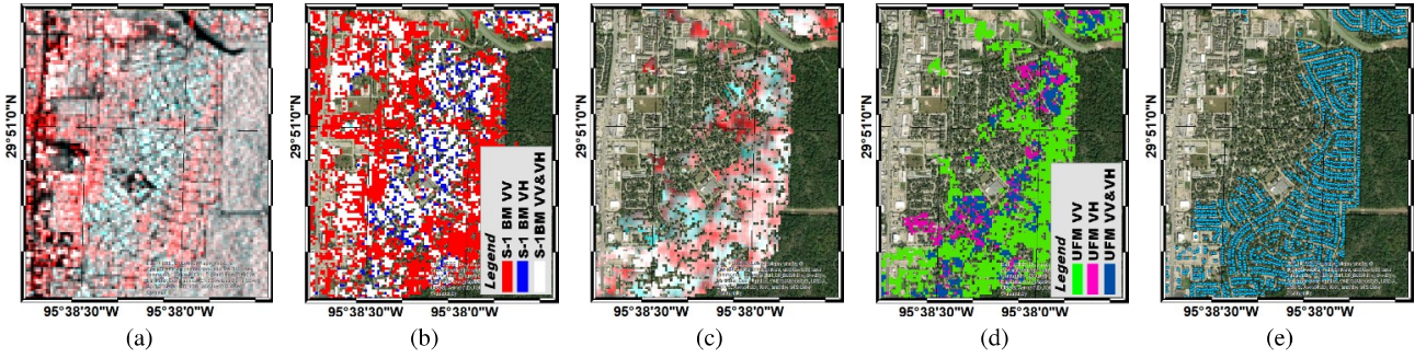
Fig. 4. VV and VH roles in (a) intensity temporal means ( R = VV , G = B = VH ), (b) S-1 BM. (c) Coherence drop-off ( R = \rho_{pre}^{VV} - \rho_{co}^{VV} , G = B = \rho_{pre}^{VH} - \rho_{co}^{VH} ). (d) VV-VH comparative UFM. (e) DG VHR imagery and flooded buildings crowd sourcing points.
