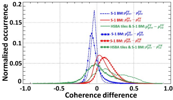
Fig. 1. Distributions of the InSAR coherence difference.
