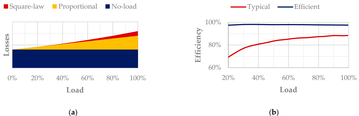
Figure 11. (a) Total losses in UPS, elaborated from [61]; (b) curve of efficiency of UPS, elaborated from [61,63].
