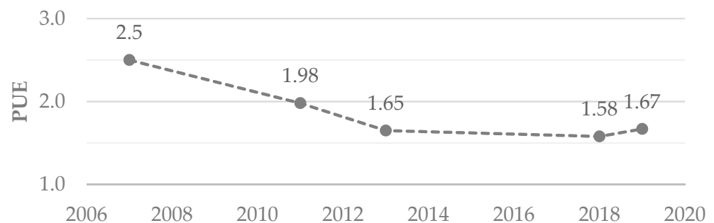
Figure 14. Evolution of industry-average PUE, elaborated from [140].
