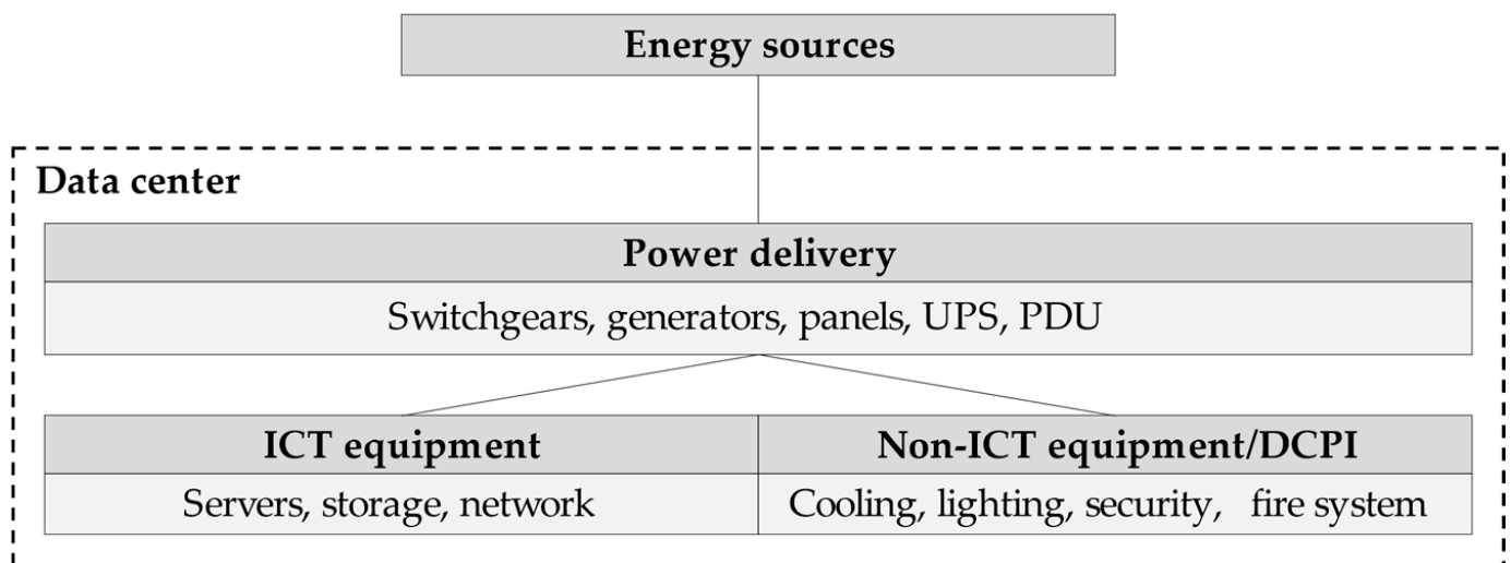
Figure 2. Energy use in a data center, elaborated from [41].
