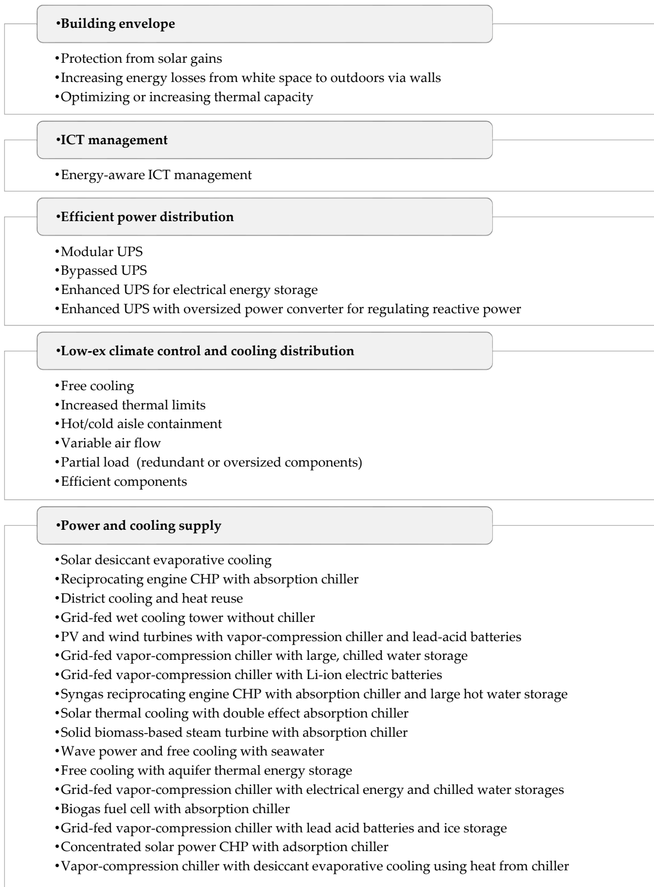
Figure 15. Advanced technical concepts to reduce electric and cooling load, elaborated from [148].
