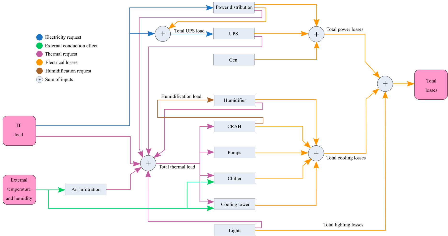
Figure 10. Diagram of energy losses in a data center, elaborated from [42].
