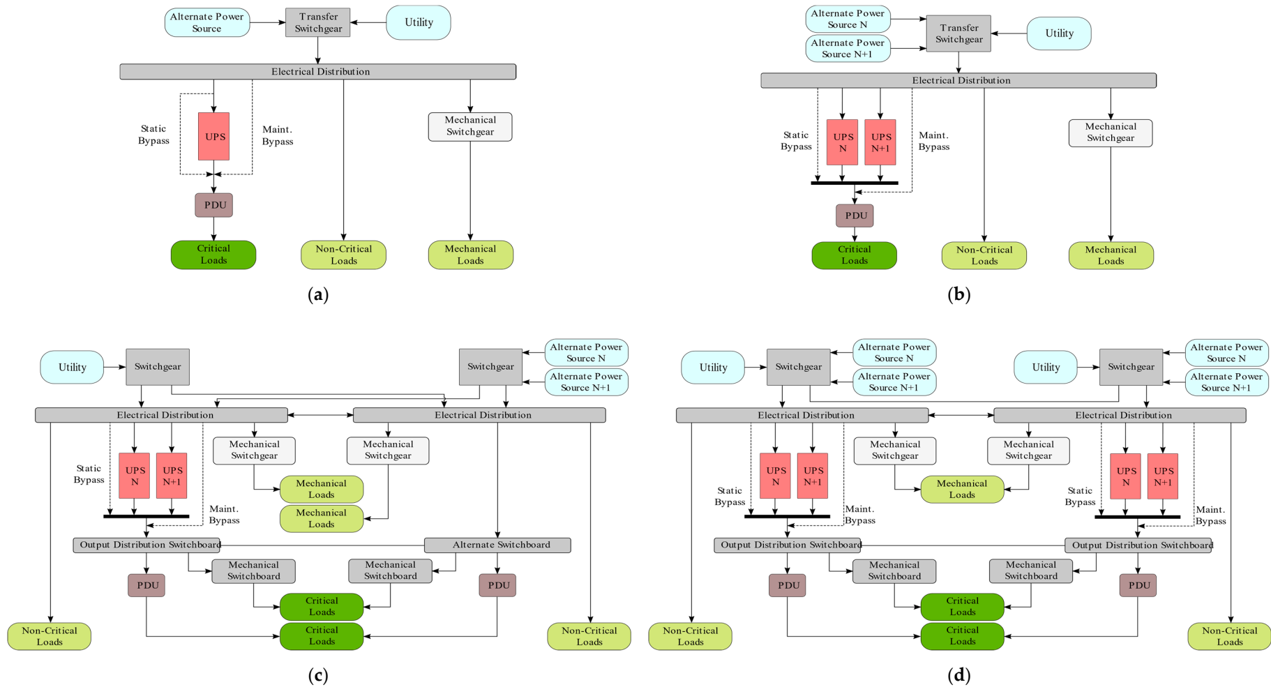
Figure 9. Diagrams of power distribution systems based on Tier: (a) Tier I; (b) Tier II; (c) Tier III; (d) Tier IV; elaborated from [59].
