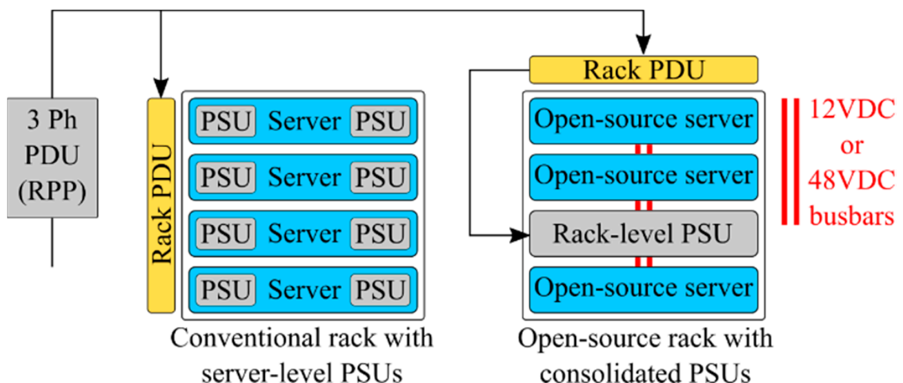
Figure 8. Conventional server rack and rack with PSU disaggregated from servers, elaborated from [52].
