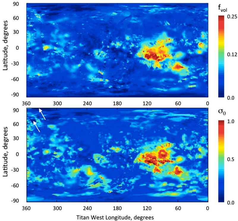
Fig. 1 Predicted and observed maps of scattering from Titan's surface. The upper panel is a map of the volume scattering parameter f_{\text{vol}} for a simple surface model composed of a smooth dielectric interface separating free space from an inhomogeneous and isotropically scattering subsurface. f_{\text{vol}} is the probability that a photon entering the surface (as determined by the effective dielectric constant) scatters and escapes from the subsurface before it is absorbed. The map of f_{\text{vol}} reconciles the maps of effective dielectric constant and emissivity and predicts the overall magnitude of the scattering. The lower panel is a global mosaic of Titan's normalized radar cross-section from all real aperture data through T71 (Wye 2011), showing the actually observed scattering. The white arrows in the upper left-hand corner indicate two small regions that were not mapped
