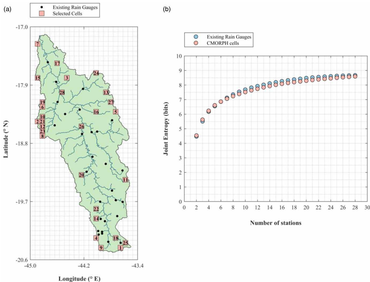
Figure 3 | (a) Map of the first 28 ranked CMORPH cells (case S); (b) joint entropy ( JH ) variation with increasing number of locations selected, both for existing rain gauges (light blue) and CMORPH cells (pink). Please refer to the online version of this paper to see this figure in colour: http://dx.doi.org/10.2166/nh.2021.113 .
