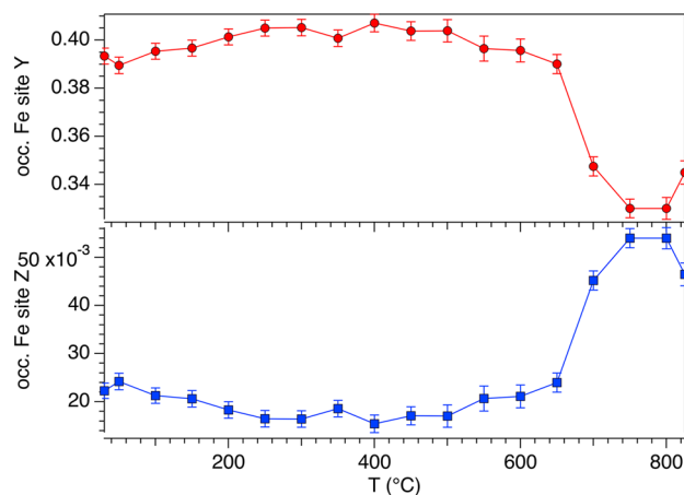
Fig. 7 Evolution with T of the Fe (+Mn) occupancy at the Y and Z sites for the fluor-elbaite studied
