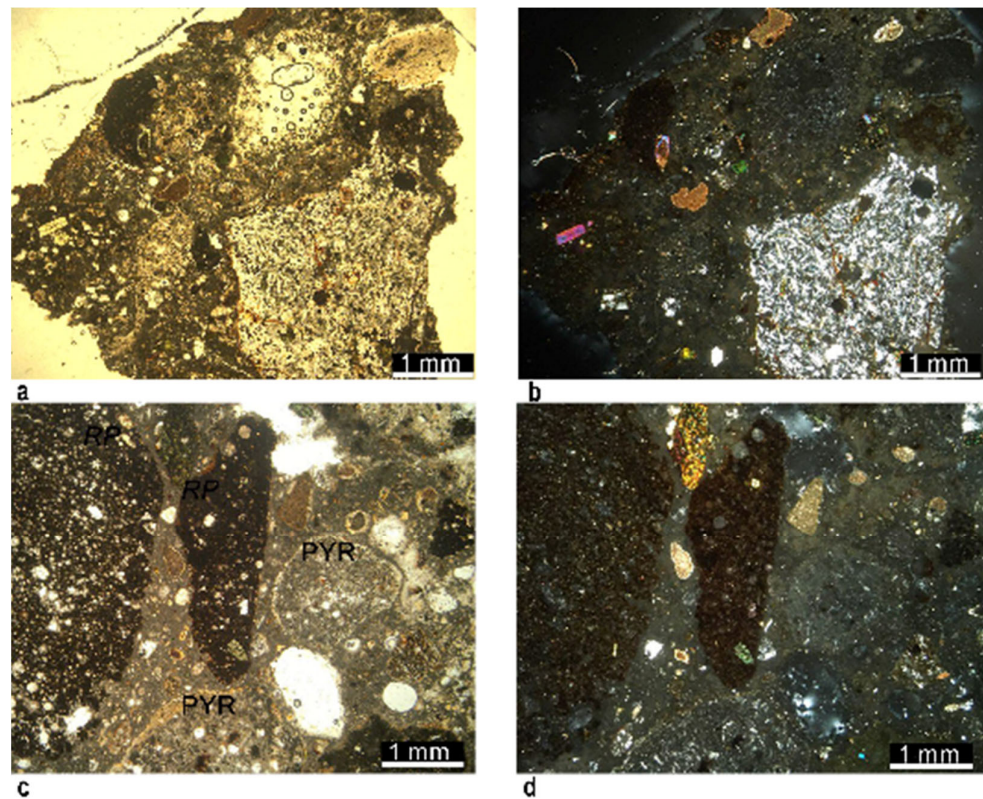
Figure 2. Optical Microscopy micrographs of two Trajan mortars in thin section (parallel (left) and crossed polarized light (right): (a,b) sample TRA 5; (c,d) sample TRA 25; PYR = pyroclastic rock fragment surrounded by illuvial clay; RP = red pozzolan.
