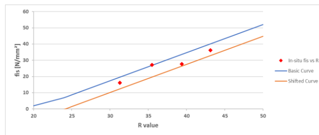
Fig. 6. The curve correlating rebound readings to the in-situ compressive strength;
