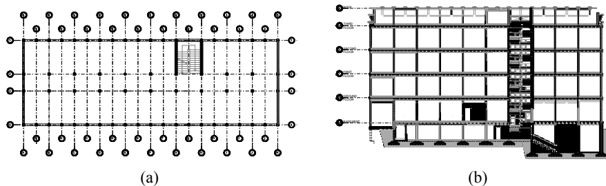
Fig. 1. (a) Existing base plan ( Source: ARTING drawings ); (b) Section drawing ( Source: EPTISA drawings );
