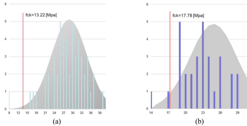
Fig. 7. Normal distribution of the compressive strengths for (a) columns and (b) beams;
