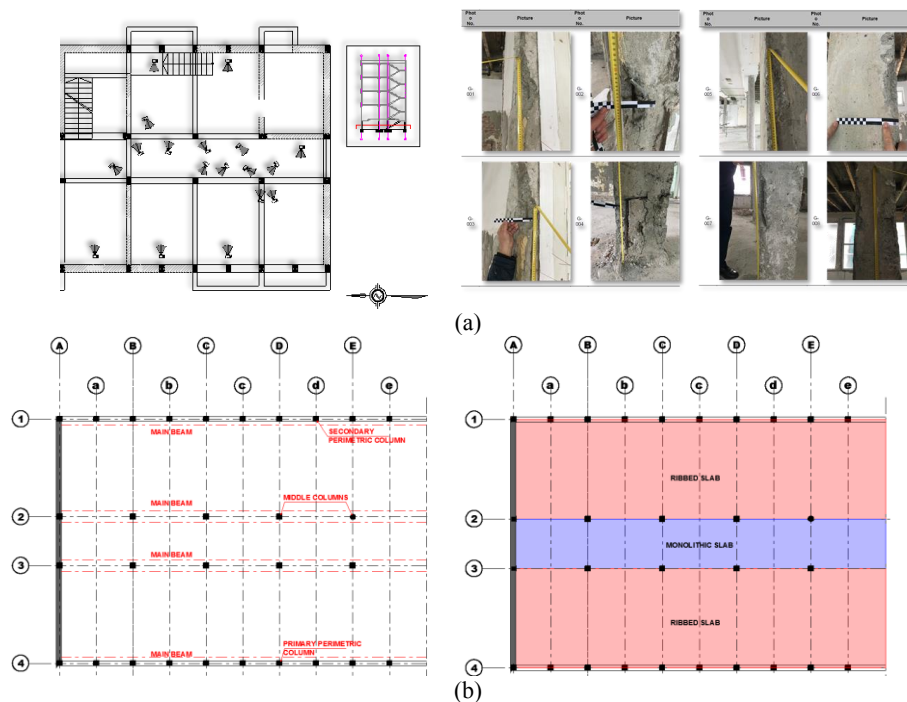
Fig. 3. (a) Example of the photographic survey and mapping on the drawings; (b) Structural system of the existing building;
