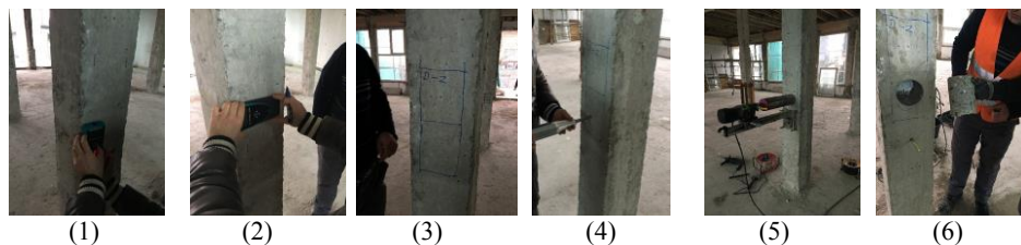
Fig. 4. Core sampling procedure;
