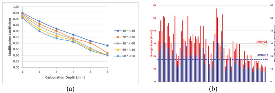
Fig. 5. (a) Carbonation reduction factor according to strength detected; (b) Strength readings from rebound hammer and after reduction;
