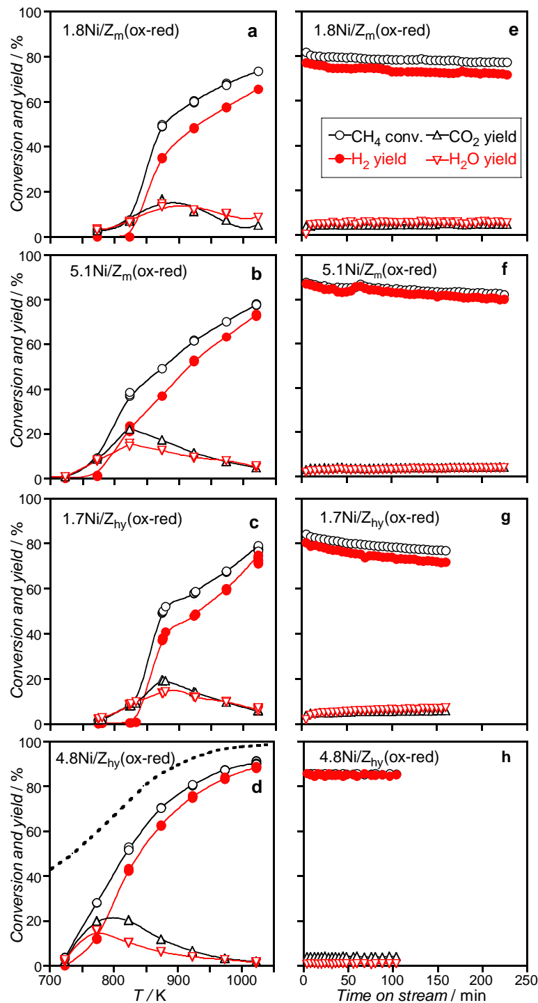
Figure 11. Catalytic activity (CH 4 conversion and H 2 , CO 2 and H 2 O yields) of Ni/ZrO 2 catalysts after ox-red activation treatment in experiments as a function of temperature (left side: (a–d)) or as a function of time on stream at 1023 K (right side: (e–h)). Reactant mixture: [CH 4 ] = 2%, [O 2 ] = 1%, N 2 as balance; total flow rate = 150 cm 3 (STP)·min -1 . Dotted line: CH 4 conversion for the same mixture calculated at thermodynamic equilibrium (data from Ref. [11]).
