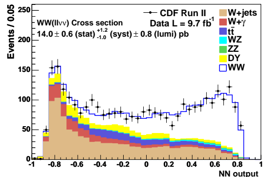
FIG. 1: Estimated and observed combined distributions of outputs for neutral networks (NNs) trained to identify WW events, with a higher NN output value indicating a more signal-like event. Event yields are normalized to the values returned by fitting signal and background distributions to the data.
