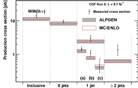
FIG. 2: Measurement and predictions of \sigma(p\bar{p} \rightarrow W^+W^- + n\text{jets}) . Values are given inclusively and differentially as functions of jet multiplicity and jet-transverse energy. Transverse energy ranges are (a) 15 < E_T < 25 GeV, (b) 25 < E_T < 45 GeV, and (c) E_T > 45 GeV.
