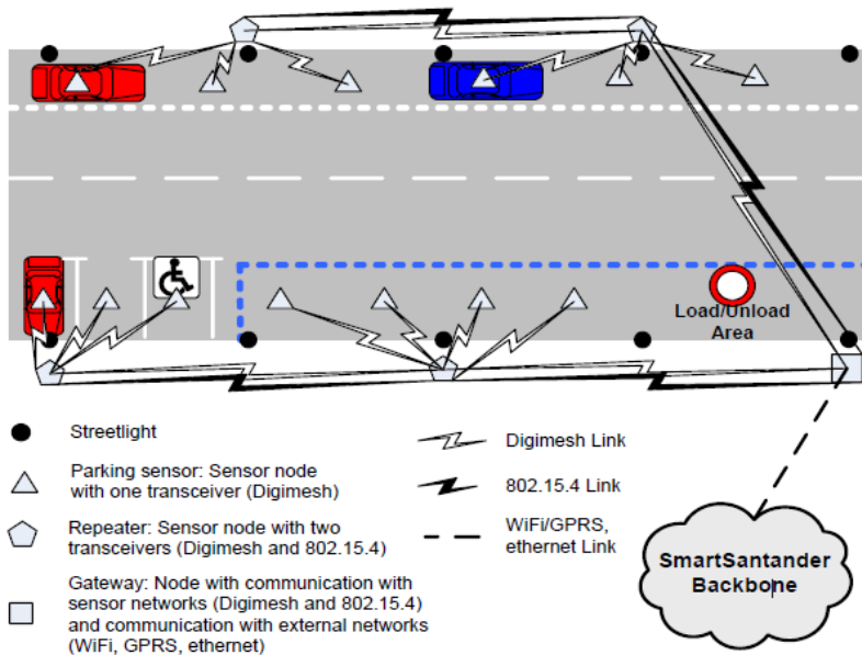
Figure 3: Architecture of Smart Parking infrastructure in the Santander deployment
