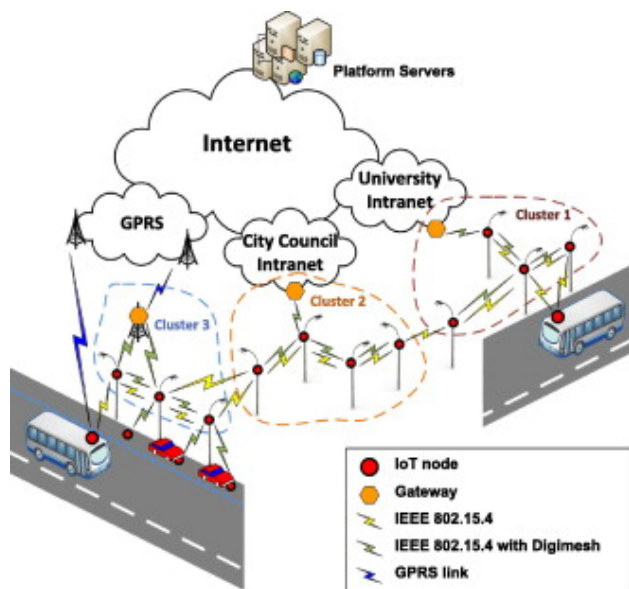
Figure 4: Physical Network layout of Smart Parking infrastructure in the Santander deployment
