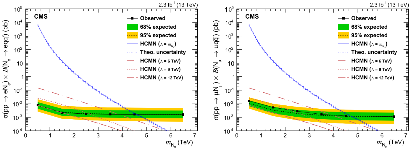
Fig. 5. The observed 95% CL upper limits (solid black lines) on \sigma(pp \rightarrow \ell N_\ell) \mathcal{B}(N_\ell \rightarrow \ell q\bar{q}') , obtained in the analysis of the e\bar{e}q (left) and the \mu\bar{\mu}q (right) final states, as a function of the mass of the heavy composite Majorana neutrino, N_\ell . The corresponding expected limits are shown by the dotted lines, and the bands represent the expected variation of the limit to one and two standard deviation(s). The solid blue curve indicates the theoretical prediction of \sigma(pp \rightarrow \ell N_\ell) \mathcal{B}(N_\ell \rightarrow \ell q\bar{q}') for \Lambda = m_{N_\ell} . The uncertainty in the theoretical prediction is derived by taking into account the factorization and normalization scales. The light red textured curves give the theoretical predictions for three \Lambda values ranging from 6 to 12 TeV in steps of 3 TeV. (For interpretation of the references to colour in this figure legend, the reader is referred to the web version of this article.)
