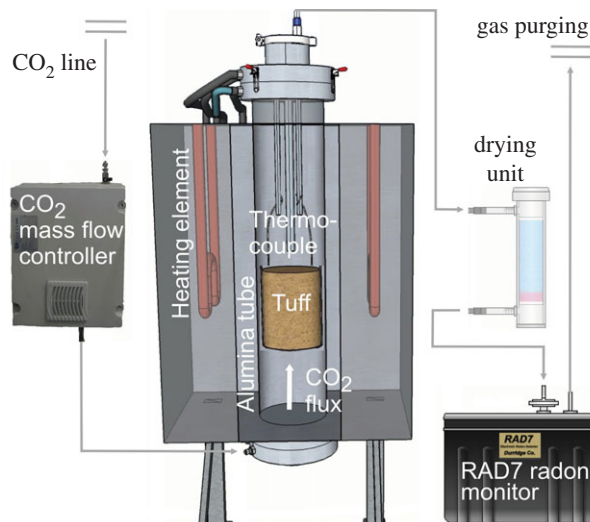
Figure 1. Sketch of the experimental system consisting of a vertical furnace equipped with a gas-impermeable alumina tube in which a cylindrical tuff sample is suspended. Four heating elements and one factory-calibrated thermocouple control the temperature with \pm 3^\circ\text{C} uncertainty. A digitally controlled \text{CO}_2 mass flow meter operates from 0.01 to 3\text{ l min}^{-1} with \pm 1.5\% accuracy. An iron steel tube is inserted into the lower flange and fluxes a pure 100\% \text{CO}_2 gas in the vertical furnace. A Teflon tube is inserted into the upper flange and connects the vertical tube with both a gas-drying unit ( \text{CaSO}_4 desiccant with 3\% \text{CoCl}_2 , as an indicator) and the RAD7 (DurrIDGE Company Inc.) counting system.
