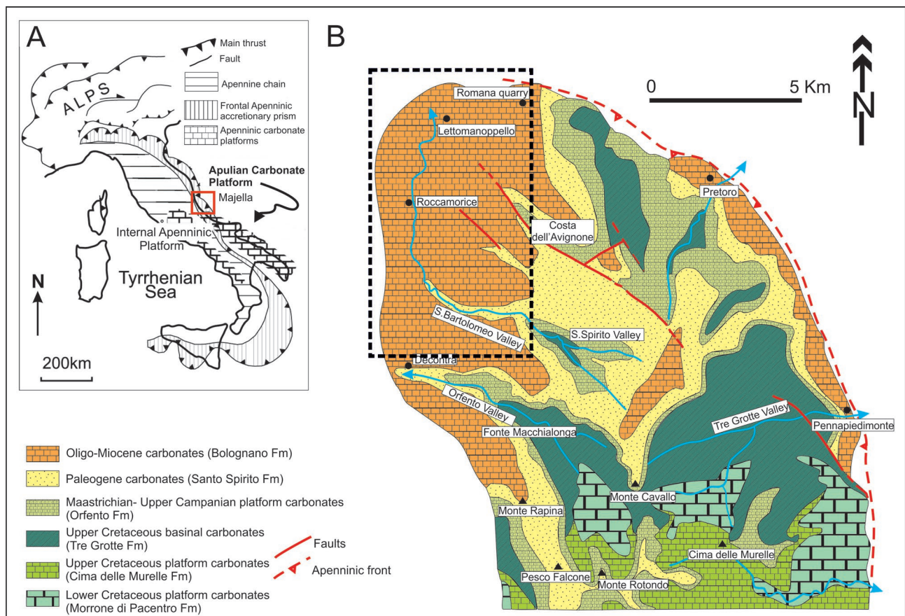
Fig. 1. A — A simplified geological map of Italy (modified from Pomar et al. 2004; B — Schematic geological map of Majella Mountain with the main carbonate deposits from Upper Jurassic to upper Miocene (modified from Vecsei & Sanders 1999); the dashed black rectangle indicates the investigated area where the geological map has been produced.
