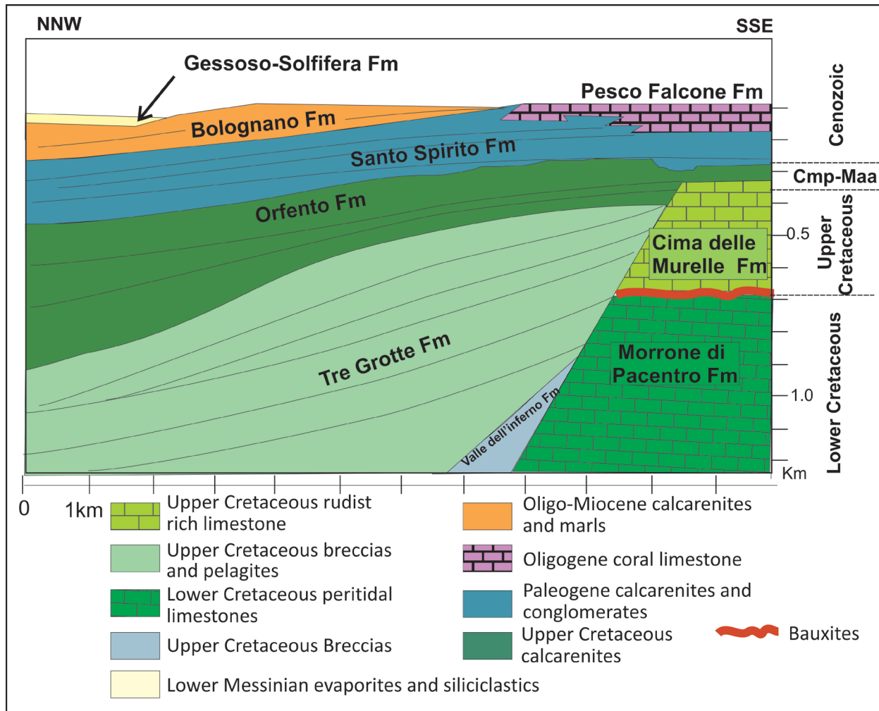
Fig. 2. Schematic stratigraphic architecture of the Majella carbonate platform (modified after Vecsei et al. 1998).
