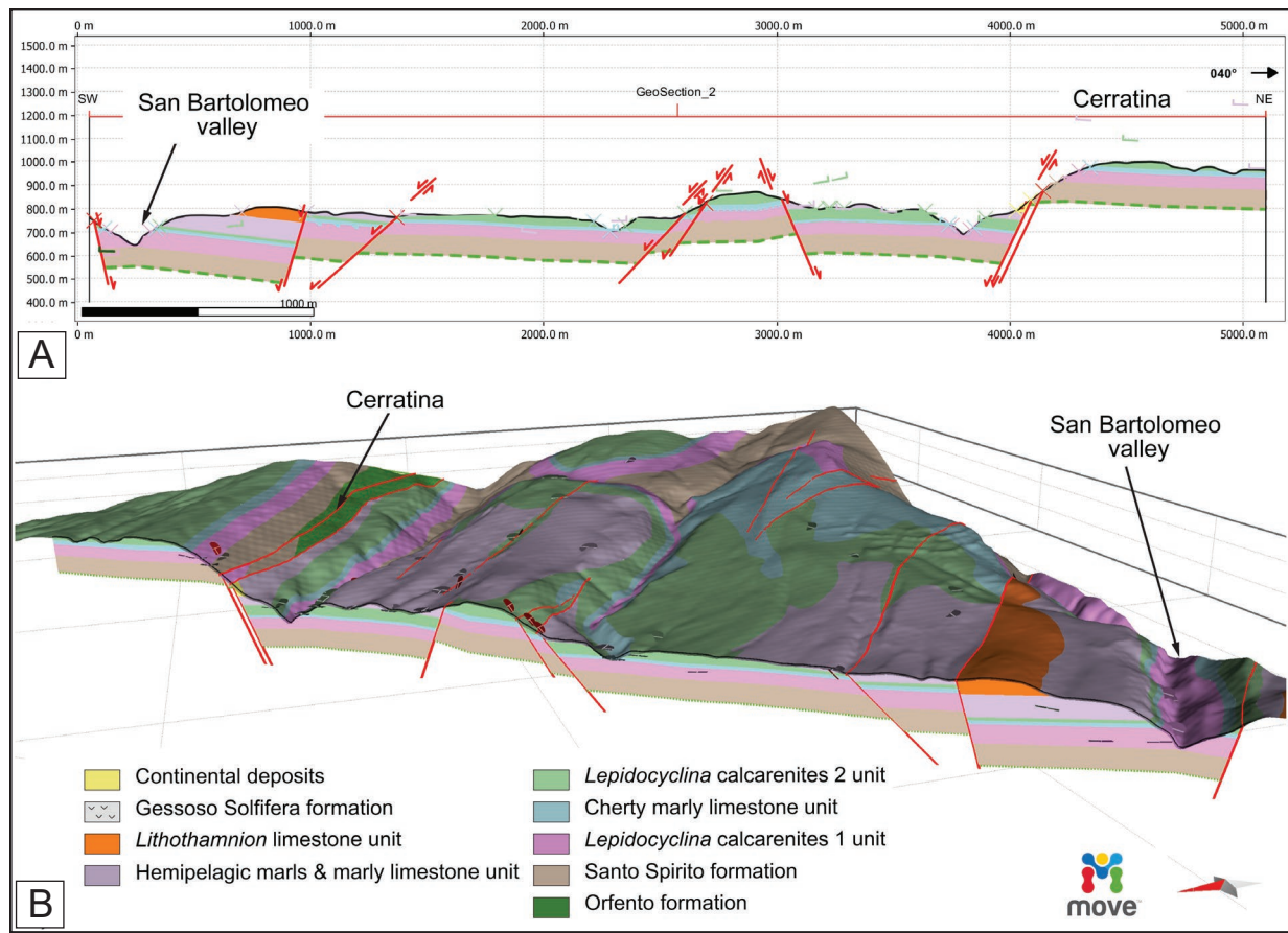
Fig. 7. A — Example of a geological section made in the Move software (© Midland valley). The topography profile has been extrapolated from the DEM and all the intersections of geological boundaries and faults lines along the trace of the geological section (see Fig. 6) have been automatically collected (see crosses along the topographic profile). The dip data of geological layers and of faults have been projected along the trace in respect of their geometric relationship (i.e. along dip or along strike projection). B — 3D visualization of the geological section of Fig. 7a. Several geological sections have been made and analysed in 3D environment to better constrain the geometry of the Bolognano units. Note the variation in the thickness of the Lepidocyclina calcarenites units. The Lepidocyclina calcarenites 2 unit becomes thicker toward NE and, in contrast, the thickness of the Lepidocyclina calcarenites 1 unit remains almost constant between Cerratina and San Bartolomeo valley (Fig. 6). Location of geological section is shown in Figure 6.
