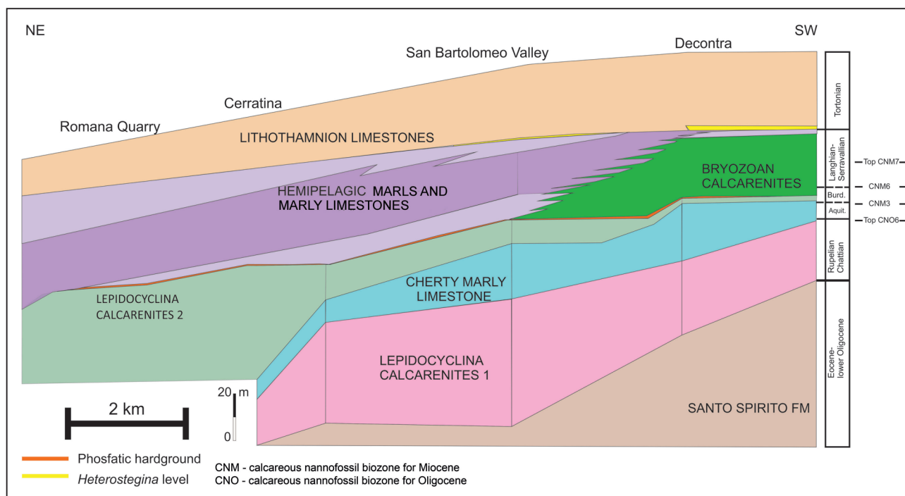
Fig. 3. Stratigraphic architecture of the Bolognano Formation showing the geometrical relationships of the five lithofacies associations and the biostratigraphic constraints based on the nannoplankton biostratigraphy of Raffi et al. 2016 (modified after Brandano et al. 2016a).
