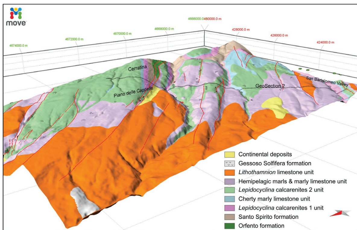
Fig. 6. 3D view of the vector-based geological map showing the stratigraphic units composing the Bolognano Fm. between Lettomannoppello and San Bartolomeo valley. The geological map created in QGis has been draped upon a 10 m-cell size grid DEM (no vertical exaggeration; Tarquini et al. 2007). Vector-based dip data representing the attitude of geological layers, distinguished according their geological units, and of faults have been imported in the 3D environment. Several geological sections have been made using the tools of the Move software (version 2017.2; © Midland valley) and the 3D visualization helped to better defined the uncertainties in the geological mapping and to analyse the geometrical relationship of the Bolognano architecture. The black line named “GeoSection 2” shows the location of the trace of the geological section shown in Figure 7.
