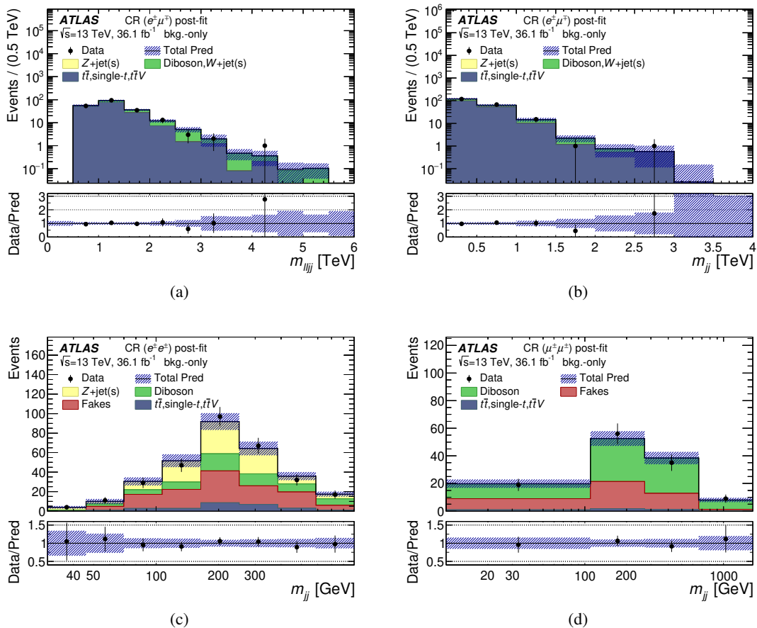
Figure 4: Distributions for data and background predictions for discriminant variables in various control regions and channels after the background-only fit: (a) m_{\ell\ell jj} in CR( e^\pm \mu^\mp ), (b) m_{jj} in CR( e^\pm \mu^\mp ), (c) m_{jj} in CR( e^\pm e^\pm ), and (d) m_{jj} in CR( \mu^\pm \mu^\pm ). The hatched bands include all post-fit systematic uncertainties. The correlation between sources of systematic uncertainties are taken into account. The last bin in each histogram contains the overflow.
