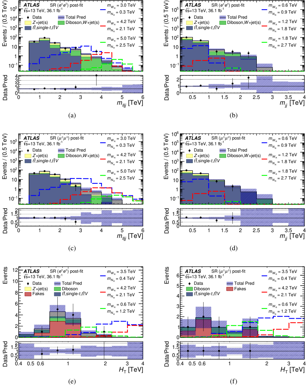
Figure 6: Distributions for data and background predictions after the CR+SR fit for discriminant variables in various signal regions and channels: (a) m_{ljj} in SR( e^\pm e^\mp ), (b) m_{jj} in SR( e^\pm e^\mp ), (c) m_{ljj} in SR( \mu^\pm \mu^\mp ), (d) m_{jj} in SR( \mu^\pm \mu^\mp ), (e) H_T in SR( e^\pm e^\pm ), and (f) H_T in SR( \mu^\pm \mu^\pm ). The hatched bands include all post-fit systematic uncertainties. The correlation between sources of systematic uncertainties are taken into account. A few simulated signal distributions, normalised to the predicted cross-section, are overlaid on top of the background prediction in the plots. The last bin in each histogram contains the overflow.
