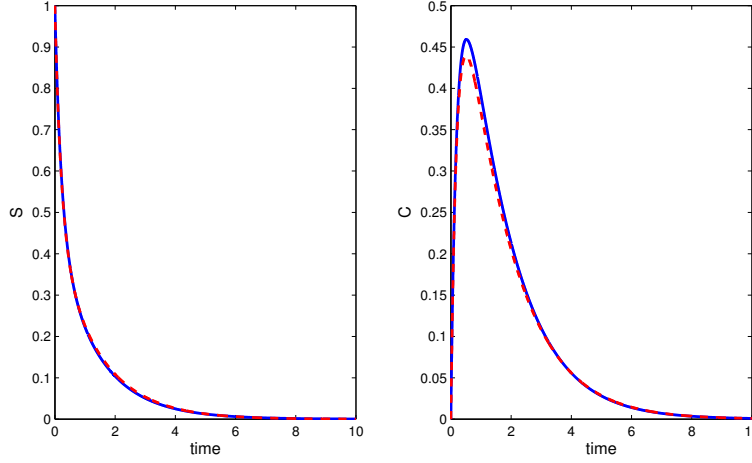
Fig. 2 Dynamics of S (left panel) and of C (right panel): full system (solid), uniform approximation (dashed). Initial concentrations: E_T = 3 , S_T = 1 . Kinetic parameters: a = 1 , d = 1 , k = 1 . Taken from [36]
