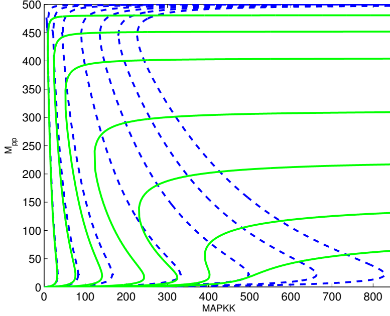
Fig. 3 Stationary branches of the double phosphorylated MAPK ( M_{pp} ) in the full system (89) (solid) and in its sQSSA approximation (94) (dashed), obtained varying the initial concentration of the kinase MAPKK, for different values of the initial concentration of the phosphatase: MKP3=20,50,100,200,300,400,500 (left-right); kinetic parameters as in Table 1 and M_T = 500 . Taken from [37,38].
