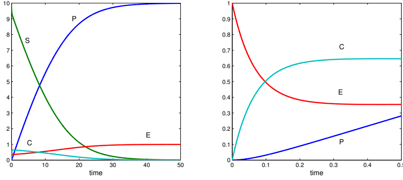
Fig. 1 Figure 1a: Time behavior of the reactants: S (green), C (azure), E (red), P (blue). Figure 1b: zoom of the transient phase, where the initial convex behavior of P is clearly shown, together with the fast growth of C . Initial concentrations: E(0) = E_T = 1 , S(0) = S_T = 10 , P(0) = 0 , C(0) = 0 . Kinetic parameters: a = k = 1 , d = 4 .
