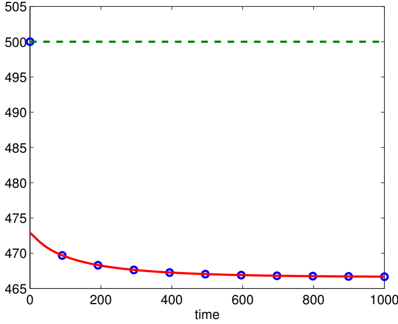
Fig. 4 Dynamics of M + M_p + M_{pp} in the reaction (86): full system (circles), tQSSA approximation (solid), sQSSA approximation (dotted). Here MAPKK=30 , MKP3=20 , kinetic parameters as in Table 1 and M_T = 500 . Differently from the full system and the tQSSA, the sQSSA predicts at any time a constant value M_T for M + M_p + M_{pp} that would imply C_1 + C_2 + C_3 + C_4 = 0 . Taken from [37,38].
