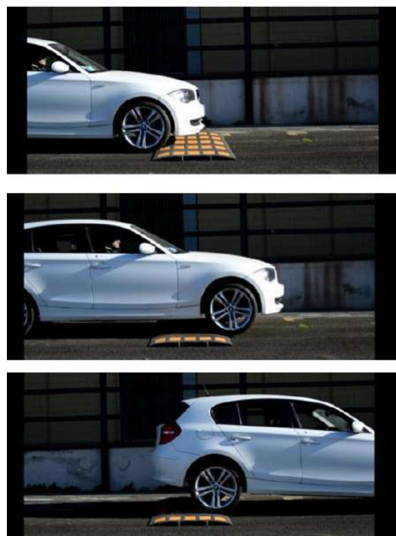
Figure 21. Experimental test of bump speed crossing.
