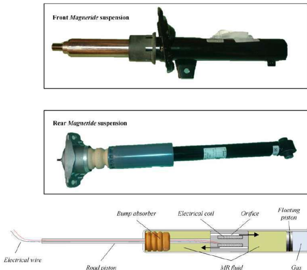
Figure 13. The magneto-rheological damper installed on BMW ( MagneRide of BWI Group).
