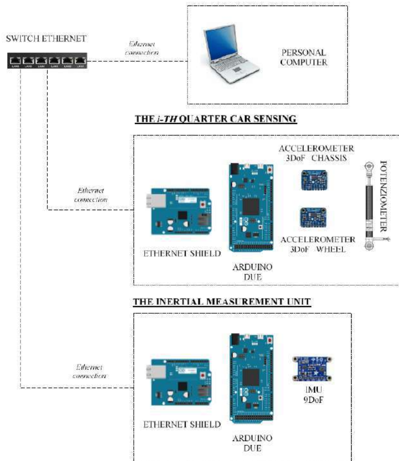
Figure 5. Sensors architecture and communication scheme.
