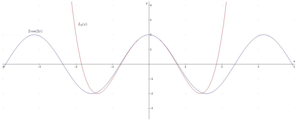
FIGURE 1. comparison between L_2(x) and 2 \cos(2x) .
