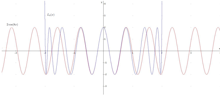
FIGURE 3. comparison between L_4(x) and 2 \cos(8x) .
