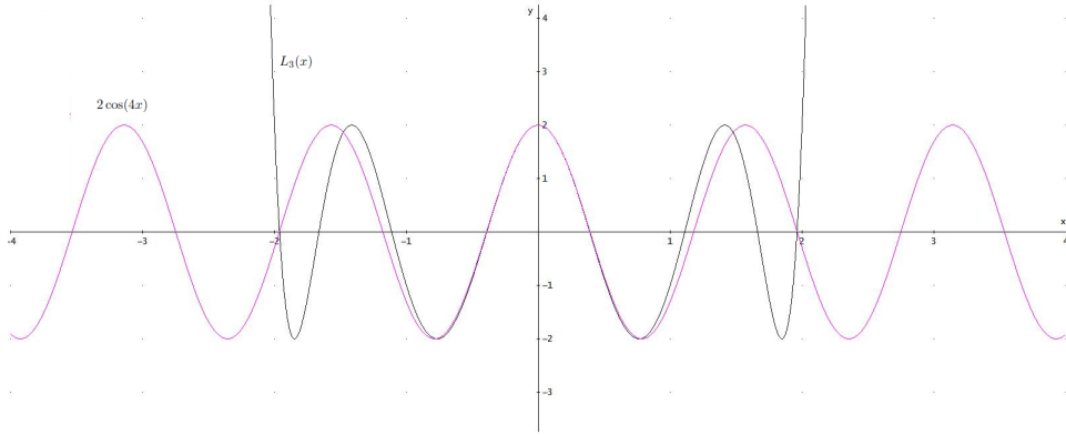
FIGURE 2. comparison between L_3(x) and 2 \cos(4x) .
