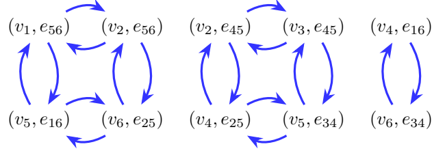
Fig. 3. A visualization of connected components in \mathcal{G}^\dagger . Each isometric circuit \mathcal{C} in \mathcal{G} corresponds to a double-linked directed cycle in \mathcal{G}^\dagger with |\mathcal{C}| vertices. This example is created using the graph in Fig. 1, while the cycle representations that do not create links by Lemma 2 are ignored.
