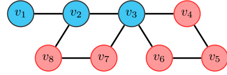
(a) Original unweighted graph.
