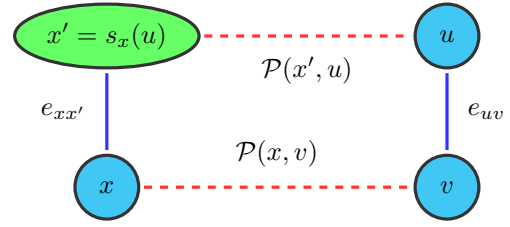
Fig. 2. An illustration of Lemma 2. Let us consider the cycle represented by the vertex x and edge e_{uv} , i.e. \mathcal{C} = \mathcal{C}(x, e_{uv}) \triangleq \mathcal{P}(x, u) + \mathcal{P}(x, v) + e_{uv} . x' = s_x(u) is the first vertex on the path \mathcal{P}(x, u) , i.e., \mathcal{P}(x, u) = e_{xx'} + \mathcal{P}(x', u) . The key to the proof of Lemma 2 is based on the observation that: If \mathcal{C} is isometric, there are two possible cases for the shortest path between the vertex x' and v : (a) \mathcal{P}(x', v) = e_{xx'} + \mathcal{P}(x, v) , (b) \mathcal{P}(x', v) = \mathcal{P}(x', u) + e_{uv} . Obviously case (a) implies x = s_{x'}(v) and \mathcal{C} = \mathcal{C}(x', e_{uv}) , while case (b) implies u = s_v(x') and \mathcal{C} = \mathcal{C}(v, e_{xx'}) .
