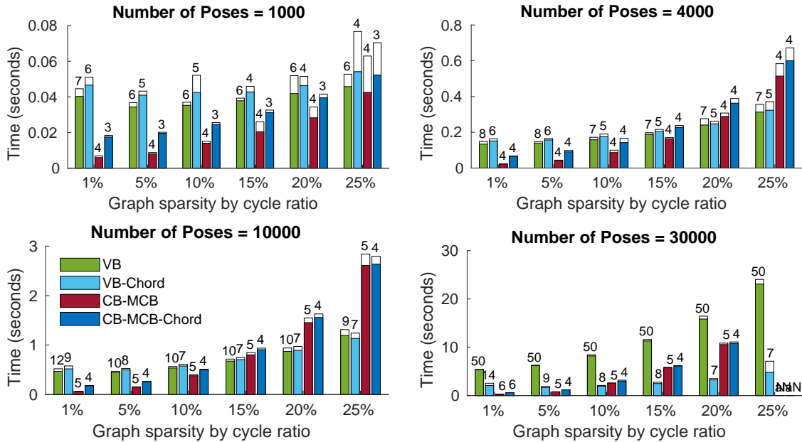
Fig. 7. The computational time of VB (VB-PGO initialized by odometry), VB-Chord (VB-PGO initialized by the Chordal initialization technique), CB-MCB (CB-PGO based on the MCB, initialized by the measurements of relative poses), and CB-MCB-Chord (CB-PGO based on the MCB, initialized by the Chordal initialization technique) on 100 run Monte-Carlo simulation. The mean is plotted with color, and the standard deviation is added to the bar-plot as the white margin. The number above each bar is the used iterations. The maximal iteration is set to 50.
