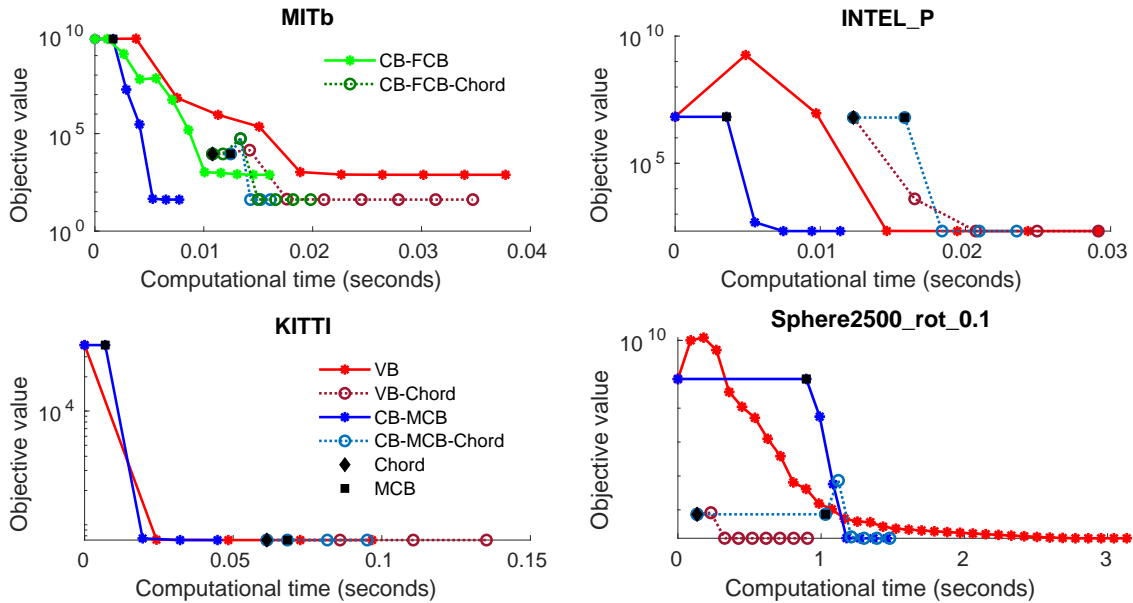
Fig. 6. The convergence of different methods on benchmark datasets. Note that for INTEL_P, the initial objective values with and without the chordal initialization are 6281560 and 6700310 respectively, which are close but not the same. Aside from the MCB, the memory usage of VB and CB are comparable. For example in INTEL_P, the graph storage takes 1.13MB, while the matrix to be factorized accounts for 8.11MB; These numbers in CB are 1.34MB and 8.04MB respectively. For MITb, there are 92 nonzero blocks in the Cholesky part of CB-MCB, whereas 2462 for VB. For INTEL_P, CB-MCB accounts for 2234 nonzero blocks, and VB 4194. The numbers for KITTI are 5015 and 13831 respectively. For dense graphs like Sphere2500, there are 12244 nonzero blocks in the Cholesky part of CB-MCB, while the number for VB is 12398.
